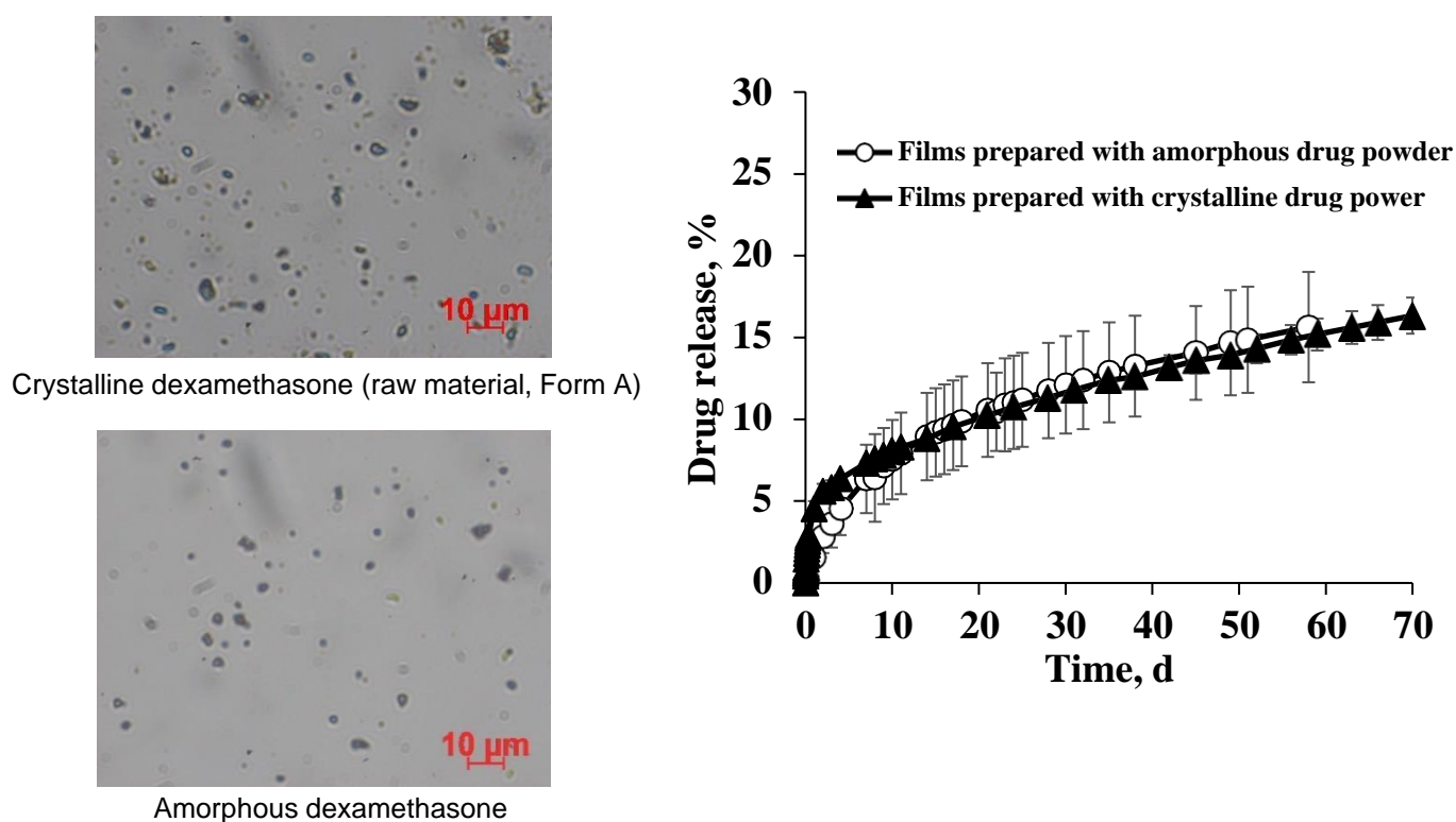
Figure 3.26. Dexamethasone release from silicone films prepared with crystalline (Form A) or amorphous drug powders upon exposure to artificial perilymph at 37 °C. The optical microscopy pictures on the left-hand side show the respective drug powders.
