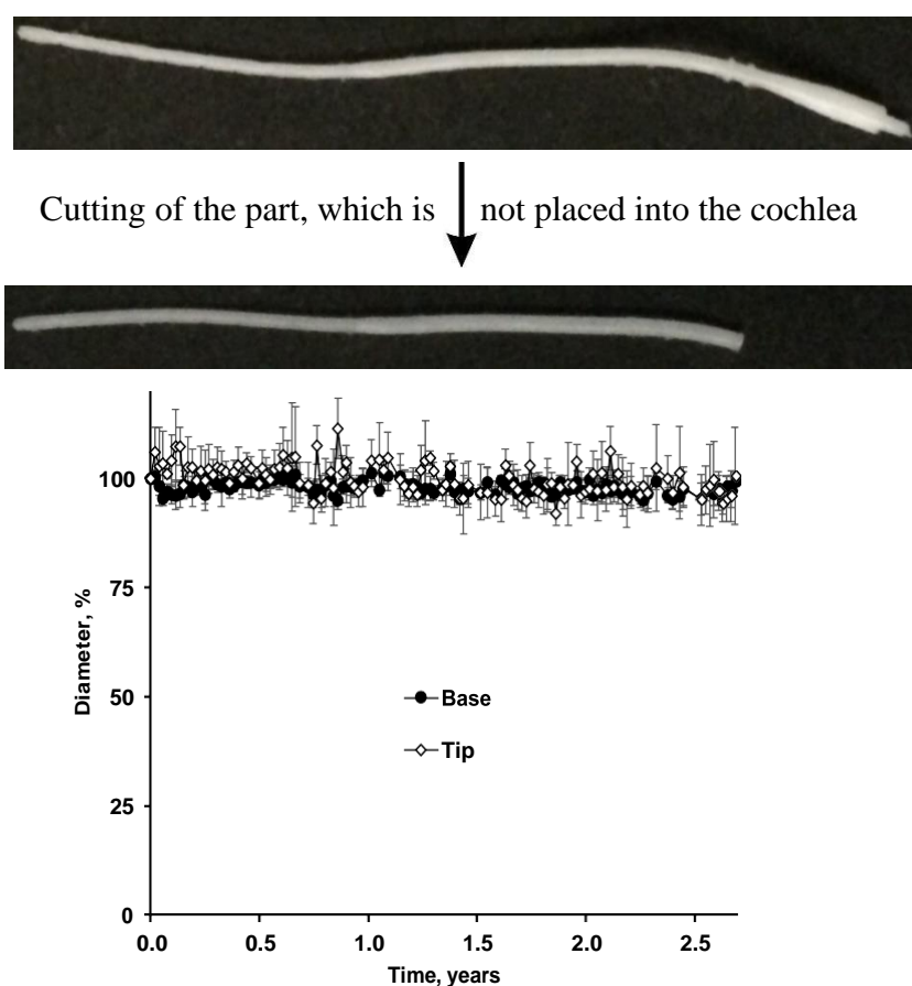
Figure 3.15. Top: Optical microscopy pictures of a cochlear implant for use in humans (without metal electrodes), loaded with 10 % dexamethasone (after manufacturing). For the drug release and swelling studies, the part of the implant which is not placed into the cochlea, was cut off. Bottom: Dynamic changes in the diameters of the “tips” and “bases” of the implants upon long term exposure to artificial perilymph at 37 °C (in vitro).
