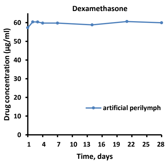
Figure 3.5. Stability of dexamethasone or dexamethasone phosphate in artificial perilymph, pure water or different types of aqueous salt solutions (as indicated) at 37 °C.
