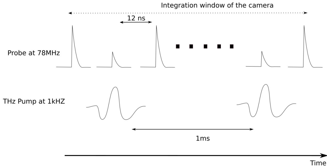
Figure 2.18: Figure showing the temporal overlap between the pump and the probe in a case where the repetition rate of the probe is greater than the one of the pump. The dot line represents the time integration of the camera.
