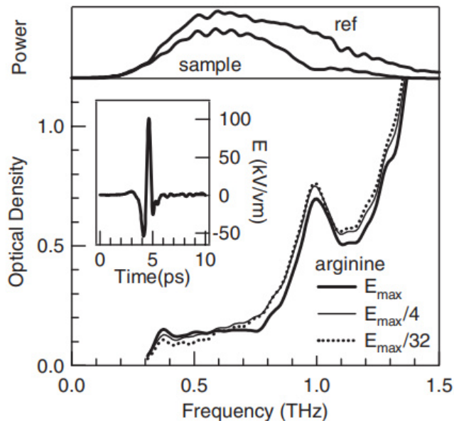
Figure 19: Optical density of an L-arginine pellet at different incident amplitudes of THz pulses. The inset shows the incident THz pulse. The upper part shows the power spectra of the THz pulse passing through the sample and without the sample. Figure adapted from [21]
