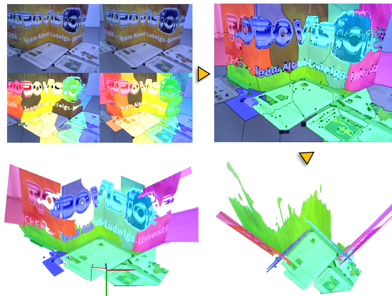
Figure 7.1 – From two RGB images of a monocular camera (left top), we propose a superpixel-driven technique to estimate simultaneously a relative camera pose and a 3D multi-planar map (bottom) without relying on a Manhattan assumption. In the right top, the different colors represent different 3D planes estimated from the images, using a novel approach we refer to as Winner-takes-all RANSAC.
