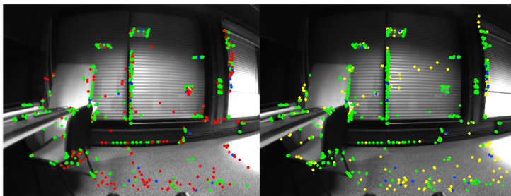
Figure 4.9 – An example of ORB feature on different illuminative condition, green dots mean correct tracked and matched features. Red and yellow represents untracked features detected at each image, respectively.
