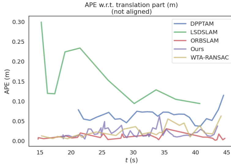
Figure 8.5 – Absolute Pose Error (APE) metric for the sequence fr_str_far of Dataset [113], it demonstrates proposed method outperforms all dense and semi-dense methods and reach good precision level to ORBSLAM which only provides sparse point cloud map.
