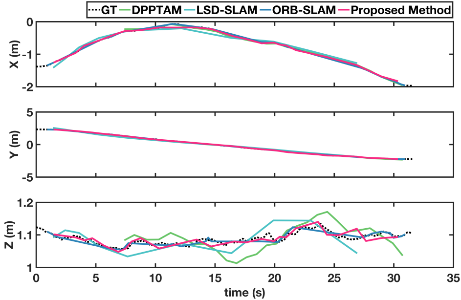
Figure 7.6 – Comparison of trajectories generated from different methods: Our proposed method shows a more stable and similar trajectory results w.r.t LSD-SLAM and DPPTAM, reaches the save level of state-of-the-art sparse SLAM method ORB-SLAM, thanks to the global planar representation and non-linear BA.
