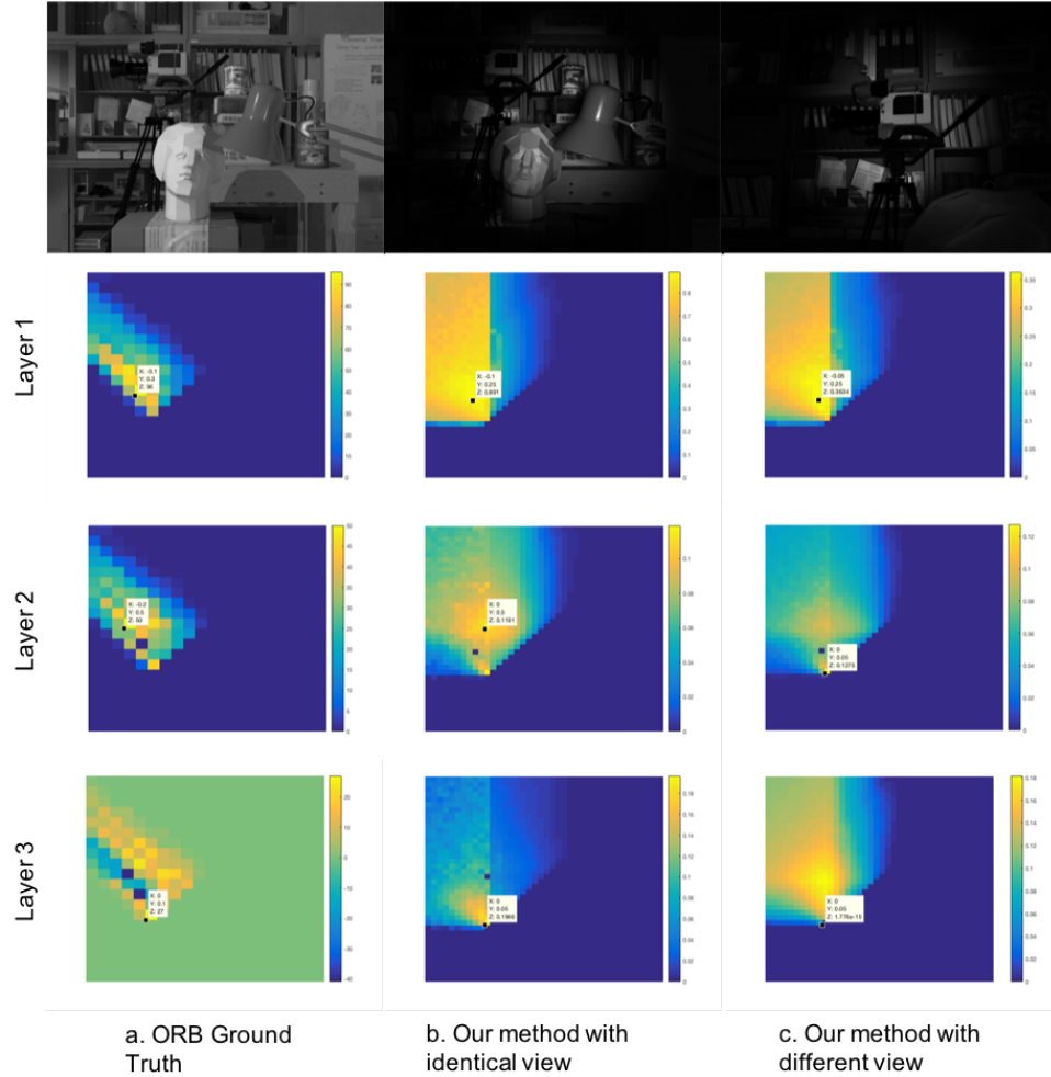
Figure 6.10 – In each layer, similar behaviors are shown with regard to optimums (see image a,b), compared with ORB detector. Ground truth for layers 2 and 3 are generated by a subtraction between the common keypoints detected from the previous optimal contrast band \mathbf{u}^* and the keypoints from all other contrast bands i.e. the ground truth of layer 2 is computed by removing all keypoints common with keypoints detected in previous optimum \mathbf{u}^* = (0, 0.15)^\top in layer 1. Empirical results also show that even with relatively different reference images (c), the landscapes are similar.
