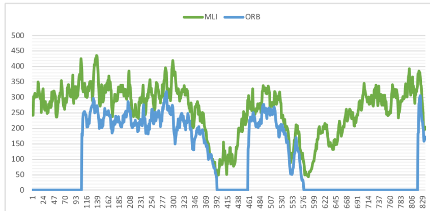
Figure 6.12 – The number of trusty inlier keypoints after graph optimization of ORB-SLAM which is a critical indicator displaying the tracking quality. MLI (green) generates significantly better results than standard ORB (blue) under the dynamic light changing environment.
