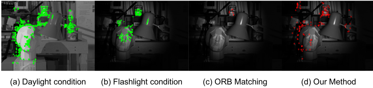
Figure 6.1 – ORB keypoint extractor and descriptor on different lighting conditions (images a and b). Only a few keypoints are matched between (a) and (b) using ORB ( i.e. same position, same descriptor), compared to our MLI method (image d).
