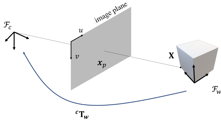
Figure 3.2 – Projecting an object from world frame to image plane represented in camera frame
