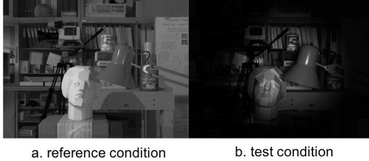
Figure 6.7 – Images I^* and I from NewTsukuba data set [84]: a synthetic data set with identical camera trajectories and variant illumination conditions
