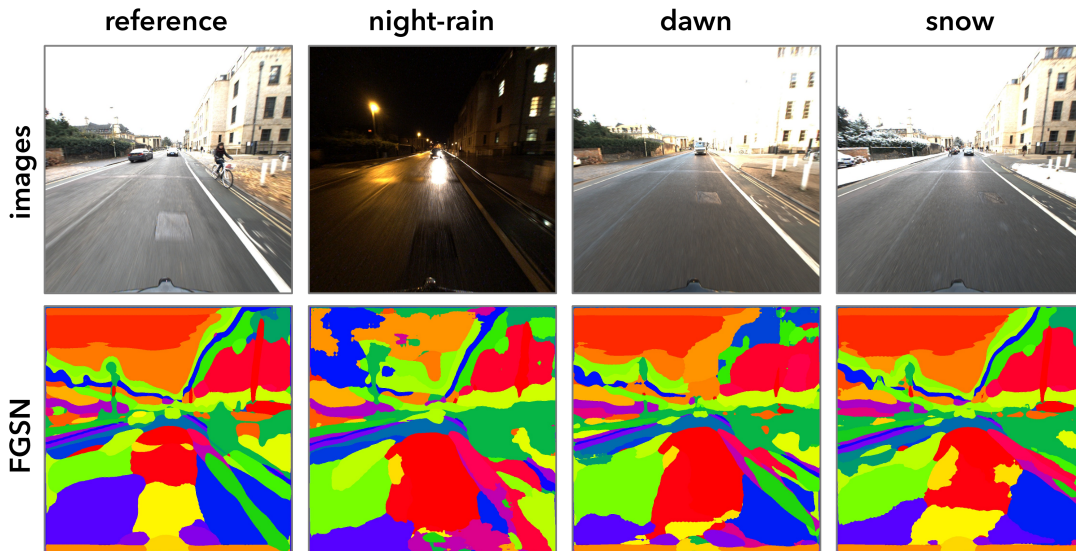
Figure 9.7 – The retrieval results from reference to various environmental conditions, our method can retrieve seen locations despite appearance disparities thanks to the spatial similarity in terms of semantic distribution on FGSN images.
