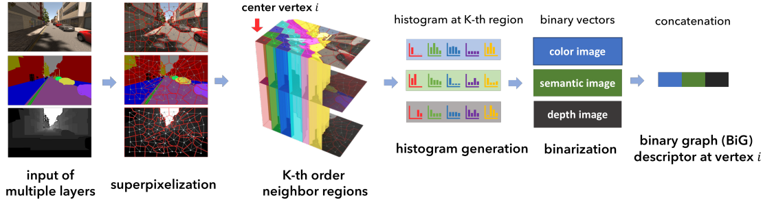
Figure 9.2 – The proposed pipeline to generate a BiG descriptor for a given superpixel (center vertex i ). Multiple layers of heterogeneous image are structured in a graph representation spanning over neighboring regions of the superpixel, and embedding in a BiG descriptor through graph embedding and binarization of multiple layered histograms.
