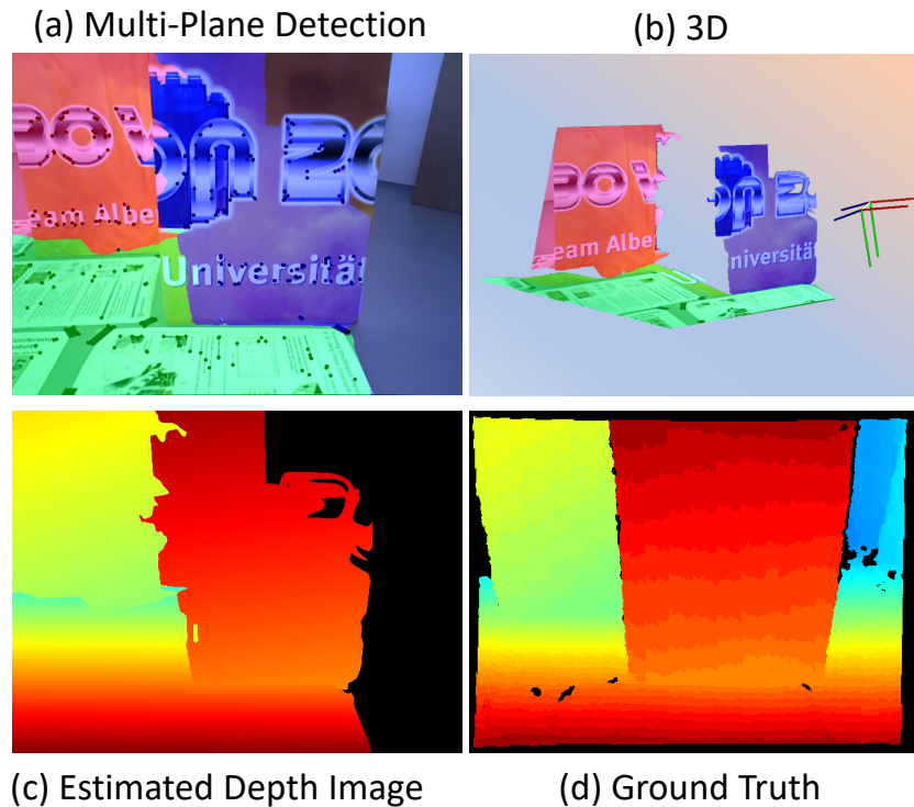
Figure 7.4 – Comparison of estimated results from image pair against the depth map from ground truth on the dataset TUM [113]. With a small number of parameters (3 planes), our proposed method is able to generate a very dense map.
