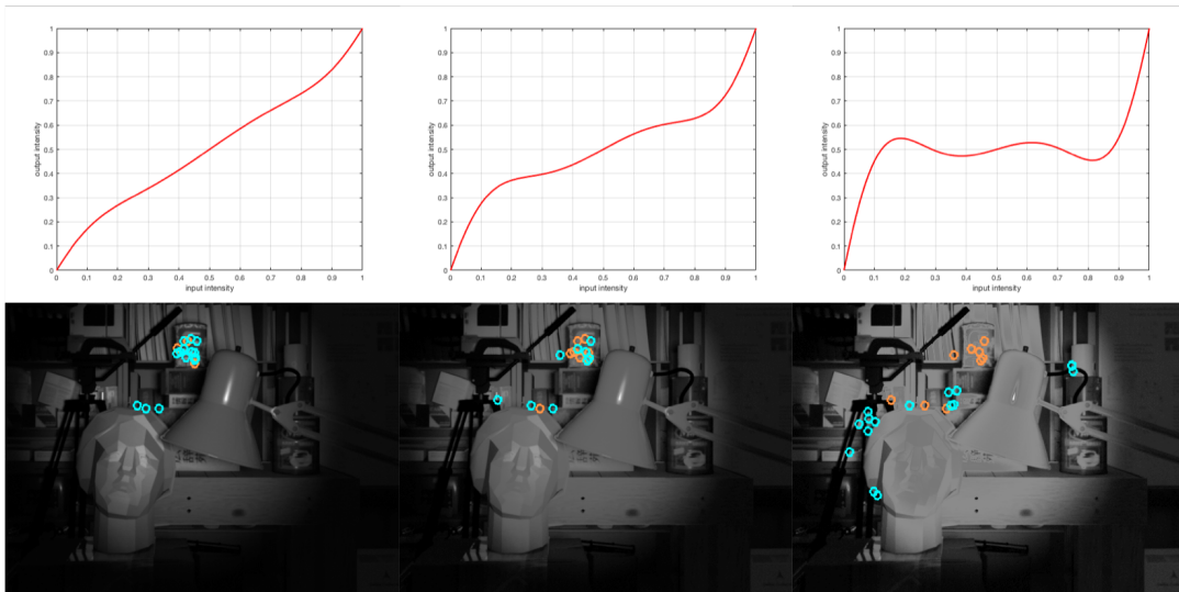
Figure 6.2 – Matching keypoints with ORB detector between a reference image (see Fig. 6.1 a) and different S-Curve tone mapped versions of an image in a different lighting condition. Each tone-mapping provides newly matched keypoints (blue) while losing others (orange).
