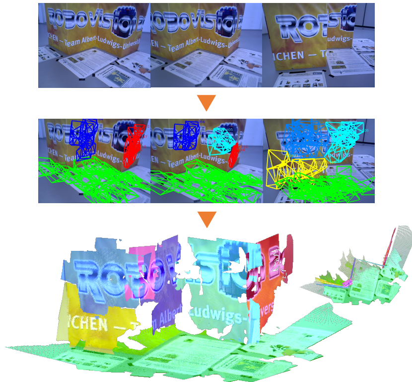
Figure 8.1 – We propose a method which tracks and clusters template-based trackers, estimates camera pose and maps three dimensional multi-planar environment on RGB image sequence acquired by monocular camera. Different colors represent different found three dimensional planes.
