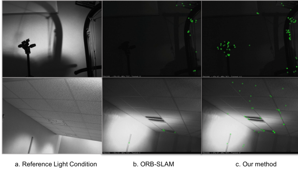
Figure 6.5 – Keypoint tracking results in different lighting conditions. Only a few keypoints are matched between reference condition (image a) and standard ORB-SLAM (image b), compared to our novel MLI method (image c).
