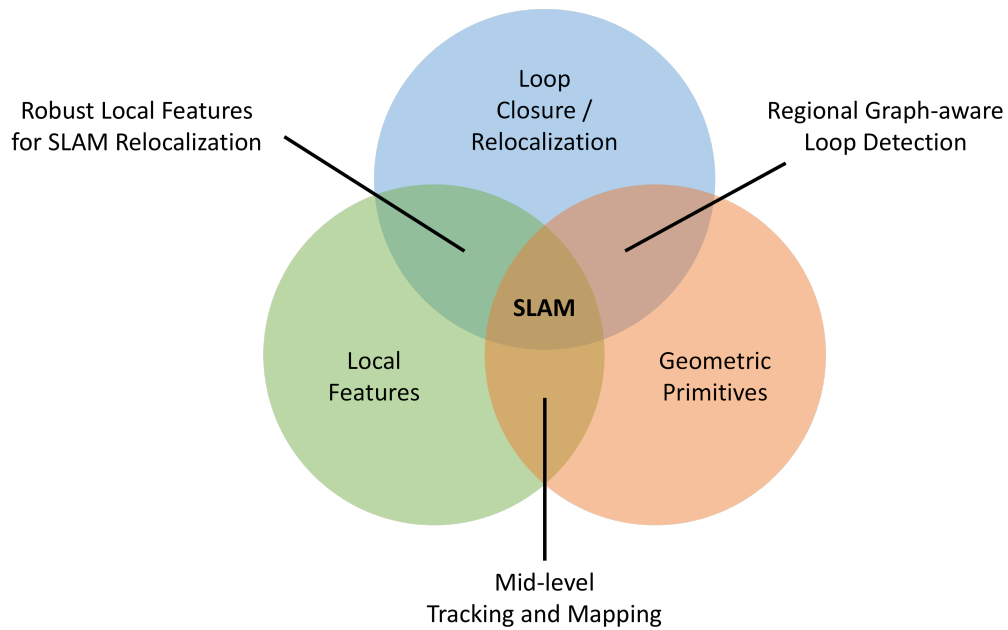
Figure 5.1 – We decompose SLAM technique into three aspects and present the intersected regions as our contributions: i) robust local feature for SLAM relocalization purpose; ii) mid-level geometric primitive for tracking and mapping more semantically; iii) regional graph-based binary descriptors for loop detection tasks.
