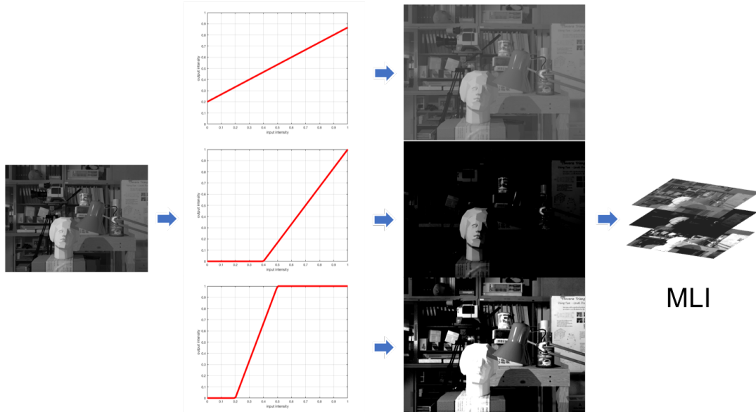
Figure 6.3 – Using SAT function with different contrast bands to generate a multi-layered image representation (MLI).
