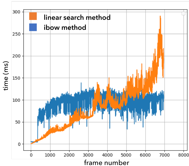
Figure 9.8 – Comparison between the iBoW method and linear search method used by common image retrievals. With inverted index technique, the iBoW methods shows constrained query time against the increasing scale, whereas the query time of linear search method grows proportionally.
