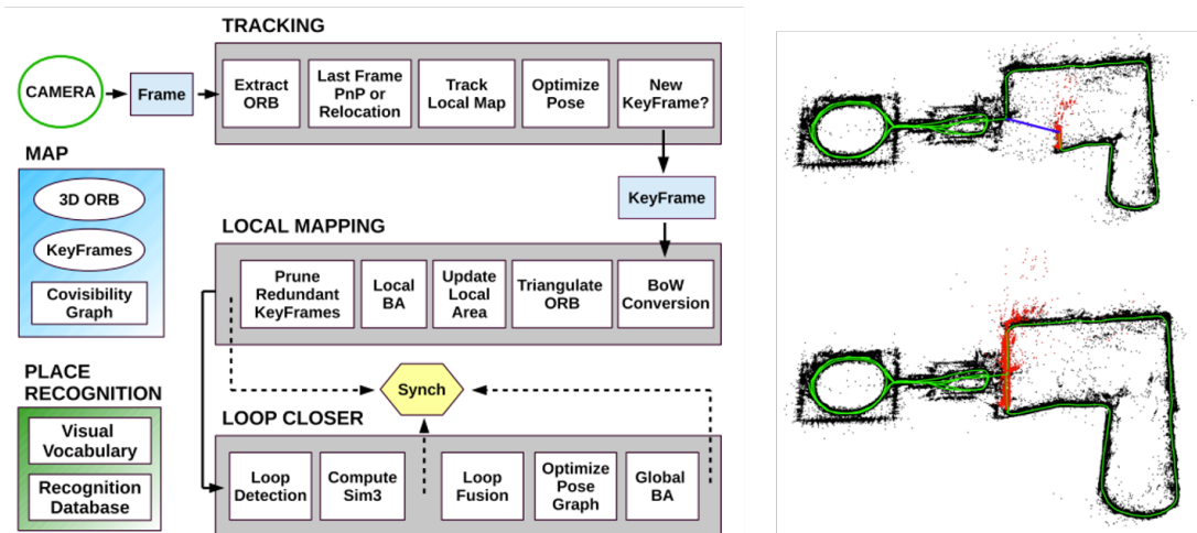
Figure 4.2 – The pipeline and an example of loop-closure executed by ORB-SLAM [77]). In the left side shows the pipeline of ORB-SLAM, three threads represent tracking, local mapping and loop closer respectively (Figure from [77])
