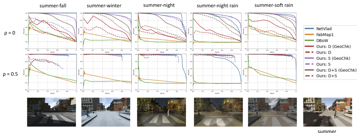
Figure 9.6 – The PR-Curves ( x,y for recall and precision) demonstrate that our BiG descriptor outperforms DBoW and FabMap on all conditions by all layer combinations and show better results against NetVlad under rainy weather conditions. The improvement of \rho and geometric checking can also be observed in the comparison between first and second row, dot line and solid line. In the legend, D and S are Depth and Semantic layers respectively, D+S is the combination of two layers.
