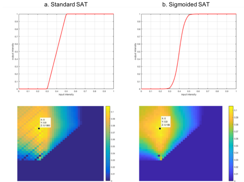
Figure 6.9 – Comparison between standard SAT function and sigmoid-smoothed SAT function wrt \mathbf{u} = (0.3, 0.5)^\top . Second row shows the conditional mutual information MI(I^*, I|I^0) computed by Eq. (6.14), notations keep as aforecited for I^* and I with I^0 generated by the optimal contrast band from MI(I^*, f_{SAT}(I, \mathbf{u})) . We see clearly that standard SAT causes aliasing-like effect in the landscape, due to derivative discontinuity at cutting points a, b
