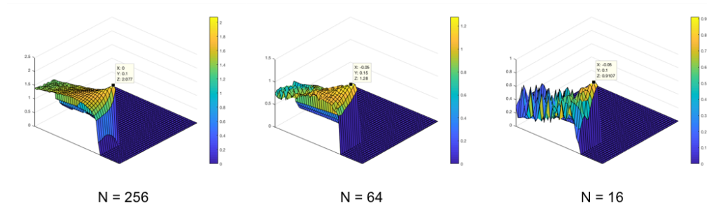
Figure 6.8 – Lowering the number of histogram bins (which is classical for image alignment tasks) leads to a difficult-to-optimize cost function landscape during illumination estimation process (axis represent parameters a and b of contrast band \mathbf{u} = (a, b)^T ).
