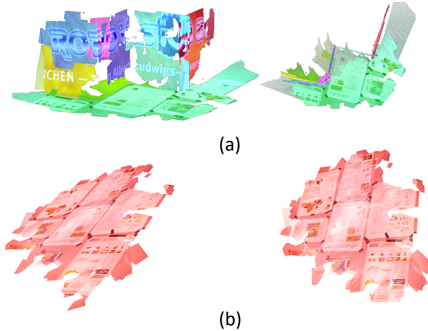
Figure 8.6 – 3D multiple (subfig a) and single plane map (subfig b) of the dataset TUM [113] generated by our method. Our proposed method is able to estimate camera trajectory and planar map representation simultaneously.
