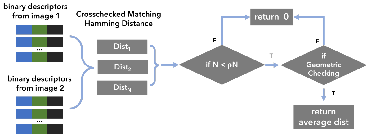
Figure 9.5 – A pipeline of the matching process of two descriptors. The result is controlled by two stages: it outputs zero (most dissimilar) when low matching number than \rho N after a crosschecked matching or high geometric checking error.
