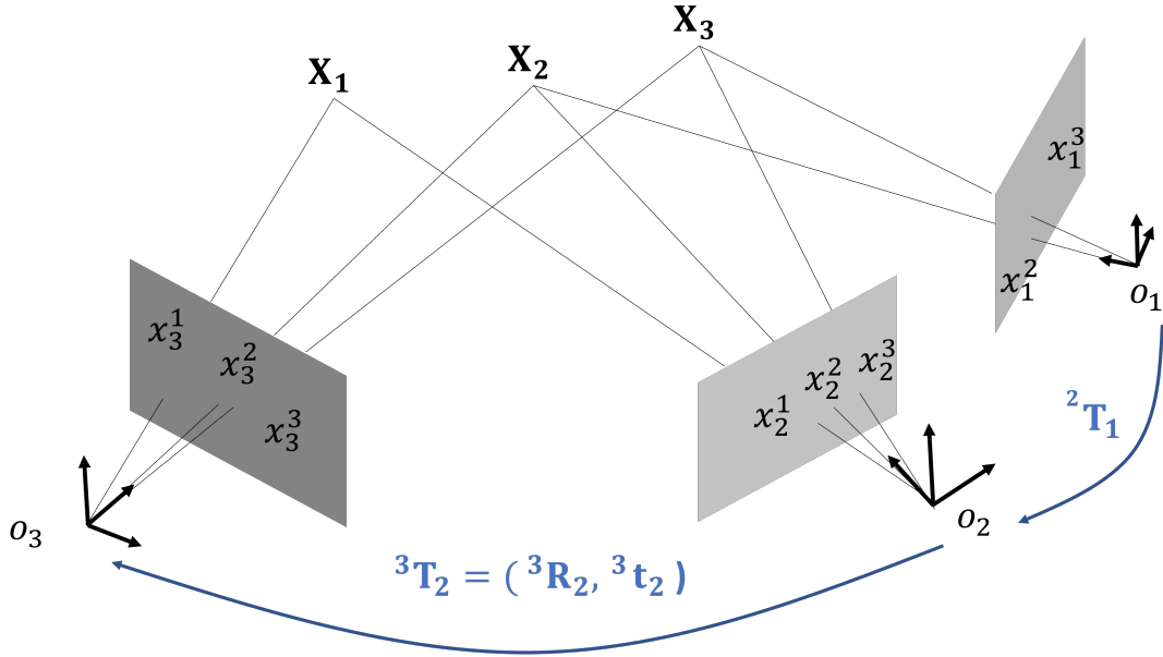
Figure 3.5 – Bundle Adjustment, in general, is defined as a nonlinear minimization on a sequence of multiple views and landmarks w.r.t to each camera pose and 3-D position of landmarks. An example is given here for three camera poses and three landmarks.
