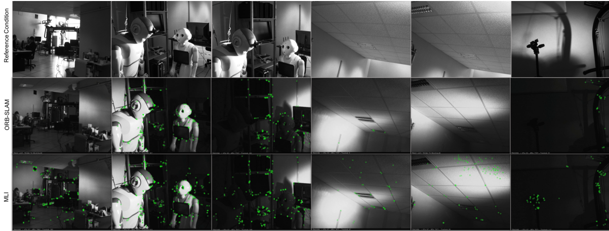
Figure 6.11 – Results of real scene against dynamic illumination variance. With a keyframe map generated under reference condition, MLI shows a better retrieve capacity especially when encountering non-uniform illumination variance. In contrast, standard ORB-SLAM only tracks the well lighted parts in the image.
