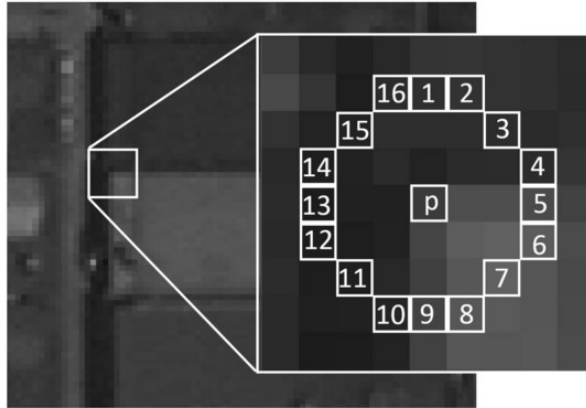
Figure 3.7 – An example of Fast detecting Bresenham circle of 16 pixels and their indexes.
