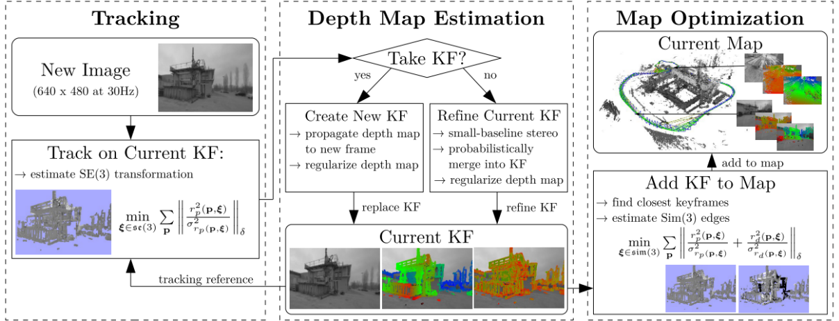
Figure 4.3 – The pipeline of direct method LSD-SLAM, the tracking is performed on high gradient intensities, and the mapping part relies on estimation of Sim3 edges in a pose-graph optimization. LSD-SLAM has a loop-closure module via appearance-based image retrieval method (Figure from [34])
