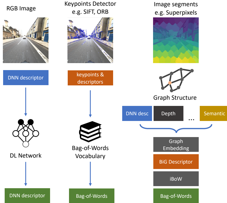
Figure 9.1 – We propose a generic graph binary descriptor on multiple heterogeneous image layers which supports iBoW for robust and efficient loop detection in SLAM applications.
