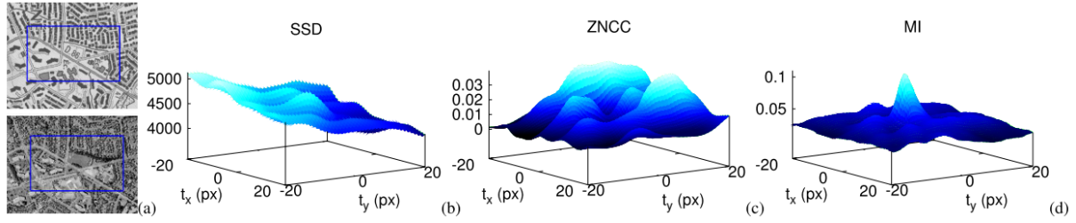
Figure 4.11 – Image registration results w.r.t translational changes between an aerial images and a map layout: MI shows a decent optimum near the zero translational distance, whereas the SSD and ZNCC give relative less apparent responses for optimization purpose. (Figure from [29]).
