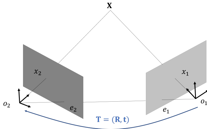
Figure 3.3 – A geometric example of epipolar constraint, in which the \mathbf{x}_1, \mathbf{x}_2 are homogeneous image coordinates of \mathbf{X} a 3-D point \mathbf{X} . The Euclidean transform between two cameras is defined by (\mathbf{R}, \mathbf{t}) \in SE(3) . The intersections of the translational vector \mathbf{t} and two image planes are called epipoles: (e_1, e_2) .
