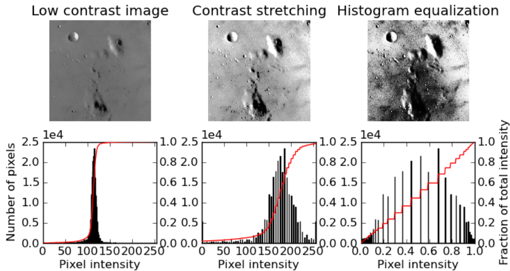
Figure 3.6 – An example of contrast stretching and histogram equalization on a low-contrast image. Images are shown at the first row and histograms are shown in the second, with red curve representing the accumulated histogram.
