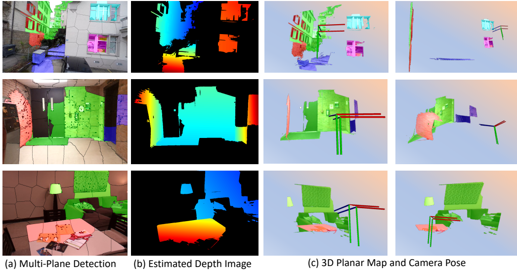
Figure 7.3 – Demonstration of results estimated from image pairs. Depth image and 3D planar maps are also illustrated showing that our method estimates well under the multi-planar environment. Result (c) shows that our method conserves well the orthogonality among planes without relying on the Manhattan assumption.
