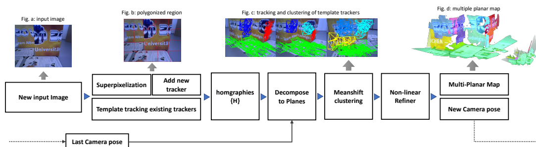
Figure 8.2 – Pipeline of our system which process input image sequence (subfig.a) to superpixelization (subfig.b). In subfig.c, tracking and clustering template trackers are undertaken (different color represent different found planes in 3D, see subfig.d). Pass through the module of refiner, our method is able to recover camera trajectories and a dense planar environment which conserves well perpendicularity without applying Manhattan assumptions.
