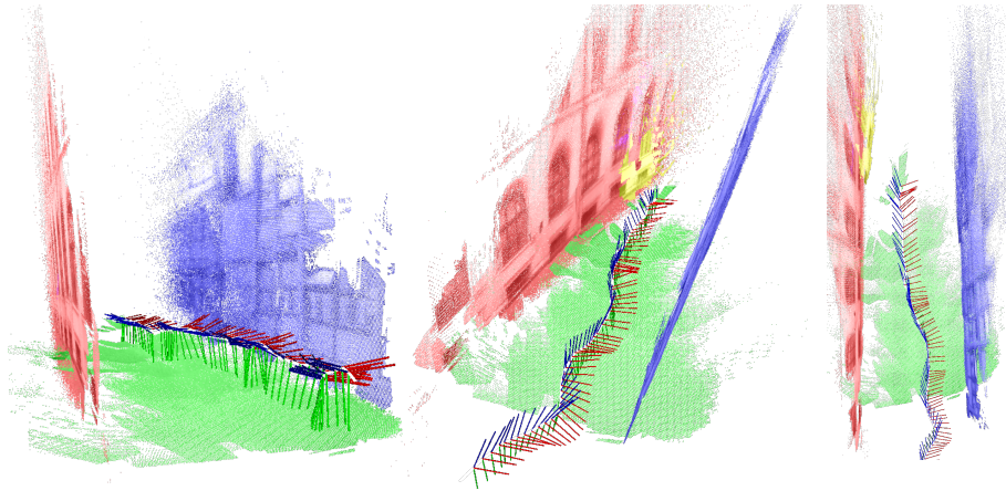
Figure 7.7 – Experiment on an outdoor dataset [35], coordinates represent the camera pose of keyframes. The multi-planar structure is well conserved without applying any assumptions under a corridor-like environment.
