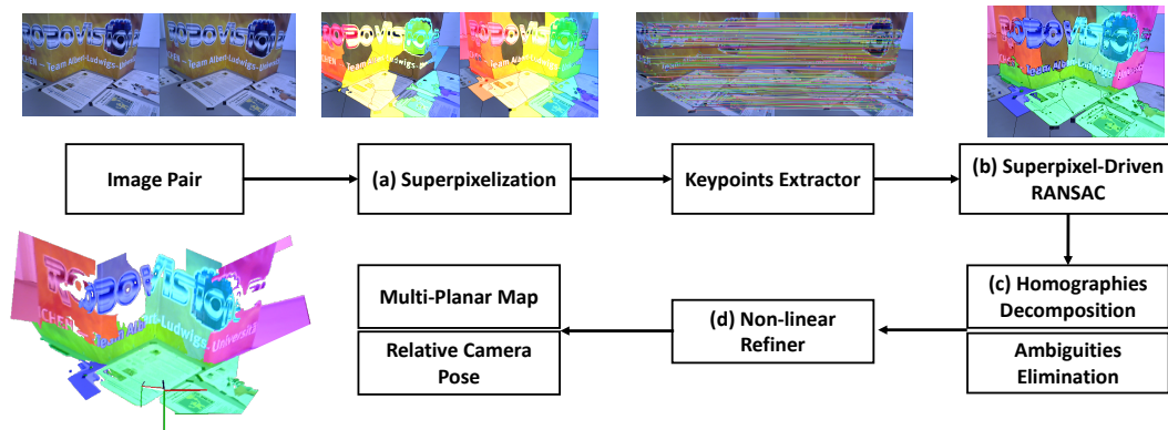
Figure 7.2 – Pipeline of our system which generates a relative camera pose and a 3D multi-planar map from a pair of color images.
