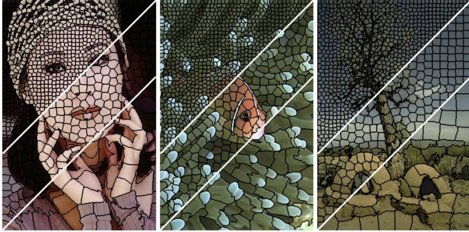
Figure 3.9 – Examples of SLIC superpixel segmentation on different size parameters. SLIC can output compact and regular superpixels of required size parameter with relative low overhead, figure from SLIC paper [1].
