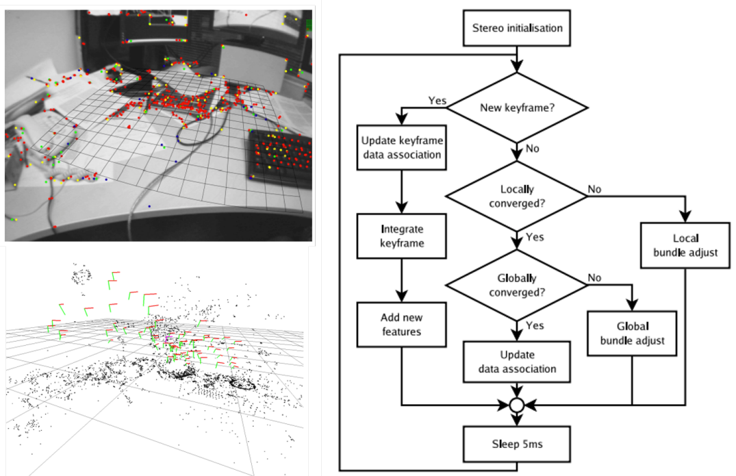
Figure 4.1 – An example of PTAM system on tracking (left-up) and mapping (left-bottom) ends with its pipeline (right), left-up subfigures shows the tracking view of PTAM and corresponding keypoints in a generated point cloud map. The three-dimensional view of the generated point cloud map and computed poses are demonstrated on the left-bottom side. The right side displays the pipeline of the PTAM system (Figure from [62]).
