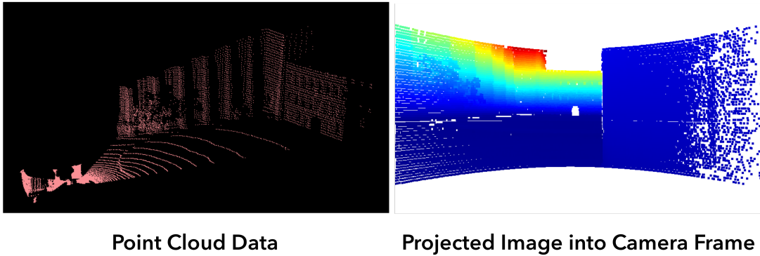
Figure 9.4 – We project point cloud data into 2D depth images along the camera frame coordinate. The blank arc regions are caused by the limited field-of-view of Lidar device.
