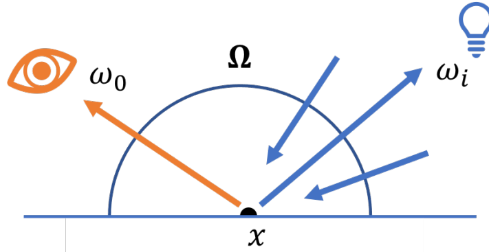
Figure 4.7 – Render equation depicting the observer’s incoming radiance as an addition between emitted radiance at location \mathbf{x} , a hemisphere integration of BRDF function and incoming light.
