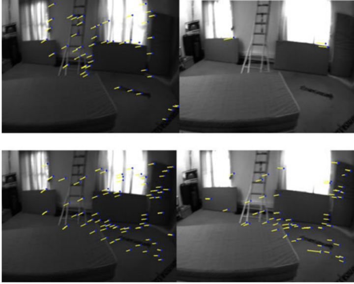
Figure 4.10 – Difference of KLT tracking results before and after gain adapting operation. First row: KLT tracking on original image; second row: gain adaptively transformed of identical images. Note that the traditional KLT method is prone to be influenced by intensity changes as it anchors on photometric error measure (Figure from [14]).
