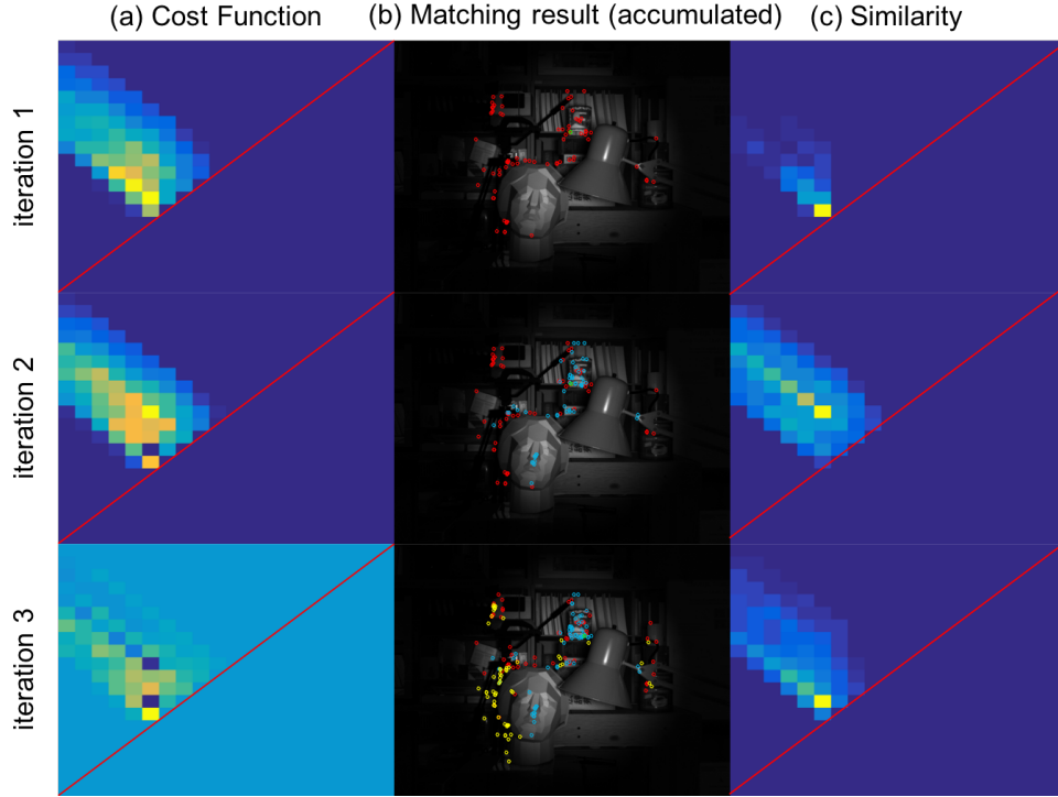
Figure 6.4 – Evolution of MLI layers: (a)(c) represent heatmaps of cost function C^i(\mathbf{u}) and similarity M_{sim}^{\mathbf{u}_i}(\mathbf{u}) in each iteration. (b) demonstrates accumulated matched ORB keypoints against reference image. In each heatmap, vertical and horizontal axis represents \mathbf{u} = (a, b)^\top respectively with a < b .
