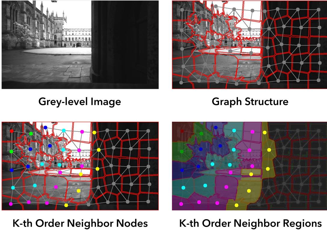
Figure 9.3 – A graph structure of superpixel connected regions is generated from an input image (left upper), red contour and gray nodes and vertices (right upper); given the center vertex of the red superpixel at left upper corner, we find k -th order neighbour vertices with different colors (red for k = 0 , green for k = 1 , etc.) (left lower) ; k -th order neighbour regions are highlighted in the image (right lower). Image from the Newer College Dataset [92].
