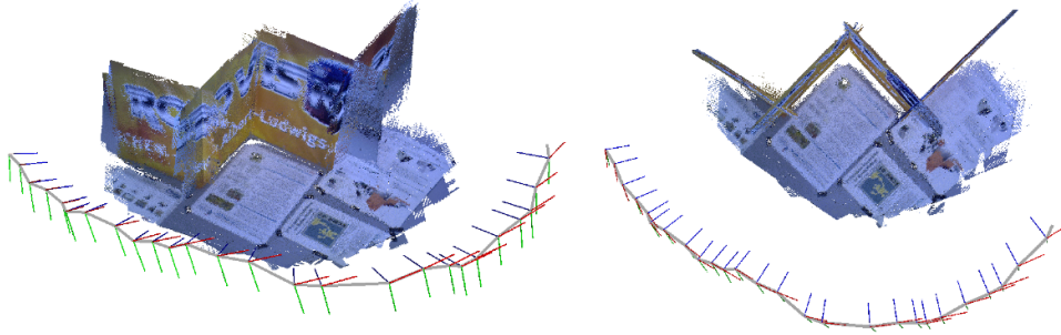
Figure 7.5 – 3D multiple plane map and camera trajectory of the dataset TUM [113] generated by our method.
