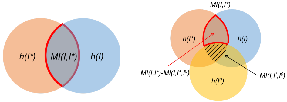
Figure 6.6 – Mutual information between two images (left), and three images (right) defined as the shared entropy between images.
