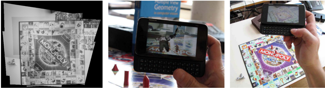
Figure 4.5 – A demonstration of a homography-based SLAM [86] and AR system implemented in a mobile phone. It recovers camera poses, then displays virtual character and does the dense mapping.
