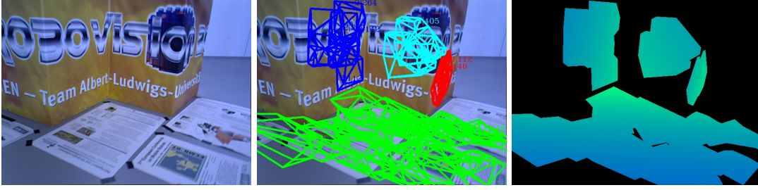
Figure 8.4 – Clustered and matched template trackers (middle) and correspondent generated depth at trackers region (right).
