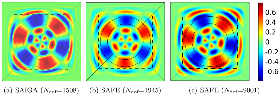
Figure 4.13 – Displacement U_r shape for a flexural mode ( F(3,3) ) at the frequency of f=0.5 MHz and C_{ph}=3791 m/s (a) SAIGA with p = 3, N_{\text{dof}}=1508 (b) SAFE with p = 3, N_{\text{dof}}=1945 (c) SAFE with p = 3, N_{\text{dof}}=9001
