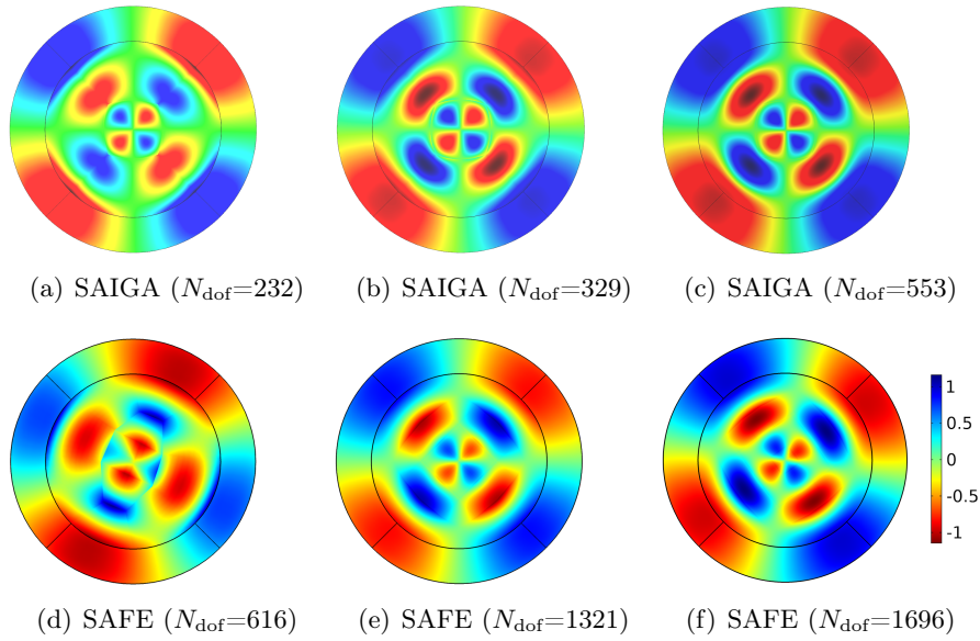
Figure 4.10 – Displacement mode shape ( U_r ) of a flexural mode ( F(2,2) ) at low frequency ( f=0.5 MHz) and C_{ph}=2452.5 m/s: (a,b,c) SAIGA with p=3 ; (d,e,f) SAFE with p=3
