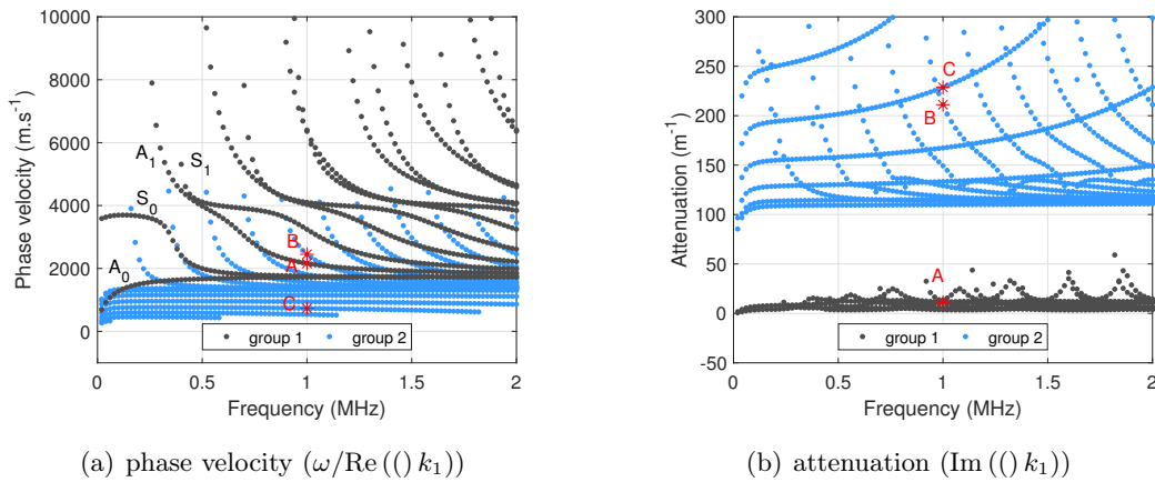
Figure 6.2 – Dispersion curves of a free poroelastic bone layer; groups 1 and 2 represent low and high attenuated waves, respectively; a filtering criteria \bar{\gamma} = 100 \text{ m}^{-1}
