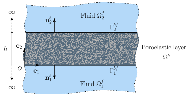
Figure 6.1 – Schematic of a two-dimensional poroelastic waveguide coupled with infinite fluids
