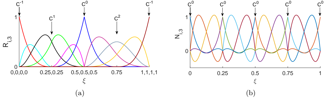
Figure 3.3 – (a) NURBS basis functions of order p = 3 with knot vector \Xi = \{0, 0, 0, 0, 0.25, 0.25, 0.5, 0.5, 0.5, 0.75, 1, 1, 1, 1\} with different desired continuities (b) Lagrange basis function of the same order of a non-avoided C^0 continuities across the elements boundaries
