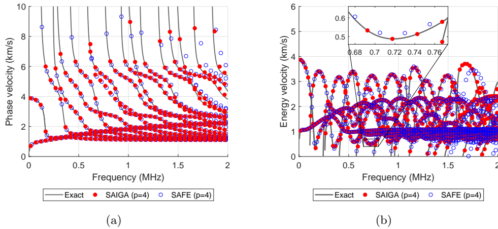
Figure 3.8 – Phase velocity (a) and energy velocity (b) of a multilayered plate: analytical solution and numerical solutions obtained by SAIGA and SAFE methods ( p = 4 , N_{dof} = 66 ).
