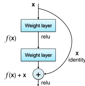
Figure 3.4 – Residual skip connection.
