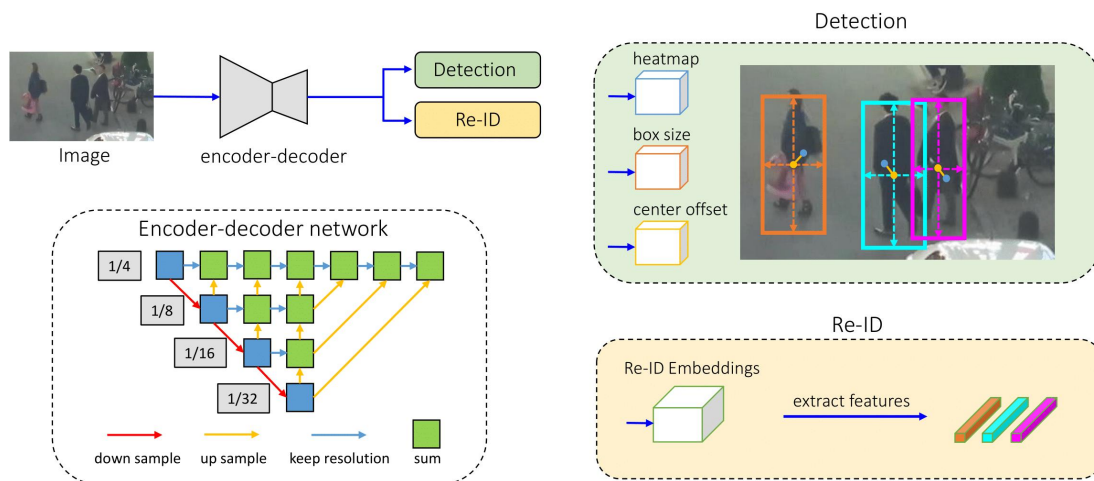
Figure 2.7 – Architecture of one-shot FairMOT tracking model proposed in [Zhang 2020b] for joint object detection and re-identification (re-ID) in a single network.
