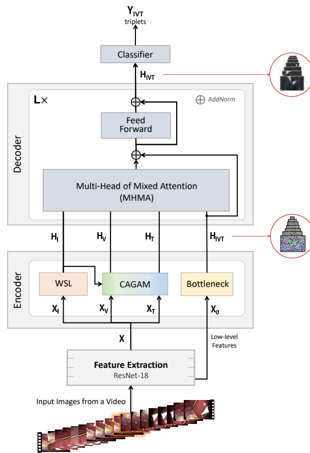
Figure 6.2 – Architecture of Rendezvous: a Transformer-inspired neural network model with multi-head of mixed attention mechanism for surgical action triplet recognition.
