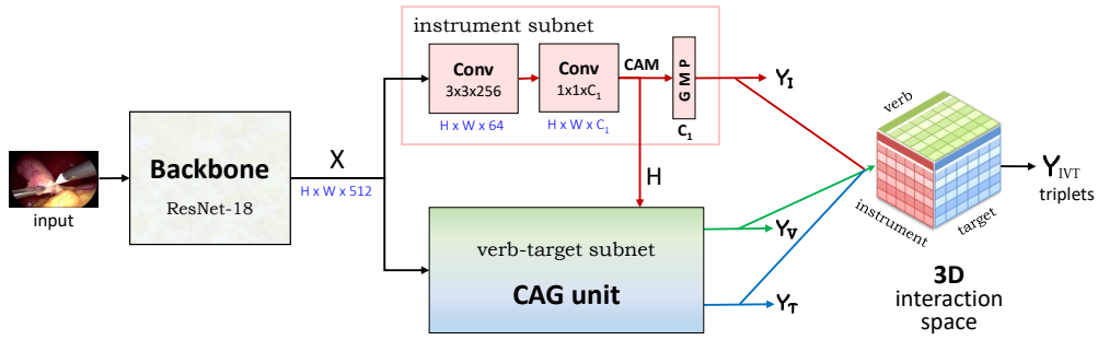
Figure 4.11 – Tripnet: the architecture of the proposed model for action triplet recognition. Feature dimension values ( H = 32 , W = 56 , C_I = 6 )
