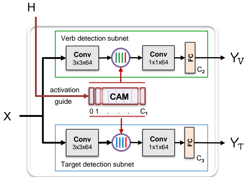
Figure 4.12 – The diagram of the class activation guide (CAG) for a directed detection of the verb and target components of the triplets.
