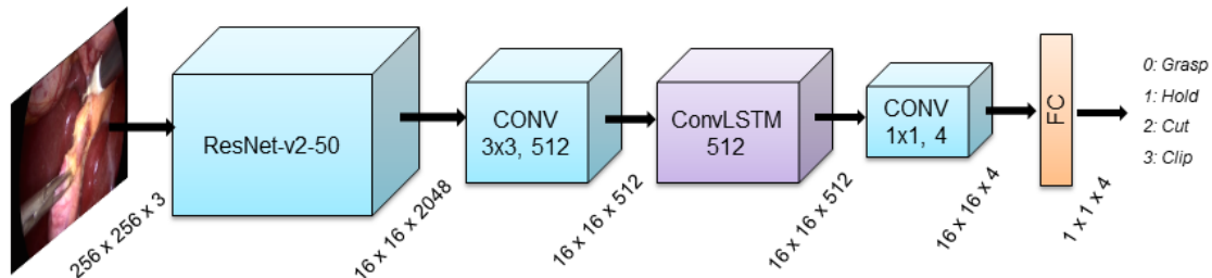
Figure A.6 – The CNN+ConvLSTM spatio-temporal model for action recognition.
