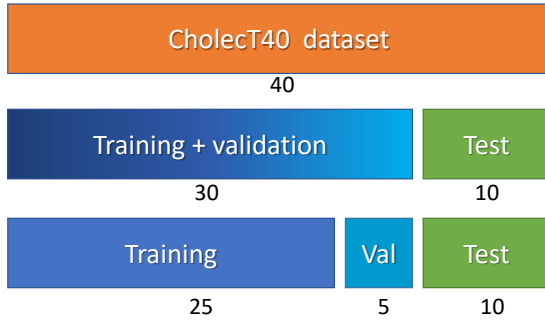
Figure 4.15 – Dataset splits.
