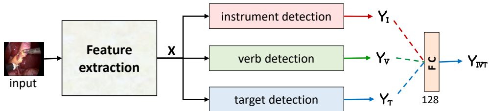
Figure 4.9 – The architecture of a MTL baseline model for action triplet recognition.
