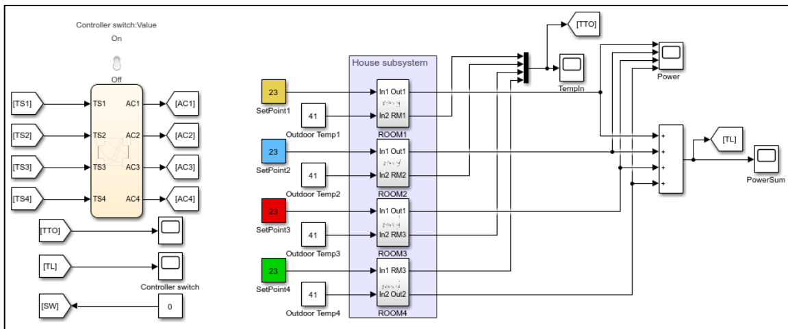
Figure 2.34. Illustration of the 4-AC control logic implementation into the house cooling system model
