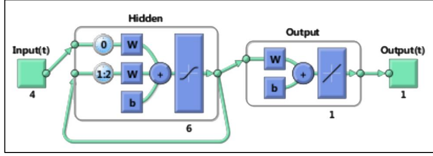
Figure 3.10. Proposed Elman Neural Network Model structure
