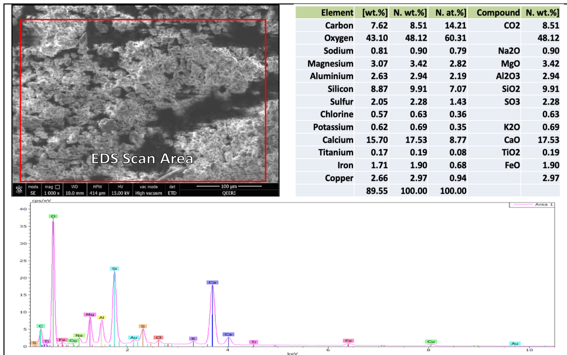
Figure 5.6. EDS analysis of sample air filter
