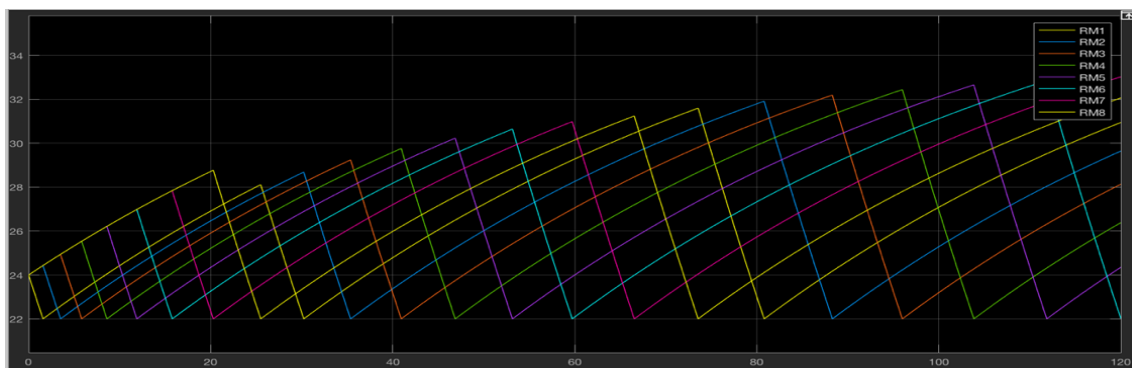
Figure 2.42. Out of control temperature response under ultra-high cooling demand beyond boundary conditions (8-AC system)
