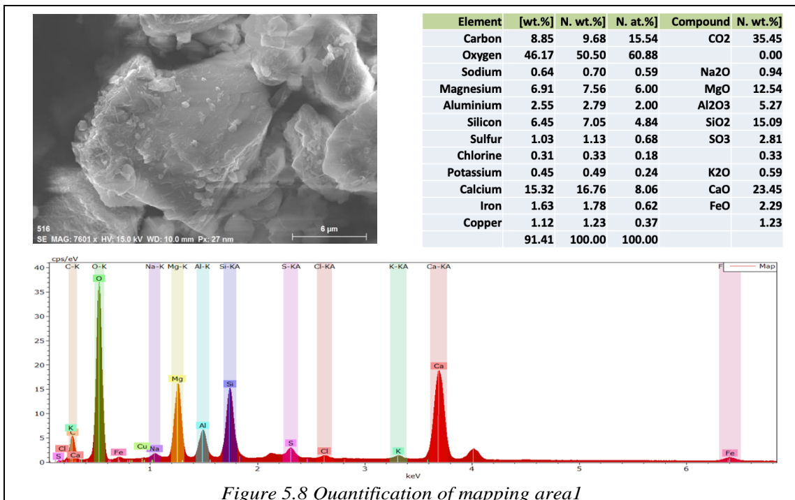
Figure 5.8 Quantification of mapping area1
