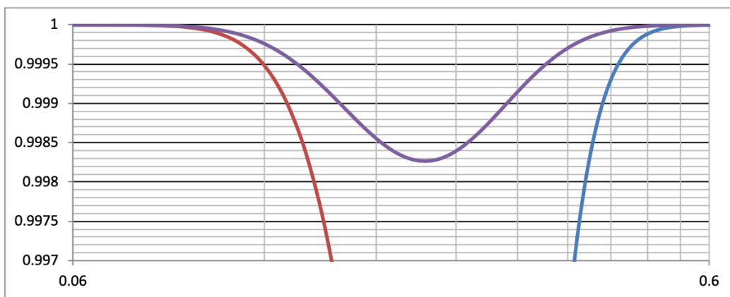
Figure 5.22. Filter efficiency vs particle diameter (zoomed in)
