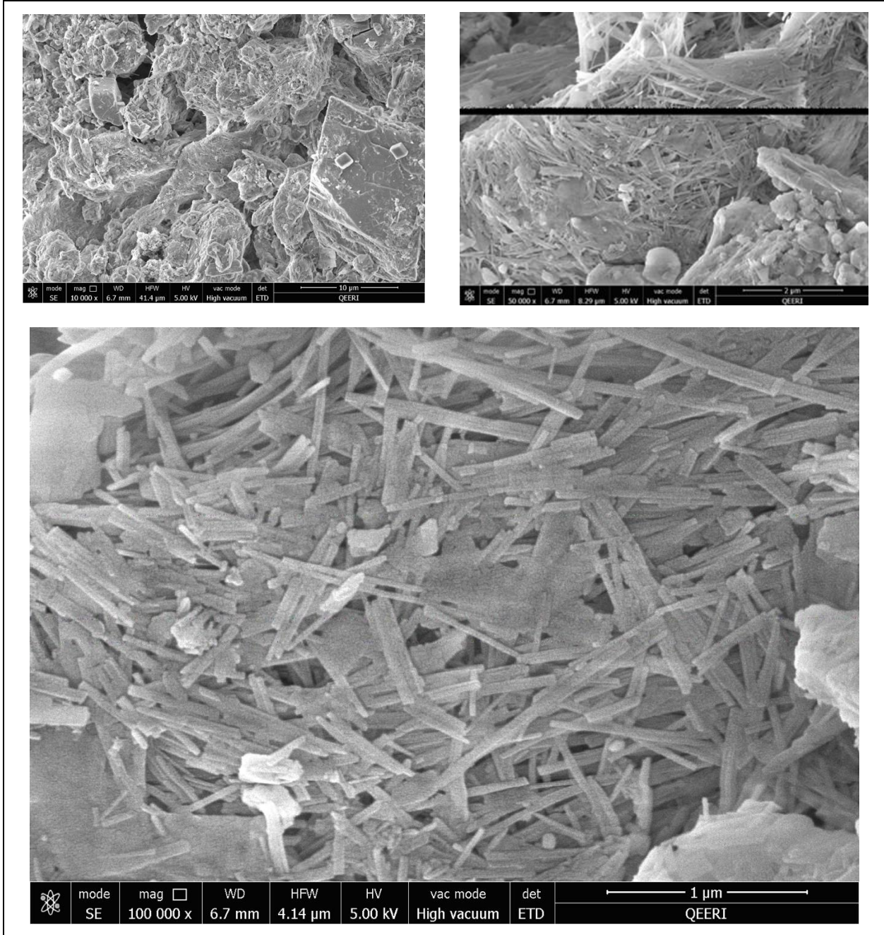
Figure 5.11. SEM analysis of sample 2 (area2)
