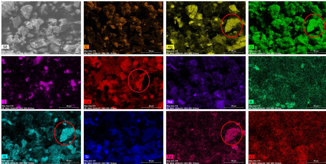
Figure 5.9. Sample ESD mapping (area 1)
