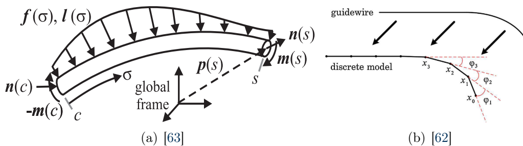
Figure 2.5: (a) [63] Section of a rod from c to s , subject to distributed and internal forces and moments. (b) [62] The guide-wire is separated into linked rigid rods and the tip portion is intrinsically curved.
