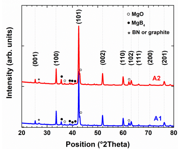
Fig.3-4 XRD analysis of MgB 2 bulks sintered with lot1 and lot2 ex-situ powders
