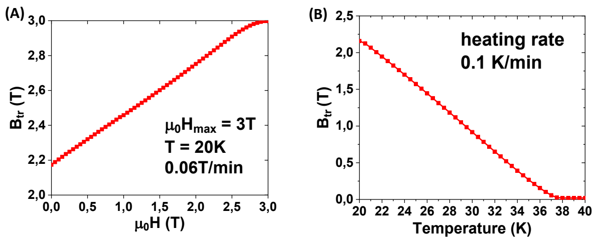
Fig.6-13: (A) Trapped field vs. applied magnetic field for the 20 mm diameter MgB 2 disc at 20 K. The applied field is 3 T, and the reduction rate is 0.06 T/min. (B) Trapped field vs. applied temperature with a 0.1 K/min heating rate.
