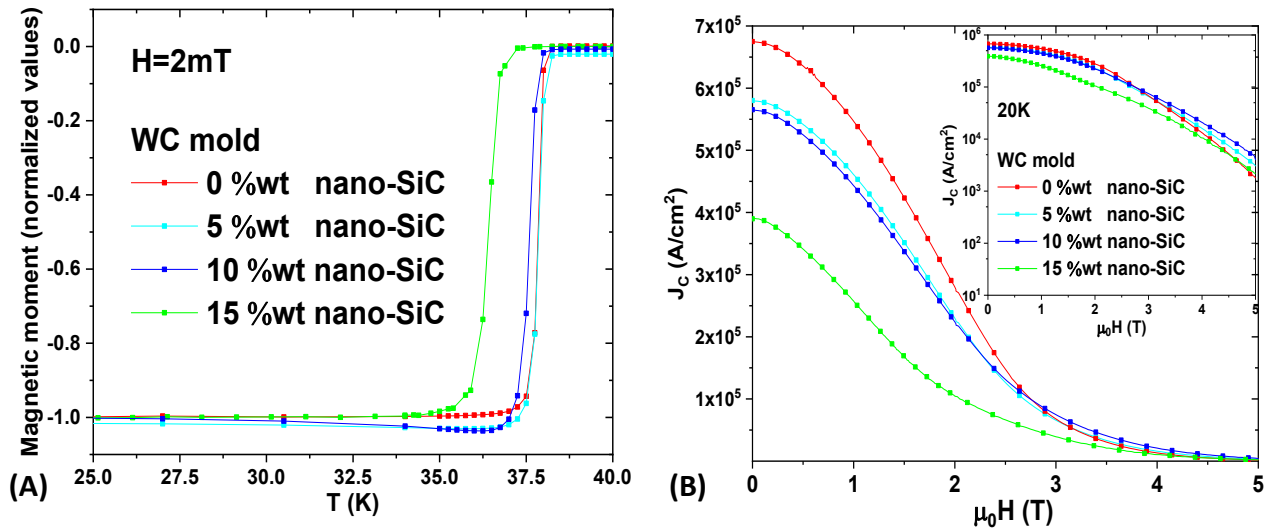
Fig.5-10: (A) Normalized magnetic moment as a function of the temperature for the different amount nano-SiC doped samples sintered in WC mold. (B) Magnetic field dependence of the critical current density J_c at 20 K. The inset shows the same curves on a logarithmic scale.
