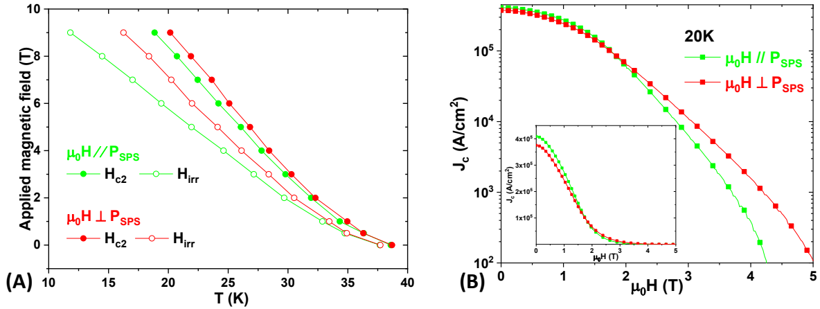
Fig.7-2: (A) Temperature dependence of H_{c2} and H_{irr} for different applied field directions. (B) Magnetic field dependence of the critical current density J_c at 20 K for different applied field directions. The inset shows the same curves on a linear scale.
