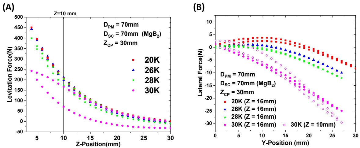
Fig.6-8: Comparison between 20-30 K of the (A) levitation forces and (B) lateral forces of 70 mm diameter and 10 mm thick MgB_2 disc after field cooling at 30 mm from the 70 mm diameter magnet.
