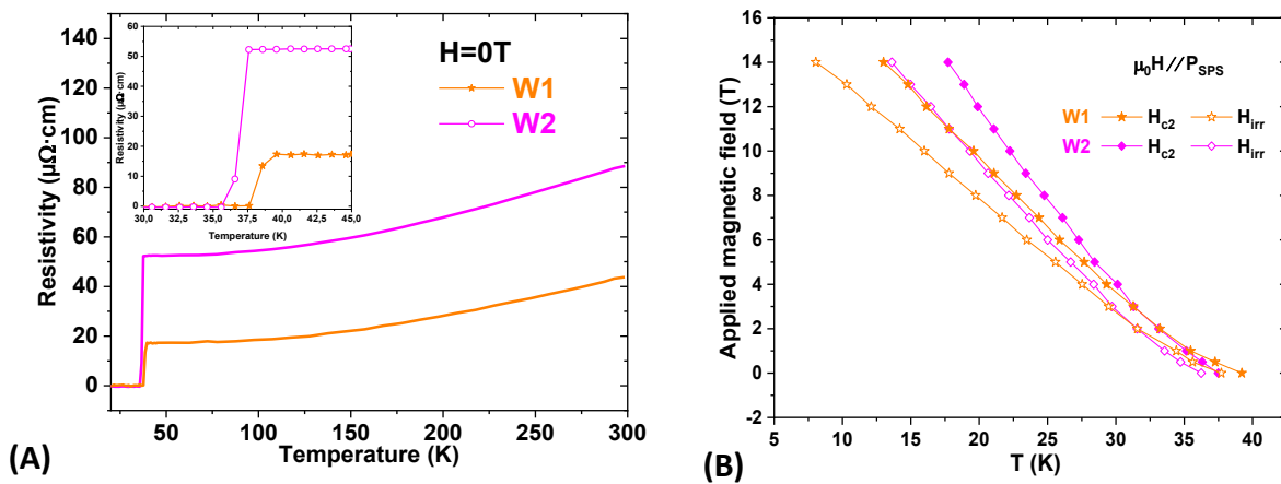
Fig.4-10: (A) Temperature dependence of the resistivity at 0 T with a 5 mA direct current. The inset shows the magnified superconducting transition region. (B) Temperature dependence of H_{c2} and H_{irr} for W1 and W2 samples.
