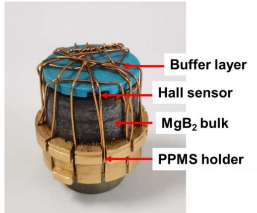
Fig.2-10 Picture of the PPMS sample holder with a MgB 2 bulk
