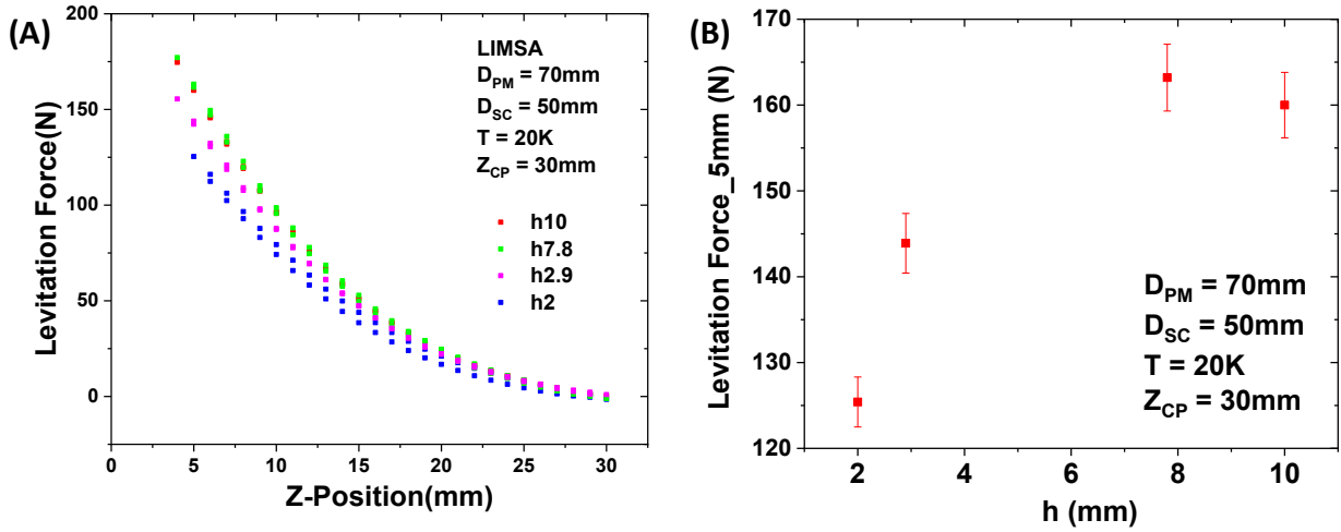
Fig.6-6: (A) Levitation forces carried out with various thick MgB 2 bulks at LIMSA. (B) Levitation force measured at Z_{min} = 5 mm as a function of sample thickness, h .
