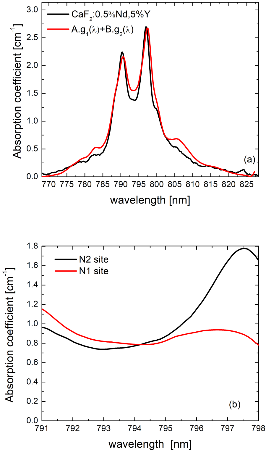
FIGURE 2.12: (a) Experimental absorption coefficient of \text{CaF}_2 : \text{Nd}, \text{Y} (black) compared with a reconstruction of it (red) obtained from a linear combination of the lineshape of the excitation spectra recorded at 1049 nm and 1054 nm. (b) Absorption coefficient of the N_1 and N_2 sites separately.
