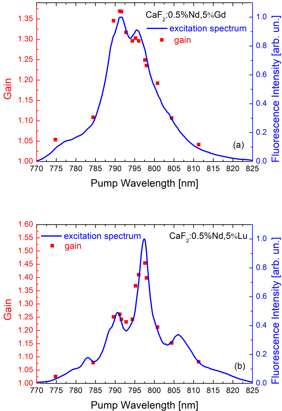
FIGURE 3.10: Excitation spectrum and amplification spectrum varying \lambda_{pump} for CaF 2 :0.5%Nd,5%Gd (a) and CaF 2 :0.5%Nd,5%Lu (b) with P_{pump} = 920 mW, \lambda_{probe} = 1053 nm, P_{probe} = 1 mW, \omega(radius) = 50 \mu m.
