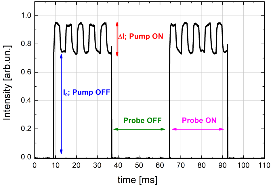
FIGURE 3.7: Typical experimental amplification signal with the double-modulation pump-probe setup.
