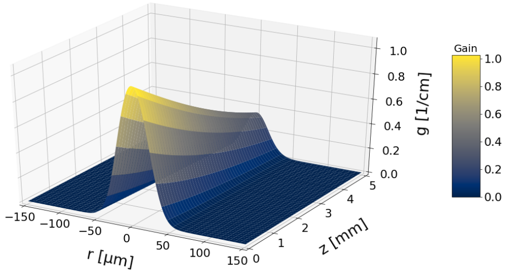
FIGURE 3.4: Gain coefficient per centimeter calculated in small signal conditions for a 5 mm thick \text{CaF}_2 : 0.5\% \text{Nd}^{3+}, 5\% \text{Lu}^{3+} crystal: P_{p,0} = 0.5 \text{W} , P_{L,0} = 1 \text{mW} , \omega_{p,0} = \omega_{L,0} = 50 \mu\text{m} , \lambda_p = 797 \text{nm} , \lambda_L = 1053 \text{nm} .
