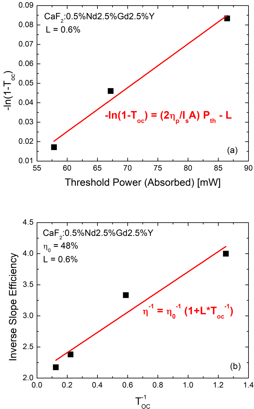
FIGURE 4.13: Passive losses calculation for the CaF 2 :0.5%Nd,2.5%Gd,2.5%Y, performed both with the Findlay-Clay analysis (a) and the Caird analysis (b).
