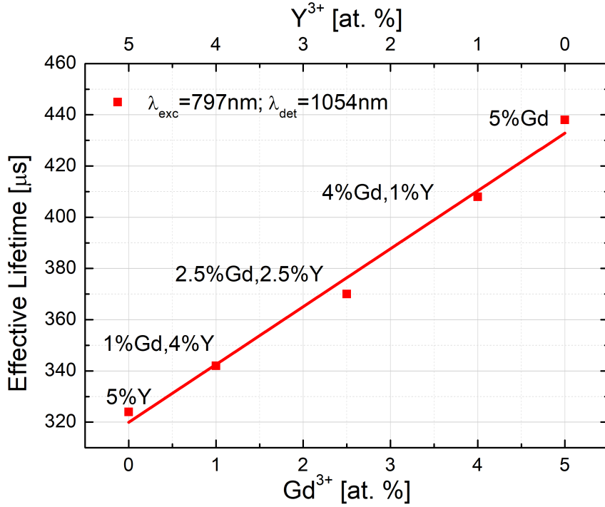
FIGURE 2.19: {}^4\text{F}_{3/2} energy level lifetime concentration trend of \text{CaF}_2 : \text{Nd}, \text{Gd}, \text{Y} for different gadolinium and yttrium concentration, keeping 5% as total buffers concentration.
