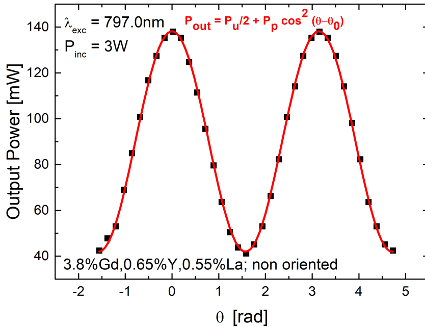
FIGURE 4.5: Birefringence effect in a non-oriented \text{CaF}_2 : 0.5\% \text{Nd}, 3.8\% \text{Gd}, 0.65\% \text{Y}, 0.55\% \text{La} crystal, with pump wavelength of \lambda_{pump} = 797 \text{ nm} and pump power P_{pump} = 3 \text{ W} .
