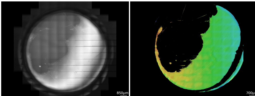
FIGURE 4.18: Sensofar picture before thermal treatment, bright field (left) and qualitative roughness. Molecular adherence is present on roughly 30% of the sample.
