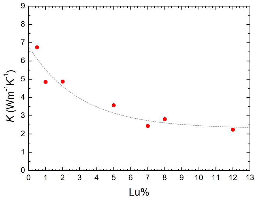
FIGURE 1.9: Thermal conductivity in function of Lu concentration in \text{CaF}_2 : \text{Nd, Lu} [15].
