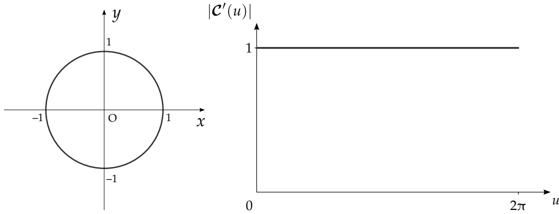
(a) Representation of the curve in \mathbb{R}^2 . (b) Plot of the velocity as a function of the parameter value u .
