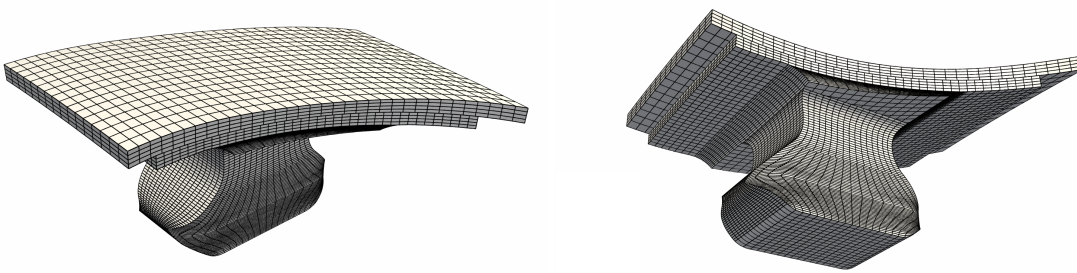
Figure 5.5 – Perspective view of the volumetric geometry of the platform and tenon with parametric lines.
