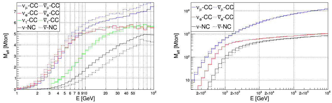
Figure 7.19: Effective mass of ORCA(left) and ARCA(right), computed from the response matrix (eq. 7.17).
