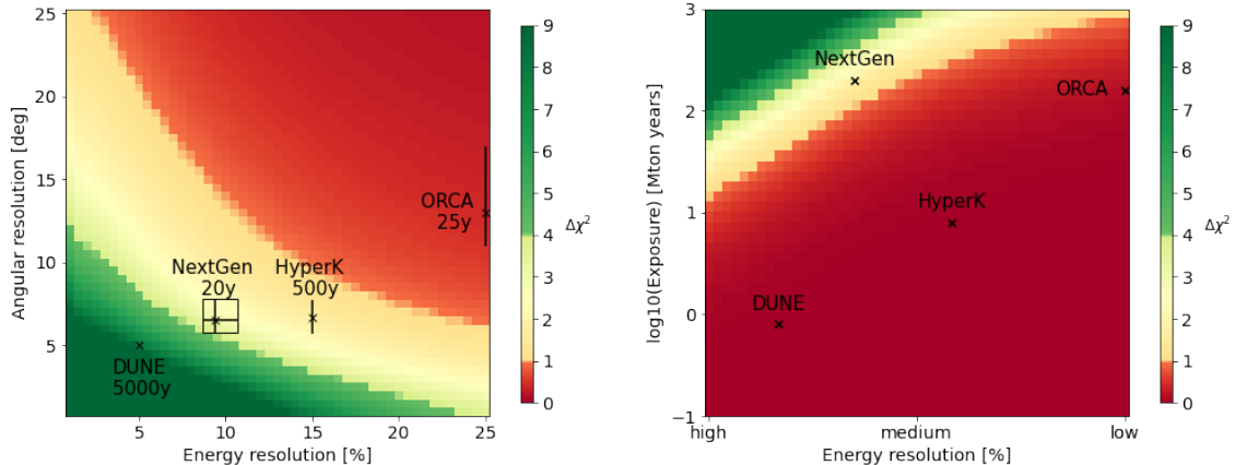
Figure 10.6: \Delta\chi^2 discrimination power for \text{FeNiSi}_2\text{O}_4 vs. \text{FeNiH} for various combinations of detector configurations. Left: Dependency on angular and energy resolution (constant in true neutrino energy) for 200 Mt yr exposure. The respective resolution ranges of the investigated detectors are superimposed together with the necessary livetime to reach the assumed exposure. The error boxes indicate their resolutions in the energy interval of 3 GeV to 7 GeV. Right: Exposure vs. overall resolution, where a linear dependency between angular and energy resolution is estimated from the left plot. All other parameters were set to the value listed for the NextGen detector in Tab. 7.2 for both plots.
