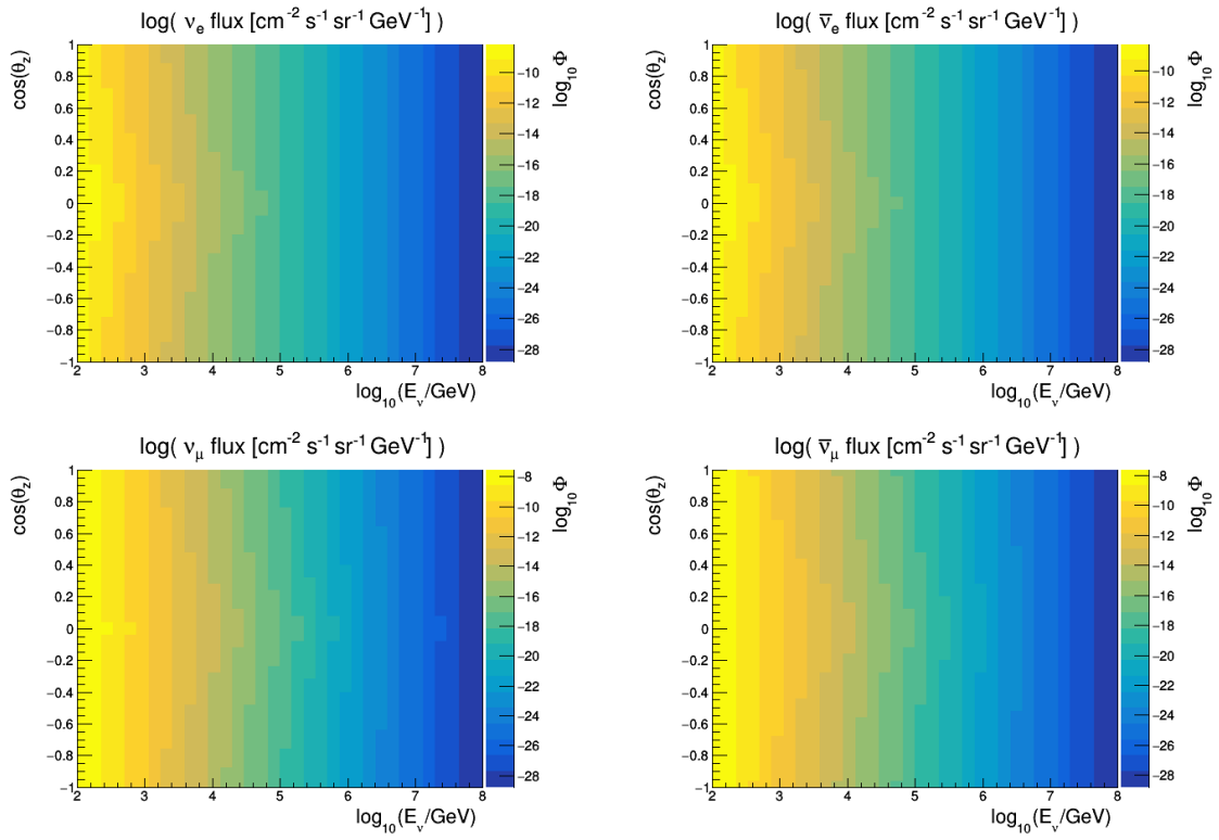
Figure 7.6: Conventional + prompt component of the atmospheric flux for \vec{\nu}_e and \vec{\nu}_\mu per \text{cm}^2 , second, sr and GeV, with logarithmic colorscale. The energy range corresponds to that used in simulations of absorption tomography.
