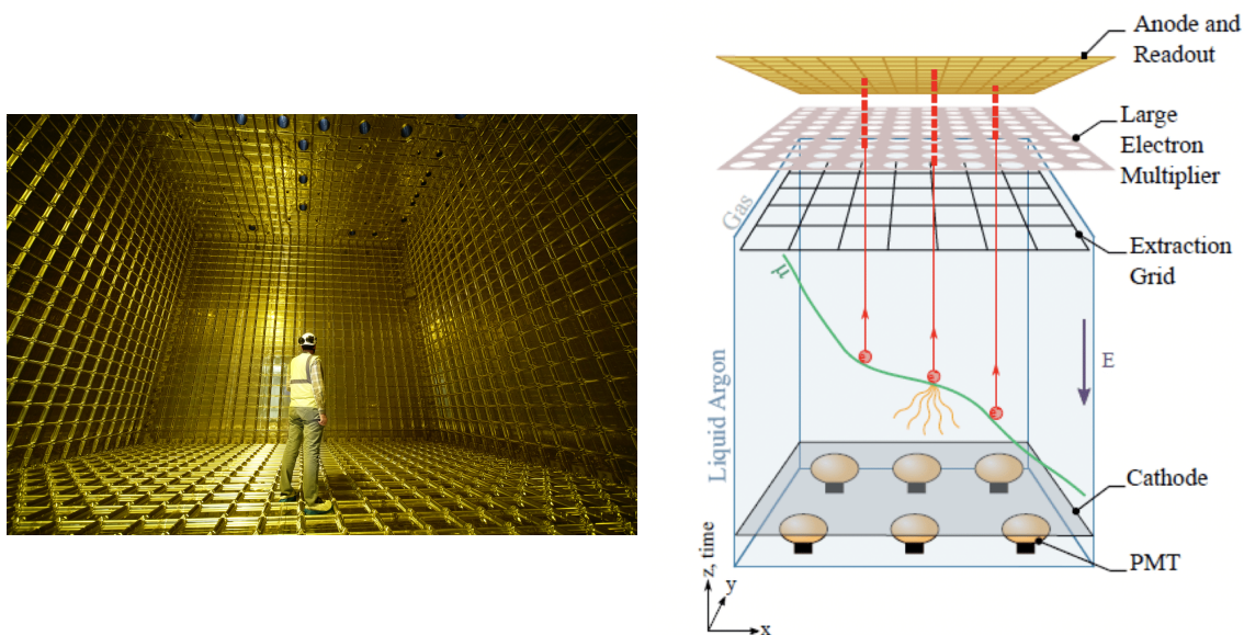
Figure 2.9: Left: Prototype of a DUNE TPC. (Image: Max Brice/Cern); Right: DUNE dual-phase detector principle[99].
