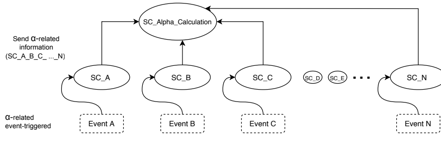
FIGURE 8.1: The SC schema for updating the value of \alpha based on different events captured with the help of SC.
