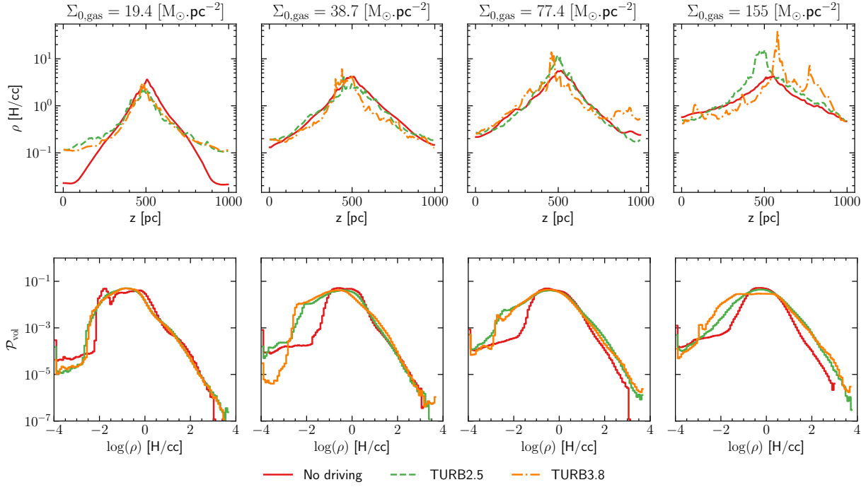
Figure 8.6 – Averaged density profile, top, and density volumic probability distribution function (PDF), bottom. All figures are made from snapshots taken at t \approx 60 Myr. There is less dense gas in the simulations with high initial column density ( \Sigma_{0,gas} \geq 77 M_{\odot} \cdot pc^{-2} ) without driving because most of it has been accreted by the sinks.
