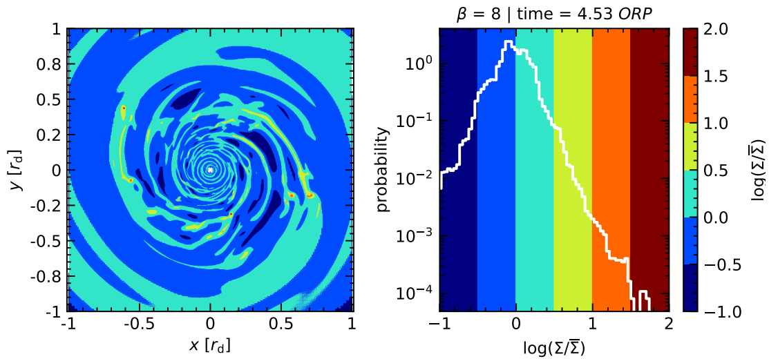
Figure 10.14 – Map of fluctuations of column density \mathfrak{G} = \Sigma/\bar{\Sigma} (left) in logarithmic bins represented on the \Sigma -PDF (right) for \beta = 8 . Dense parts of the PDF ( \log(\mathfrak{G}) > 0.5 ) are only present in some restricted regions of the filaments.
