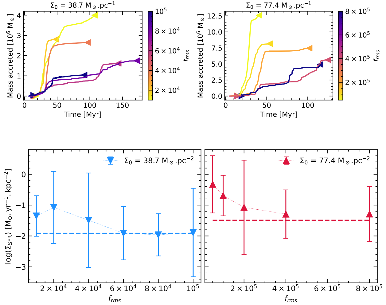
Figure 9.2 – Study of the effect of the intensity of the turbulent driving on the SFR (group STRENGTH). f_{rms} is RMS of the force density in code units. Top: Mass accreted in sinks. The SFR computation starts when 3 % is consumed or lost ( t_{3\%} , left triangle) and ends when 40 % of gas is consumed or lost ( t_{40\%} , right triangle). Bottom: Surface density of star formation rate as a function of the strength of the driving f_{rms} . The value plotted is the accretion rate between t_{3\%} and t_{40\%} and the error bars reflect the standard deviation of all the accretion rates obtained by choosing starting and end points between these two values. The dash line is the value of the SFR given by the SK relation (Kennicutt & Evans, 2012).
