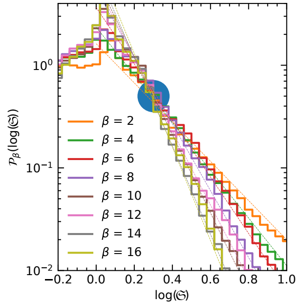
(b) Zoom over the PDFs of Figure 10.4. The value of the PDF is roughly the same for \mathfrak{G}_0 = 2 and is P_0 \approx 0.5 (blue area).
