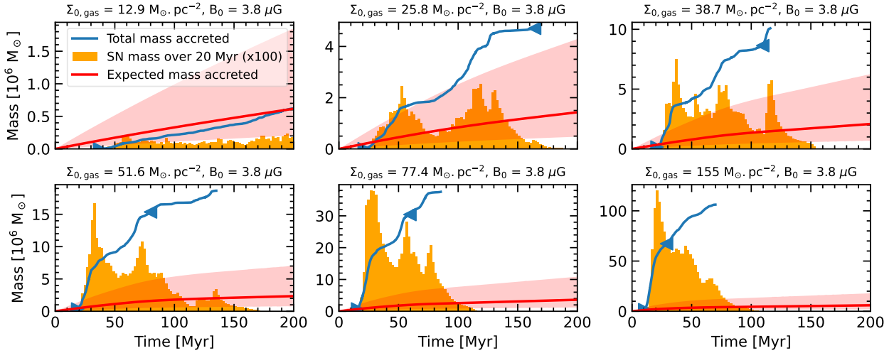
Figure 9.7 – Stellar mass for the group NOTURB. The red line is the stellar mass creation if the SFR in the kpc box equal to 2.5 \times 10^{-3} (\Sigma/10 M_{\odot} \cdot \text{pc}^{-2})^{1.4} M_{\odot} \cdot \text{yr}^{-1} (Kennicutt & Evans, 2012). The red-colored zone corresponds to SFR 3 times higher and lower and aims to represent the spread of the Schmidt-Kennicutt relation. The orange histogram is the mass (multiplied by 100 for readability) of stars that blow up into supernovae in a time span of 20 Myr. The SFR computation for Figure 9.8 starts when 3 % is consumed or lost ( t_{3\%} , left triangle) and ends when 40 % of gas is consumed or lost ( t_{40\%} , right triangle).
