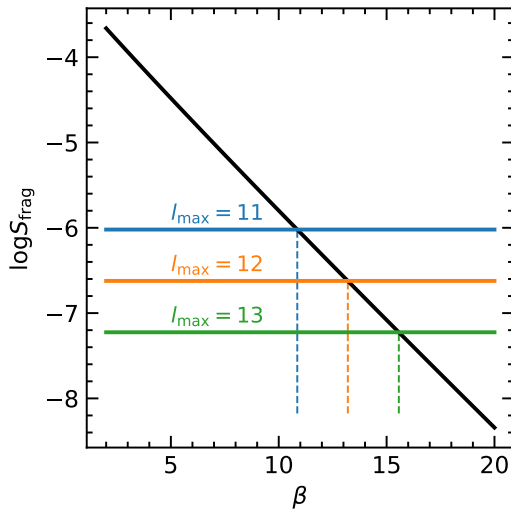
(c) Left: Surface S_{\text{frag}} of the disk with a column density over \mathfrak{G}_{\text{frag}} = 30 as a function of \beta according to Equation (10.26) (in black). The colored lines correspond to the tinniest resolved surface at the indicated level. The vertical dotted lines give an upper bound for \beta_{\text{crit}} at the given resolution, that is a value of \beta for which the fragmented zone (as defined in Figure 10.3) is resolved by at least one cell. Right: comparison between the upper bound for \beta_{\text{crit}} from our empirical model (left panel) and the values measured in the simulations. The bottom of the shaded zone corresponds to the maximal value of \beta for which the fragmented zone is resolved by at least 40 cells according to the model.
