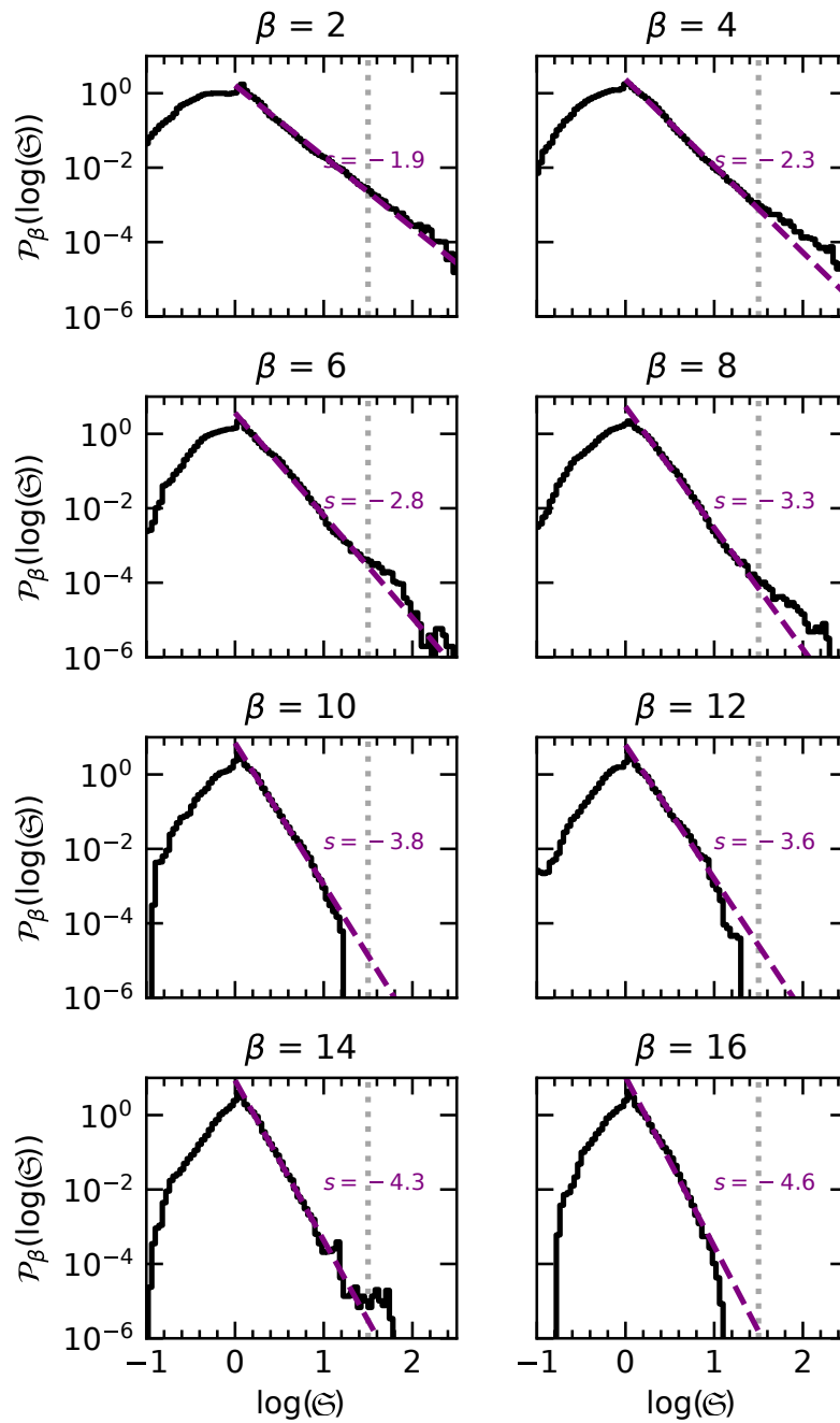
Figure 10.4 – Time-averaged \Sigma -PDF for several different values of \beta (group JR12) with \mathfrak{G} = \Sigma/\bar{\Sigma} . The value of the PDF is averaged bin by bin. The dashed purple line is a fit of the overdense zone (see Figure 10.3) and the vertical dotted grey line corresponds to the limit between the overdense zone and the fragments zone, in accordance with Definition 1.
