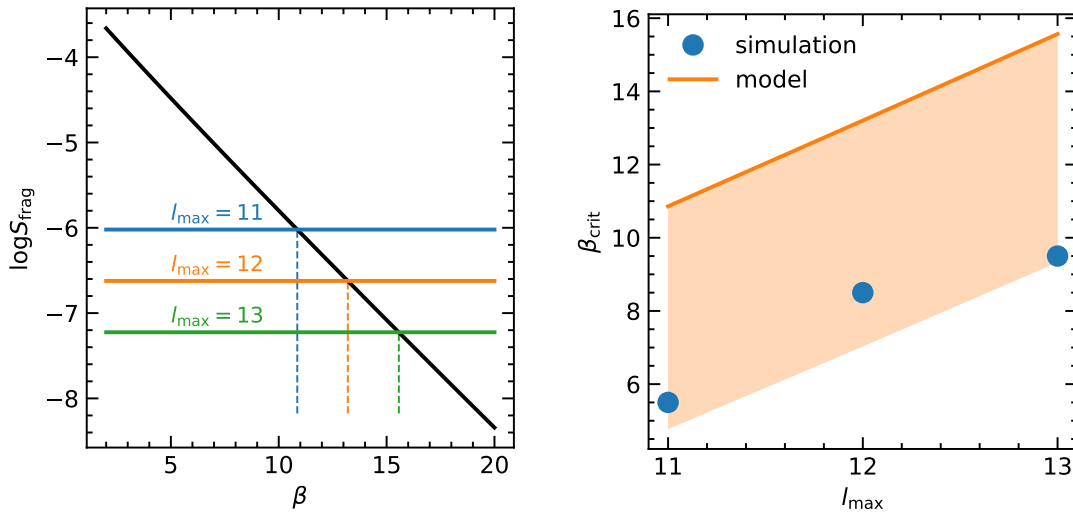
(c) Left: Surface S_{\text{frag}} of the disk with a column density over \mathfrak{G}_{\text{frag}} = 30 as a function of \beta according to Equation (10.26) (in black). The colored lines correspond to the tinniest resolved surface at the indicated level. The vertical dotted lines give an upper bound for \beta_{\text{crit}} at the given resolution, that is a value of \beta for which the fragmented zone (as defined in Figure 10.3) is resolved by at least one cell. Right: comparison between the upper bound for \beta_{\text{crit}} from our empirical model (left panel) and the values measured in the simulations. The bottom of the shaded zone corresponds to the maximal value of \beta for which the fragmented zone is resolved by at least 40 cells according to the model.
