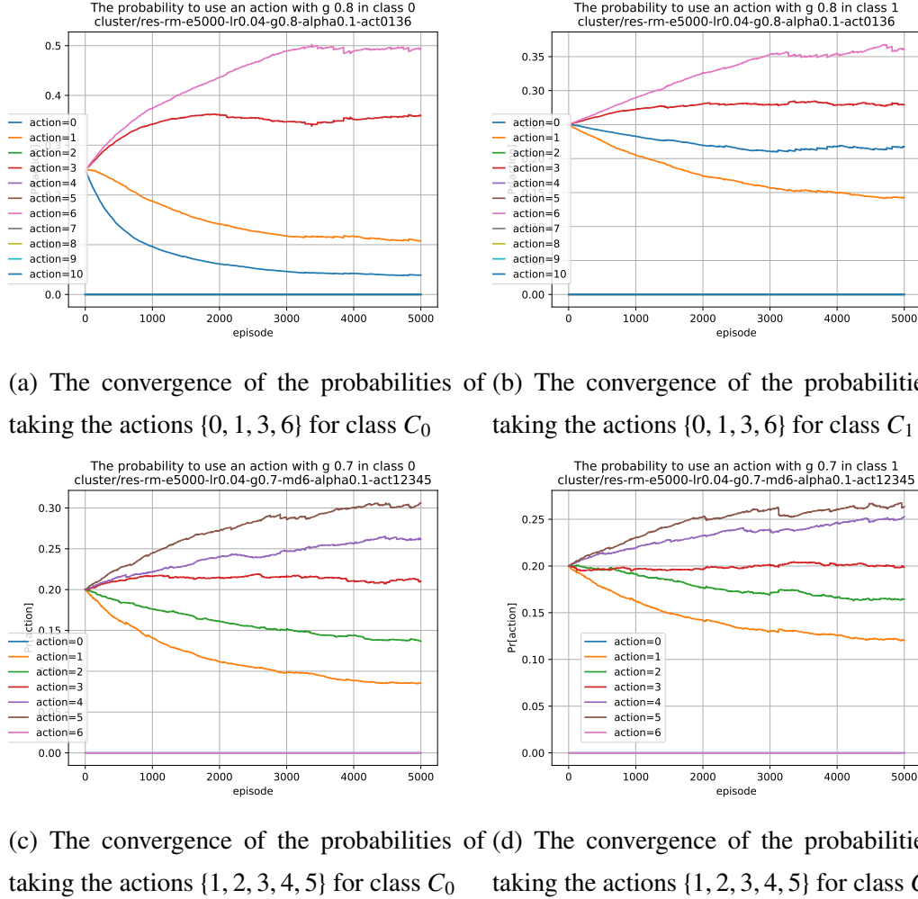
Figure 6.7: The convergence of the probabilities of taking the actions for both classes and for different sets of actions
