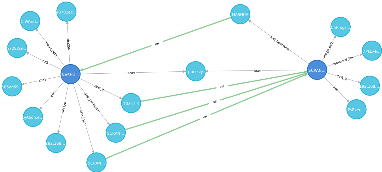
FIGURE 3.2 – \mathbf{G}(\text{psexec})
