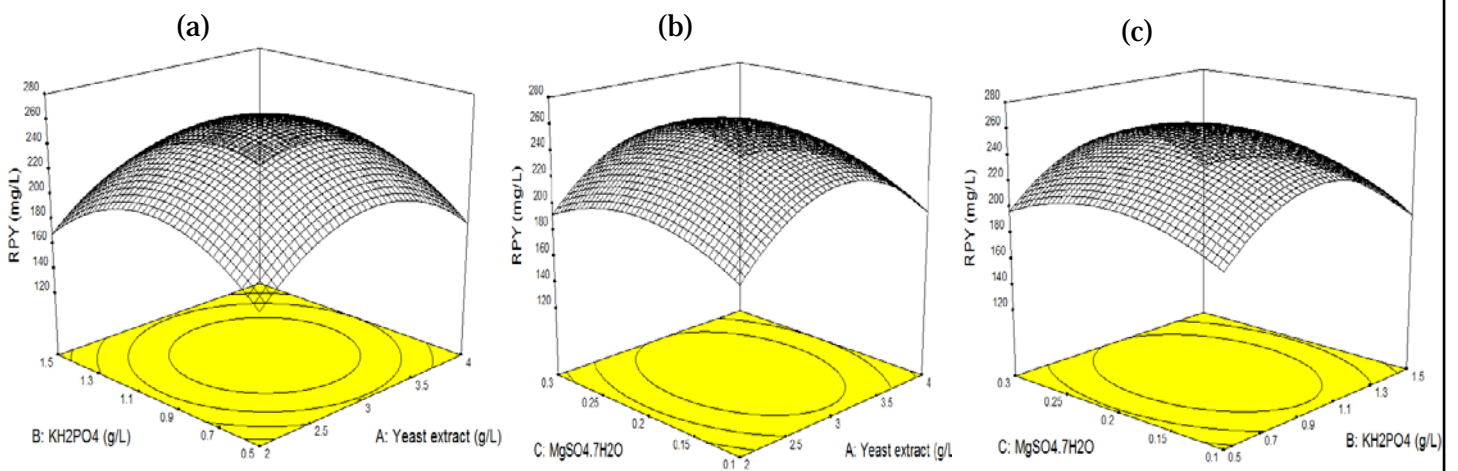
Fig. 3: 3D surface plots showing the interactive effects of factors on red pigment yield (RPY)
