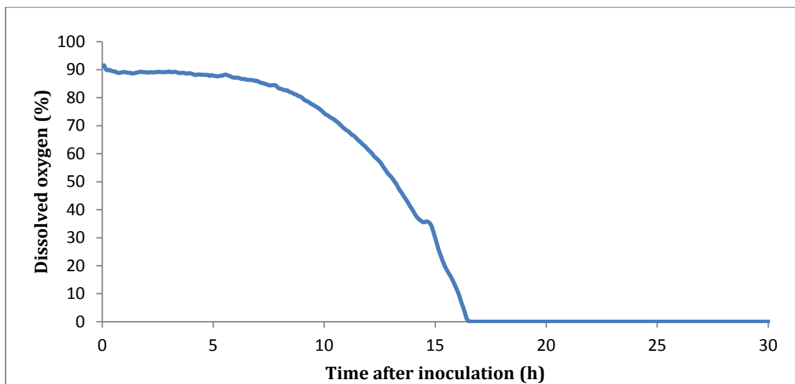
Figure 2: Decreased response of dissolved oxygen (1% DO_2 ) after fungal inoculation at 25 °C when the bubbling was set at 190 ml/min (90% DO_2 ) and stirring at 30 rpm
