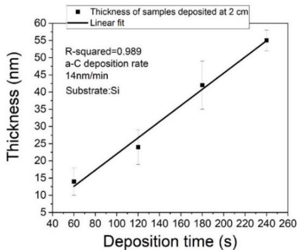
Figure 4.5: Experimental measurements of the a-C thickness on Si versus the deposition time.
