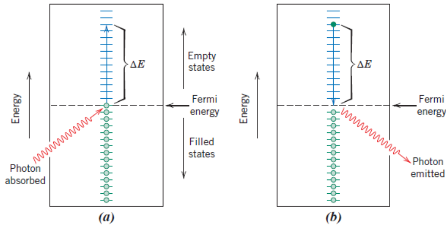
Figure 1.7: a) Schematic representation of photon absorption for metallic materials in which an electron is excited into a higher-energy unoccupied state adapted from [83].
