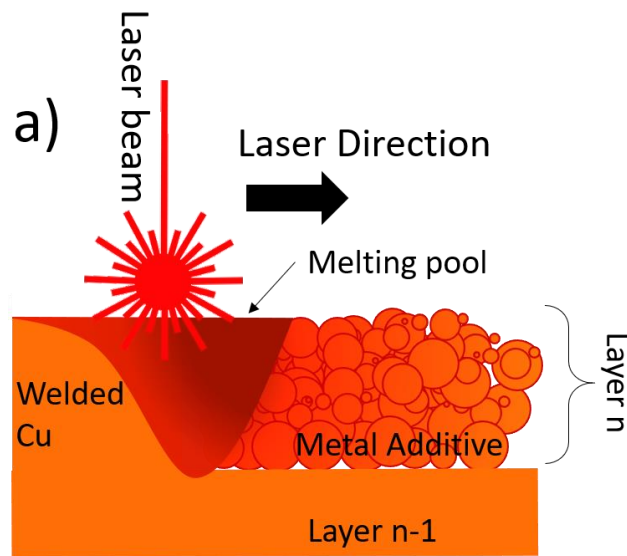
Figure 1.9: Melting pool mechanism of an additive manufacturing process using laser as the source; when the laser scans the powder bed, the metal additive melts, forming a new layer of the printed object [113].
