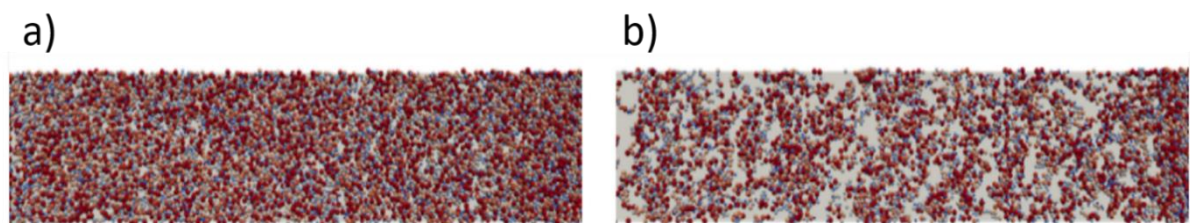
Figure 1.10: Numerical simulations of the layer topography view using 20–44 \mu\text{m} distribution of \text{Ti}_6\text{Al}_4\text{V} . a) The homogeneity of a non-cohesive powder and b) a cohesive powder. The images represent the spreading homogeneity after two layers each layer of 44 \mu\text{m} thickness. Adapted from [133].
