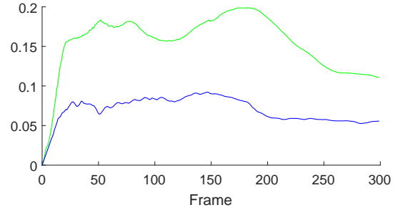
Fig. 4.4.4. RMS error per frame of the 2D simulations depicted in Figure 4.4.3. Blue: Our method. Green: Nielsen et al. [83].
