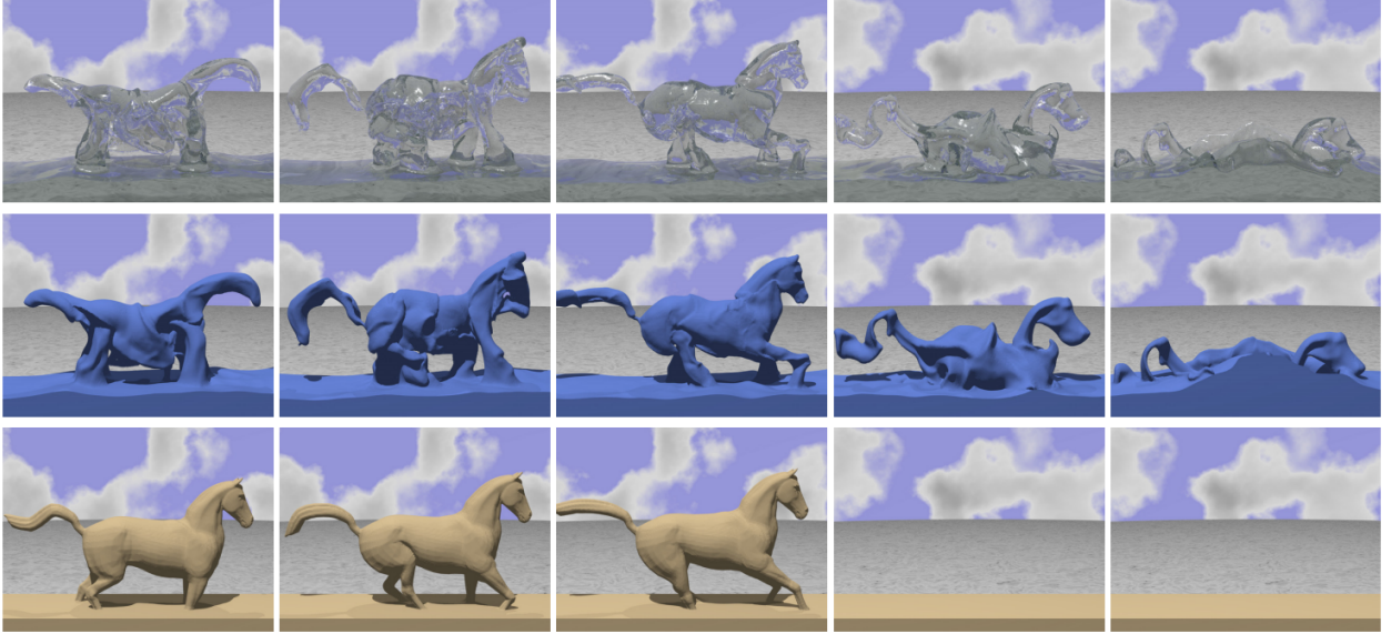
Fig. 2.2.8. A liquid is controlled using the method of Shi and Yu [112] to match an animated mesh representing a galloping horse. Top and middle row: Surface of the controlled liquid, rendered using respectively a water-like and a Lambertian shading. Bottom row: The animated target used to control the liquid simulation.
