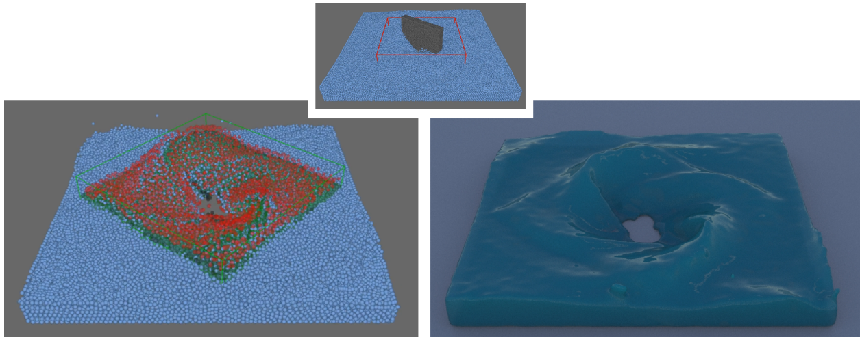
Fig. 3.5.7. 3D liquid controlled using a template describing a liquid mixed using a 3D rotating blade. Top: Recording a portion of a liquid mixed using a rotating blade. Left: Liquid simulation controlled using the resulting template. Right: Offline rendering of the resulting liquid surface.
