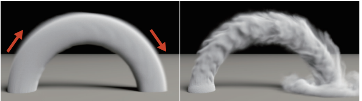
Fig. 2.5.4. Left: Density field advected by a procedurally-generated low-resolution flow field. Right: High-resolution simulation generated using the method of Sato et al. [99].
