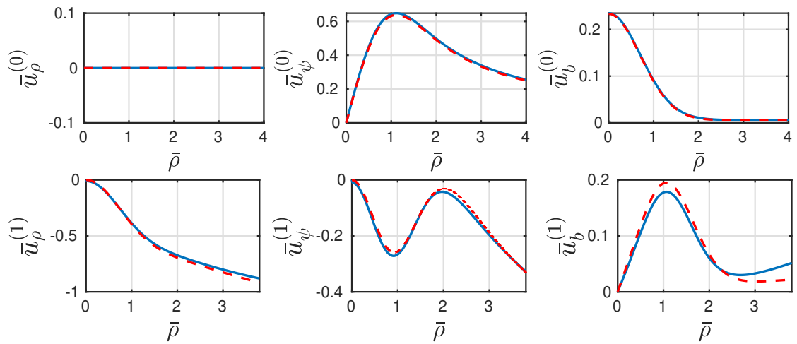
Figure 4.12 – Case BS1: radial distributions of velocity components ( \bar{u}_\rho^{(m)}, \bar{u}_\psi^{(m)}, \bar{u}_b^{(m)} ) for m = 0 (top) and m = 1 (bottom). Blue solid line: DNS results; red dashed line: theory.
