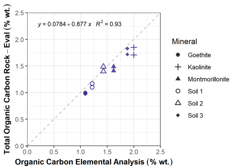
Figure 35: Performance of Rock-Eval® for detecting carbon (TOC+MinC) in simple dry mixtures compared to classic flush combustion elemental analysis. Points represent duplicate measurements. The equation represents the linear regression between x and y values.
