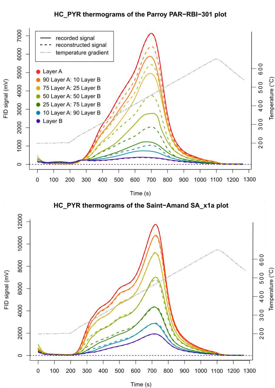
Supplementary Figure 2: Example of recorded and reconstructed HC_PYR thermograms of a plot with a heterogeneous clay content profile (Parroy) and a plot with little change of clay content with depth (Saint-Amand).
