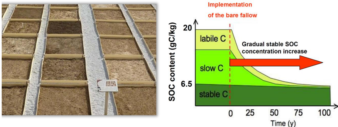
Figure 20: To the left: Picture from the Versailles long-term bare fallow experiment (©INRAE). To the right: Schematic representation of the evolution of the different SOC pools at an LTBF site ( Chenu, 2020 ).
