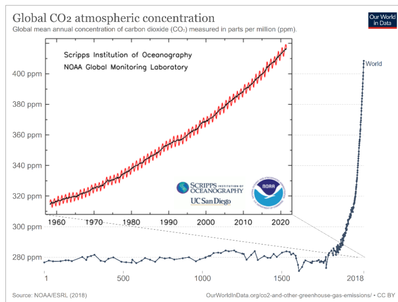
Figure 6: Atmospheric CO 2 concentration rise in the last two millennia. Values before 1958 are inferred from gases trapped in Antarctic ice cores (Bereiter et al., 2015). Data from 1959 onwards are direct measurements of atmospheric CO 2 concentration from the Mauna Loa observatory in Hawaii. Figure modified after sources mentioned on the figure.
