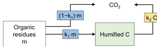
Figure 14: Conceptual representation of the simple two-compartment Hénin-Dupuis model. The model considers two organic matter compartments, organic residues ( m ) and humified organic carbon ( C ). Fluxes are expressed by arrows. Incorporation of fresh organic matter into soil is controlled by the humification coefficient k_1 and loss of humified carbon through mineralization is controlled by the mineralisation coefficient k_2 (modified after Mary and Guerif, 1994 ).
