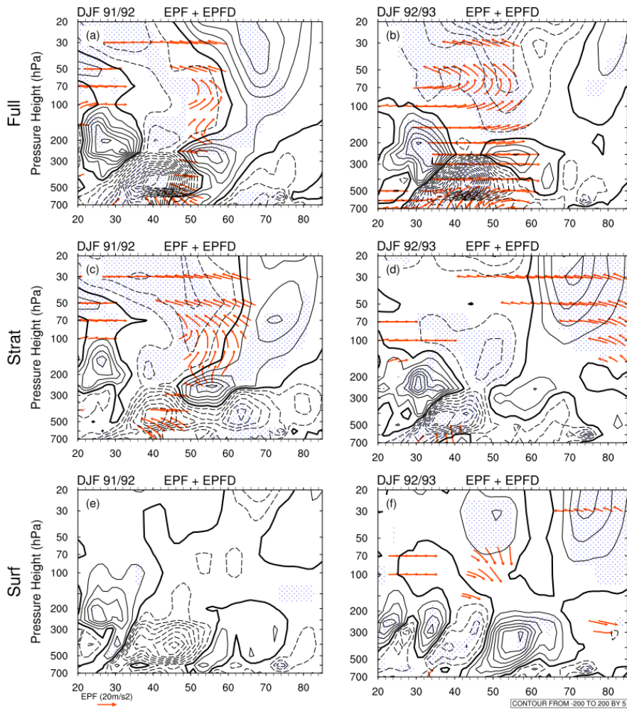
Figure 12: Latitude-Pressure Height cross sections of simulated EP flux anomalies and EP divergence anomalies in the first (left panel) and second (right) winter after 1991 Mt. Pinatubo eruption for a and b Full , c-d Strat , e-f Surf experiment. Only significant(90%) anomalies of the EP flux vectors are shown in arrows. Ensemble means of EP divergence are drawn with thin solid (positive) and dashed (negative) contours. Significant (90%) EP flux anomalies are stippled.
