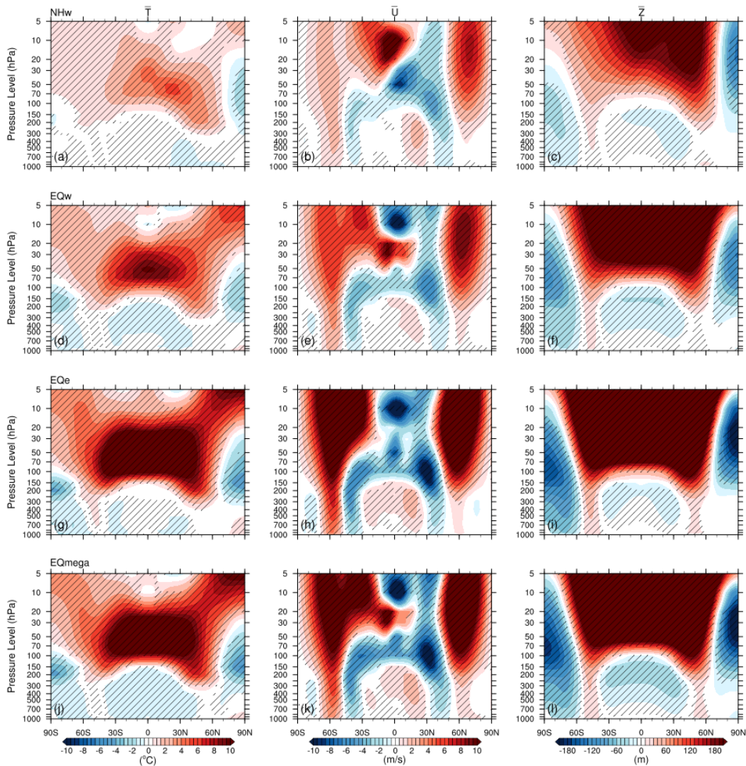
Figure 3.13: Same as Figure 5.11, but for the first winter anomalies of a-c: NHw, d-f: EQw, g-i: EQe and j-l: EQomega volcanic cluster.
