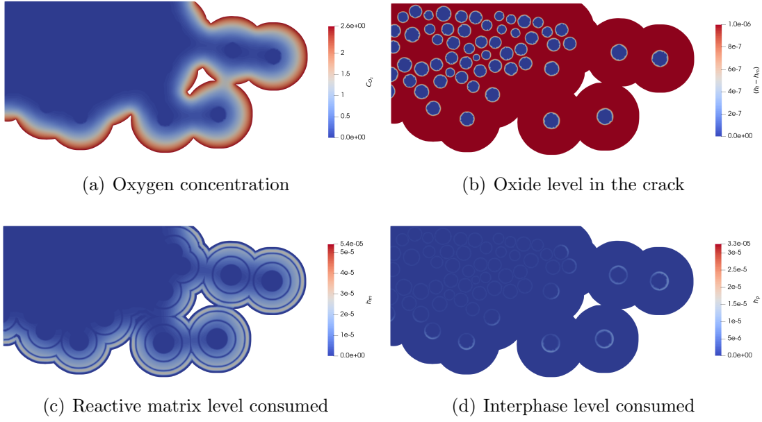
Figure 2.19: Two-dimensional self-healing simulation at t = 28 hr .
