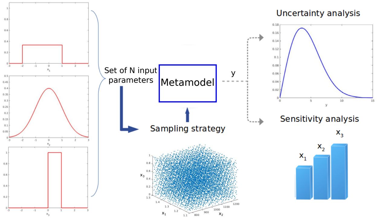
Figure 6.1: Uncertainty quantification on PCE-based metamodel strategy.
