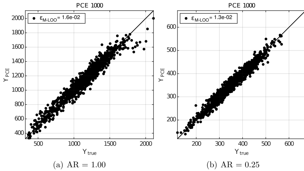
Figure 6.18: Failure time of the mini-composite computed via PCE metamodel built with 1000 points on the experimental design set w.r.t. the true response of the model for tow with AR = 1.00 and AR = 0.25 .
