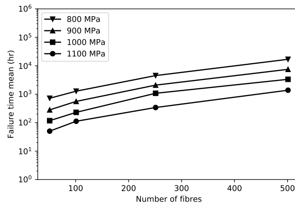
Figure 5.17: Failure time mean vs number of fibres for tow with AR = 1.00 subjected to different values of applied stress.
