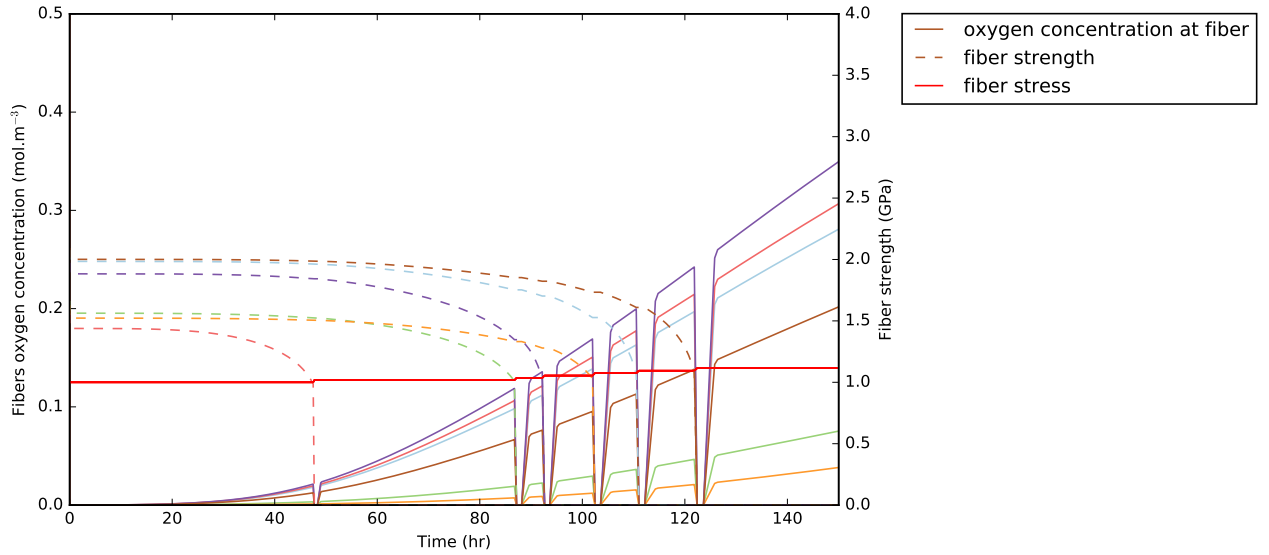
Figure 4.8: Time evolution of fibres' oxygen concentration, strength and applied stress for 4.4(b).
