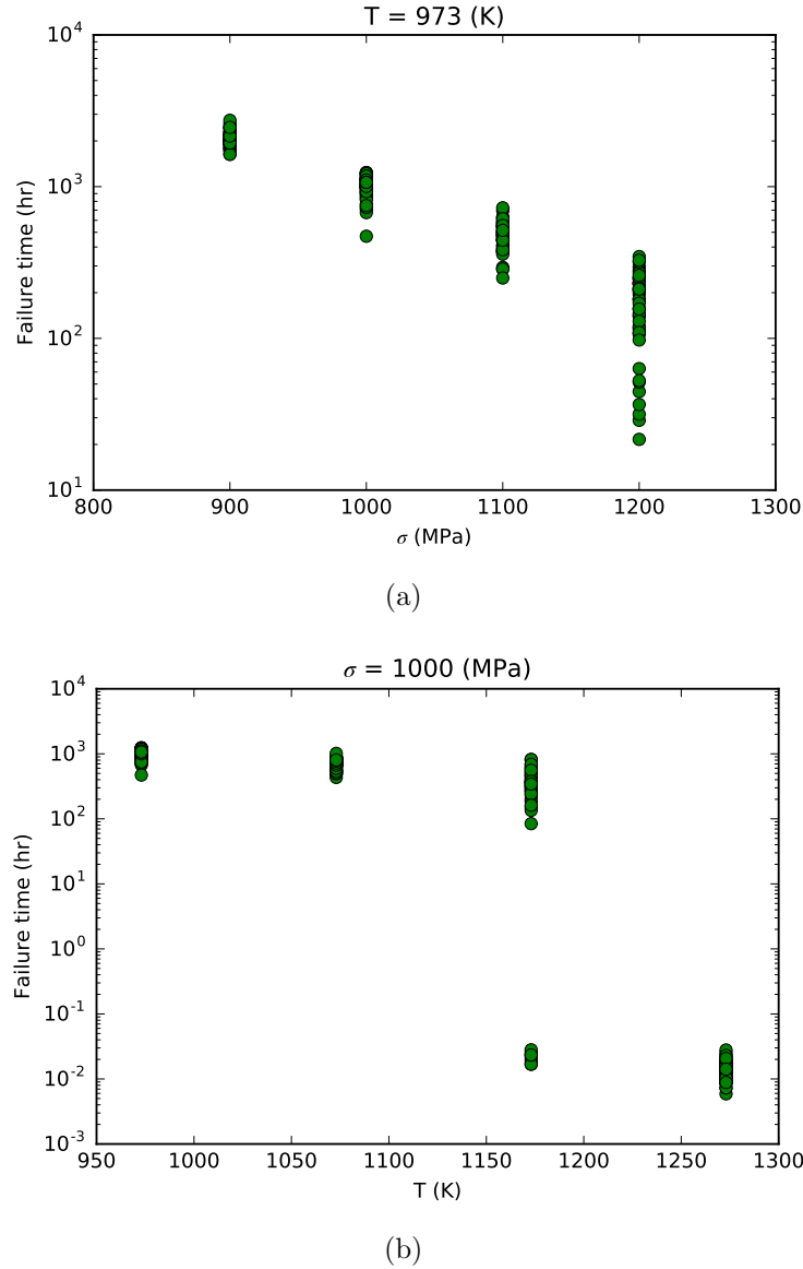
Figure 4.10: Mini-composite failure time for different load 4.10(a) and temperature 4.10(b) conditions.
