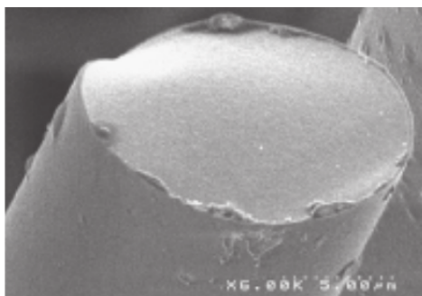
Figure 3.5: \text{SiO}_2 oxide layer on a Hi-Nicalon fibre [37].
