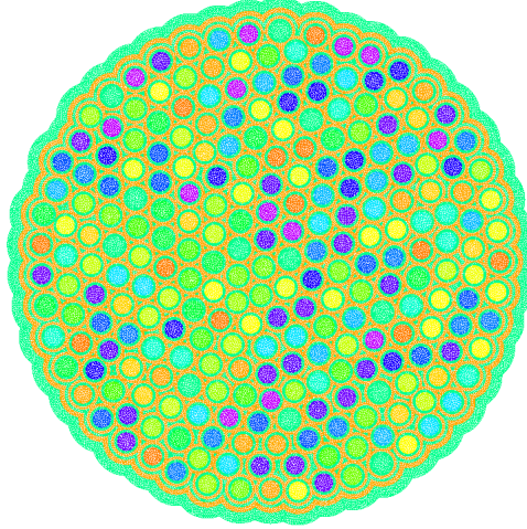
Figure 6.7: Considered tow for metamodal construction, consisting in 251 fibres with aspect ratio (AR) = 1.00.
