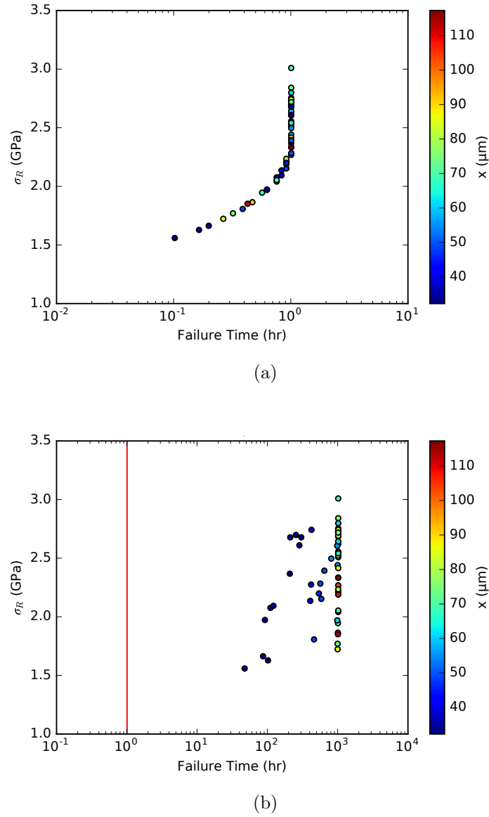
Figure 4.4: Fibres' failure history in function of their initial strength and distance from the outer boundary at T = 973 K and \sigma = 1 GPa without (4.4(a)) and with oxide (4.4(b)).
