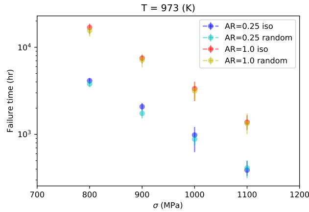
Figure 5.7: Failure time vs applied stress for tow with AR = 0.25 and AR = 1.00 constituted by 51 5.7(a), 251 5.7(b) and 501 5.7(c) fibres iso-distributed or randomly-distributed.
