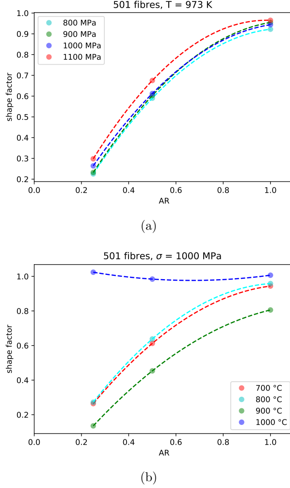
Figure 5.22: Shape factor vs. aspect ratio (AR) under different stress and temperature conditions (reference tow 501 fibres).
