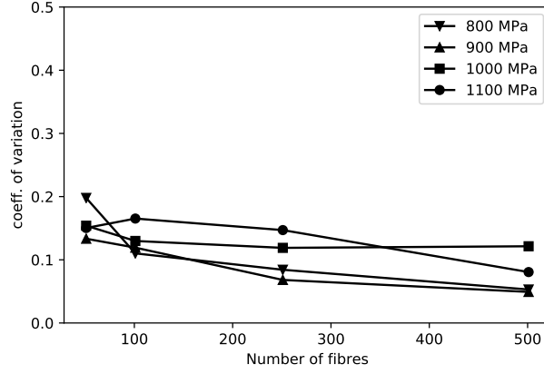
Figure 5.18: Failure time coefficient of variation vs number of fibres for tow with AR = 1.00 subjected to a different values of applied stress.
