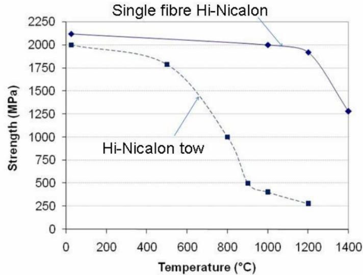
Figure 4.1: Temperature-strength diagram for tows and Hi-Nicalon single filament [58].
