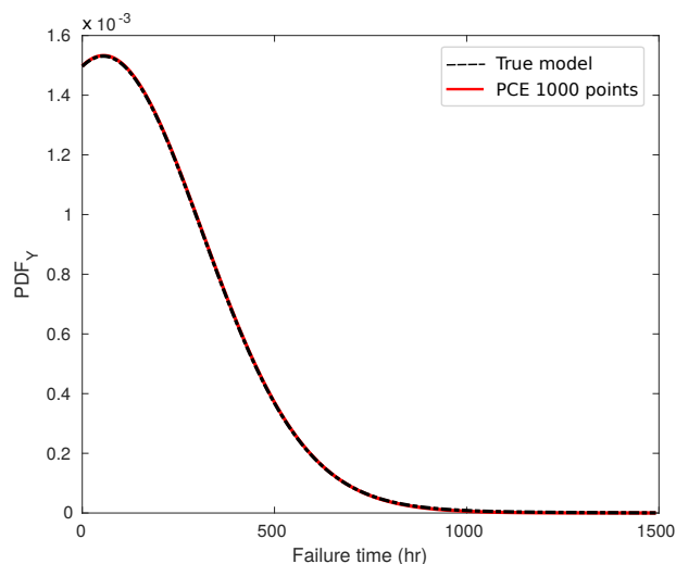
Figure 6.10: Probability density functions (PDFs) of the mini-composite failure time on validation set (1000 points) computed via PCE metamodel built with 1000 points w.r.t. the true PDF of the model.
