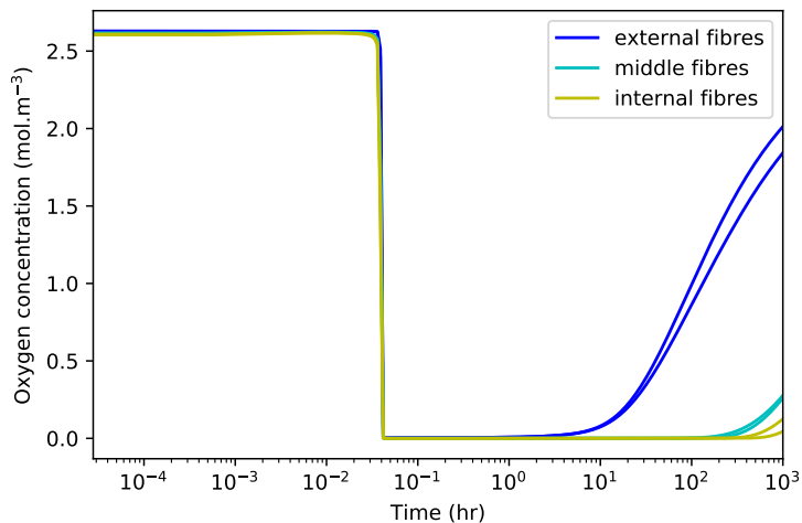
Figure 4.5: Oxygen concentration at the surface of fibres vs. time for \sigma = 1 GPa and T = 973 K.
