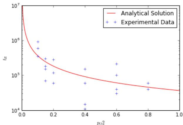
Figure 3.12: Hi-Nicalon fibre tow lifetime as a function of oxygen partial pressure at T = 773 K and \sigma = 1000 MPa.
