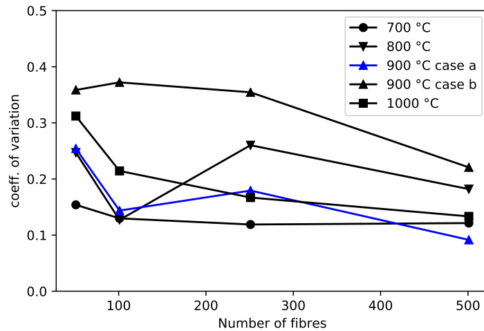
Figure 5.21: Failure time coefficient of variation vs number of fibres for tow with AR = 1.00 at different temperatures.
