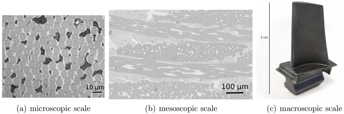
Figure 1.3: Different scales for CMCs.
