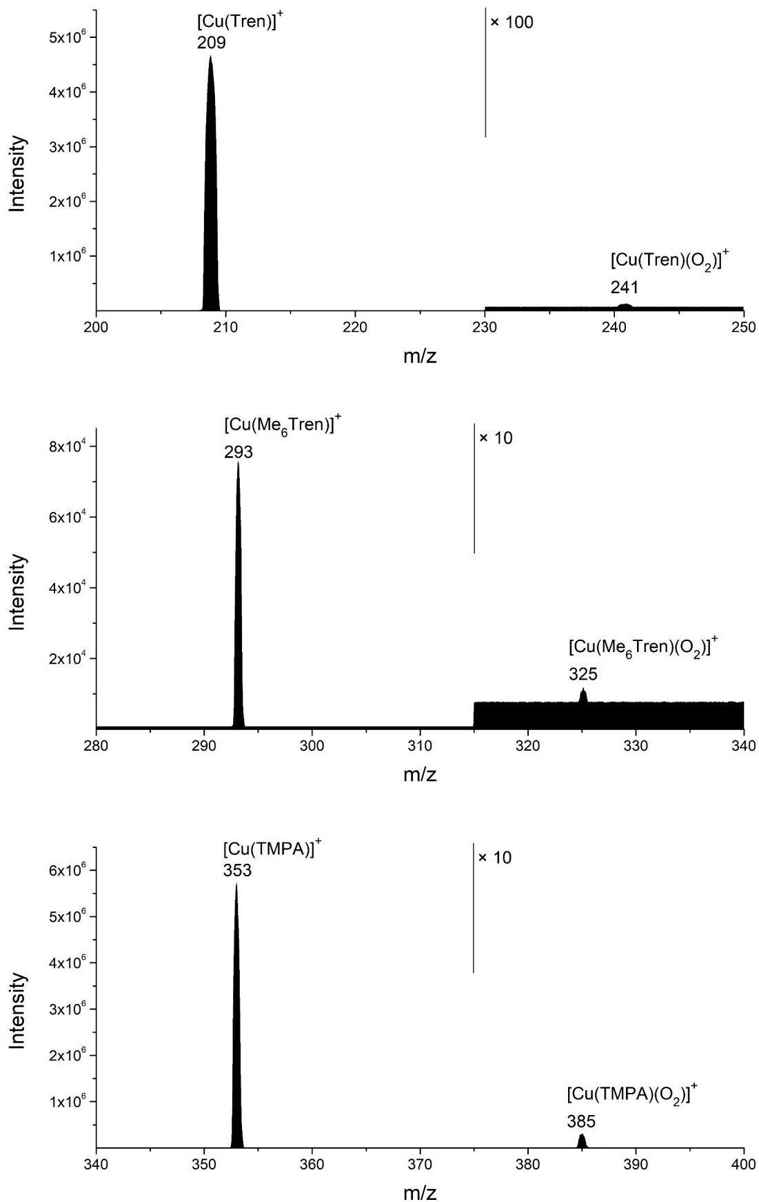
Figure 10: CAR-MSMS spectra of [Cu(Tren)] + (top), [Cu(Me 6 Tren)] + (middle) and [Cu(TMPA)] + (bottom), with O 2 as collision gas ( P = 6.5 \cdot 10^{-3} mbar, V_{coll} = 3 V).
