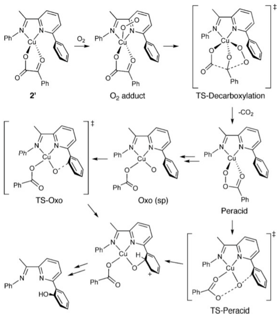
Figure 22: Postulated mechanism for the selective hydroxylation of phenyl group. Reprinted with permission from [102]. Copyright 2007 American Chemical Society.
