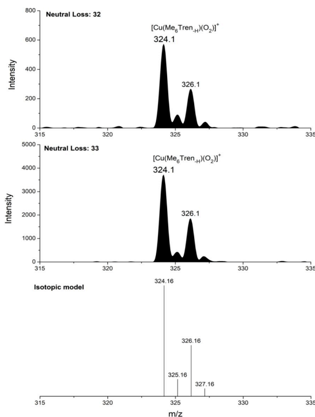
Figure 16: Neutral loss spectra with P(O_2) = 5 \cdot 10^{-5} mbar in H0 and P(Ar) = 1.2 \cdot 10^{-3} mbar in collision cell (H2). Sample: [Cu(Me_6Tren-H)(O_2)]^+(H_2O)(ClO_4)_2 5 \cdot 10^{-5} M in CH_3CN/H_2O 4:1.
