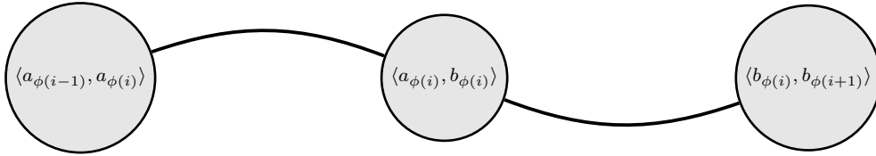
Figure 50: Neighborhood relationship of \phi(i) = \langle a_{\phi(i)}, b_{\phi(i)} \rangle , \phi(i-1) = \langle a_{\phi(i-1)}, a_{\phi(i)} \rangle and \phi(i+1) = \langle b_{\phi(i)}, b_{\phi(i+1)} \rangle .
