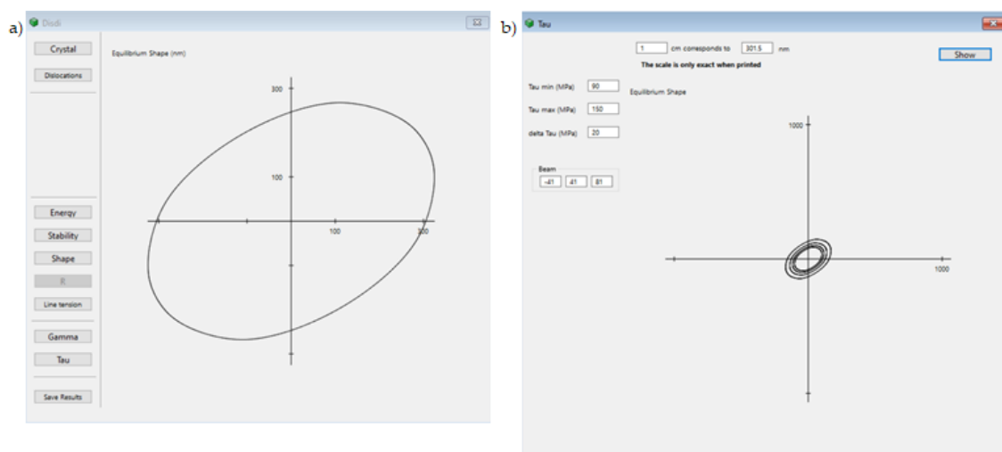
Figure 3-4 – DISDI screen capture of: a) shape of the dislocation loop in equilibrium, b) proposed CRSS values for the dislocation “P” ( \tau_{min} = 90, \tau_{max} = 150, \text{step} = 20 ). The scales on the axis are in nm.
