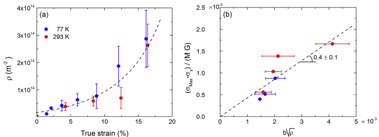
Figure 1-21 – a) Dislocation density \rho as a function of true strain. b) Taylor hardening plot showing linear dependence of the normalized work hardening (\sigma_{Max} - \sigma_y) / (M \cdot G) as a function of (b \cdot \rho^{1/2}) . From [60].
