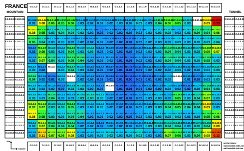
Figure 3.27 – Top : Time offset values per OM of the French Main Wall w.r.t OM 396. Bottom : to the left the final offset error values per OM of the French Main Wall w.r.t OM 396, on the right a 1 dimensional distribution of the error on time offset values. All in [ns].
