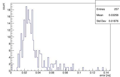
Figure 3.27 – Top : Time offset values per OM of the French Main Wall w.r.t OM 396. Bottom : to the left the final offset error values per OM of the French Main Wall w.r.t OM 396, on the right a 1 dimensional distribution of the error on time offset values. All in [ns].
