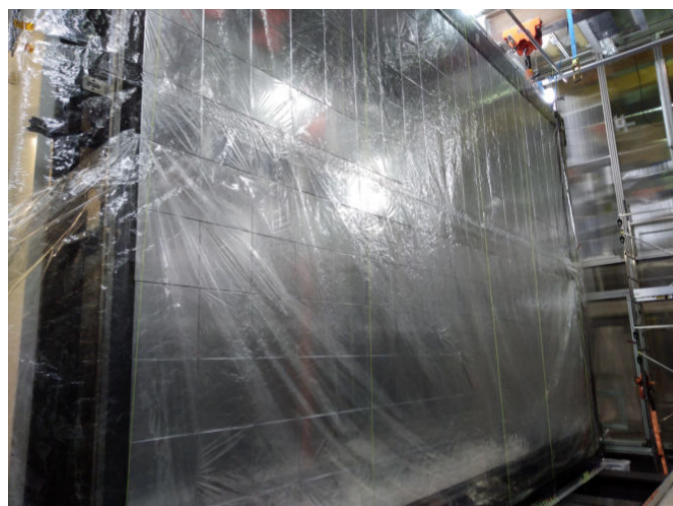
Figure 2.17 – A calorimeter wall covered with radio-pure nylon film. To avoid Radon diffusion from the calorimeter towards the tracker gas
