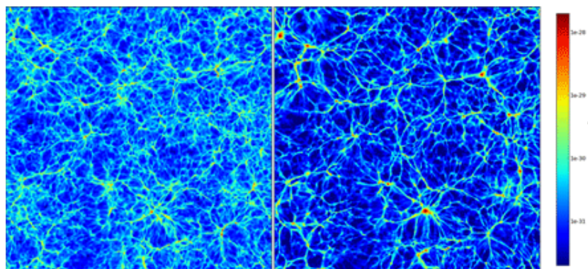
Figure 1.7 – Density distribution in the universe : To the left : With massive neutrinos ( m_\nu = 1.9 \text{ eV} ) and to the right : With massless neutrinos ( m_\nu = 0 \text{ eV} ). The maps are produced through numerical simulations, the colors represent the density of ordinary (baryonic) matter [12].
