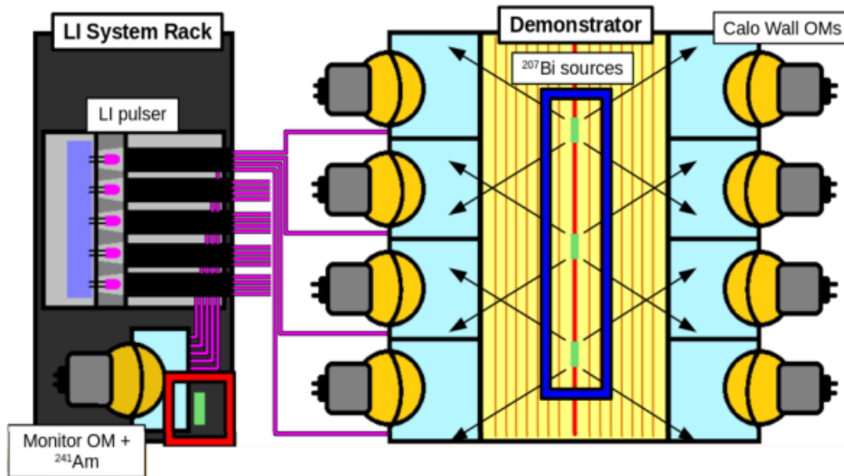
Figure 2.23 – the Light injection system setup. Inside the rack is shown the reference OM with the ^{241}\text{Am} source. Optical fibers (shown in purple) are connected between the LEDs (pink dots) and each OM.
