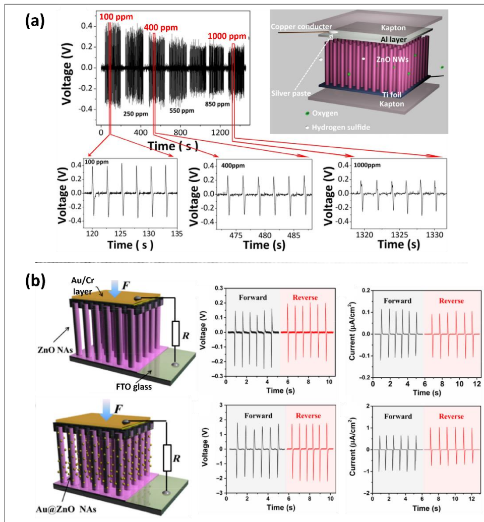
Figure 11. (Image taken from [46], [65]). (a) Schematic diagram of the ZnO NWs-based PZ for gas sensing applications. The voltage generated by the NWs decreases with increasing the concentration of adsorbed gas in ppm. The depletion thickness decreases and screening becomes effective leading to the decreased piezo-response of NWs. (b) The presence of Au nanoparticles on the surface of ZnO NW-based PZ suppresses the screening. The voltage and the current generated by the PZ thus increases (bottom) as compared to the ZnO NWs without Au particles (top).
