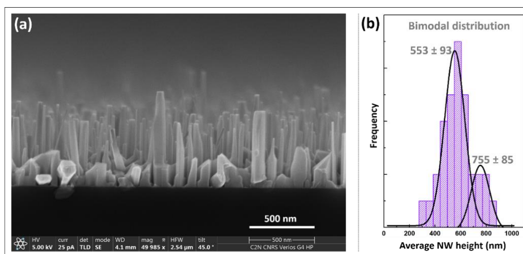
Figure 24. (a) SEM image of the intrinsically p-doped GaN NWs in the cross-section view. (b) Histogram showing the bimodal distribution of the NW heights with respective Gaussian fittings.
