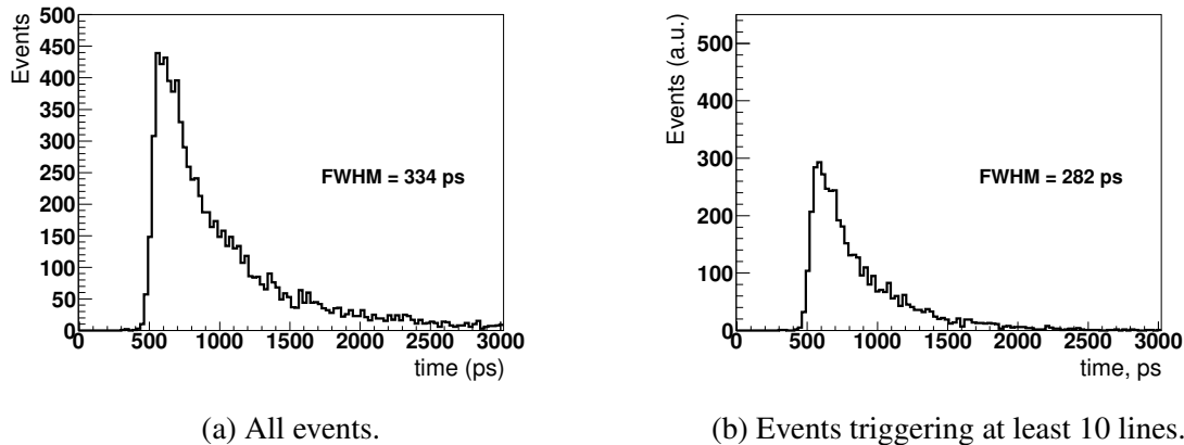
Figure 5.34: Simulated CM prototype time resolution.
