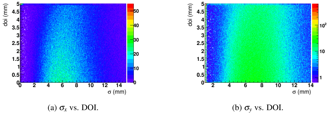
Figure 4.3: Correlation \sigma_x , \sigma_y and DOI in the CM prototype.
