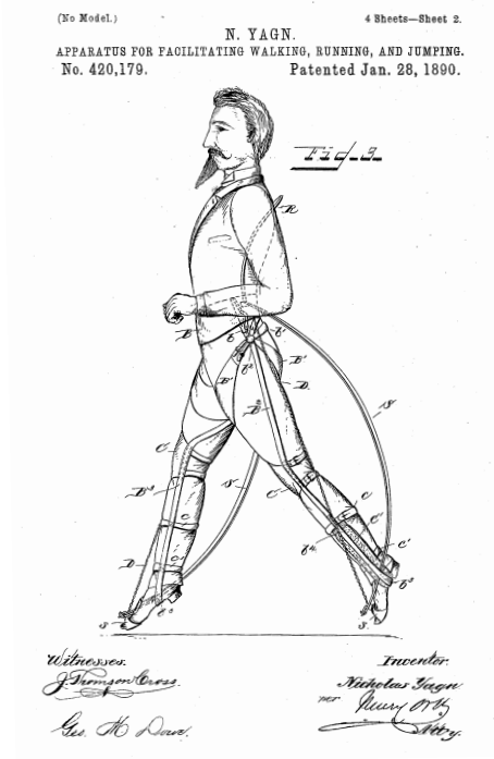
FIGURE 1.1: Drawings from Nicholas Yagn's patents of multiple devices for facilitating walking, running, and jumping (Yagn 1889, 1890a-c).
