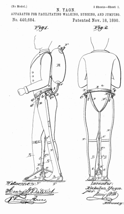
FIGURE 1.1: Drawings from Nicholas Yagn's patents of multiple devices for facilitating walking, running, and jumping (Yagn 1889, 1890a-c).
