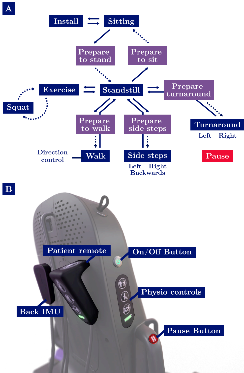
FIGURE 2.3: A. Finite State Machine of the Atalante exoskeleton. Purple boxes represent preparatory transition states. Solid blue lines represent button-enabled transitions. Dotted blue lines represent IMU-enabled transitions. Specific modes of a generic state (for example, left turnaround) are written under the corresponding boxes. Direction control is a button-enabled alteration of the Walk state. The Pause state (in red) is button-enabled, and can be accessed from any other state. B. Hardware control inputs of the Atalante exoskeleton. The patient is equipped with a remote controller, and a back IMU for transition confirmation. Additional buttons are available on the robot for the physiotherapist.
