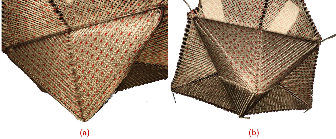
Figure 3.17: Final configuration of tetrahedral forming
