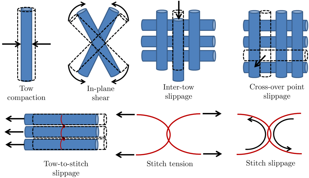
Figure 1.9: Deformation modes of conventional textiles (Reproduced from Creech and Pickett (2006) )
