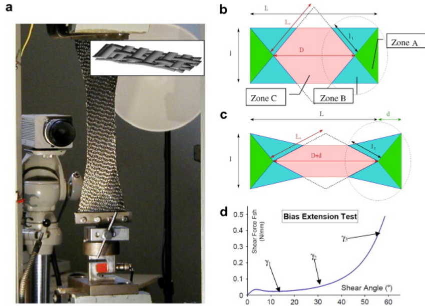
Figure 1.18: Bias extension test: (a) the device (inset: weave structure of the fabric G1151) (b) initial rectangular specimen with yarns oriented at \pm 45^\circ (c) deformed specimen (d) shear load curve for G1151 interlock fabric (Lomov et al., 2008)
