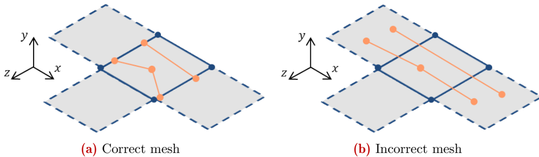
Figure 2.23: Meshing of 1D embedded elements in 2D host elements
