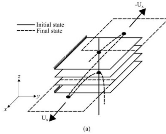
Figure 4.61: Proposed models based on mixed embedded-ALE elements: (a) Simplification of the tufting Model I and (b) tufting Model II
