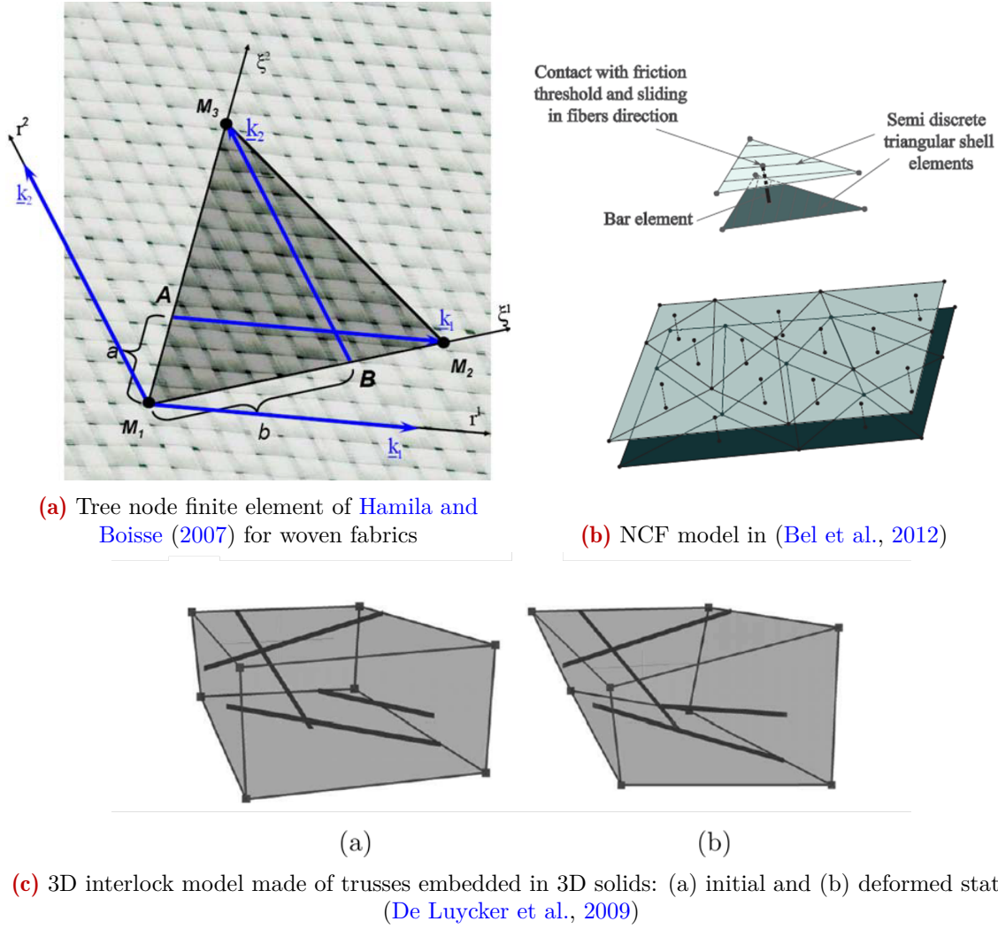
Figure 1.15: Discrete models' examples
