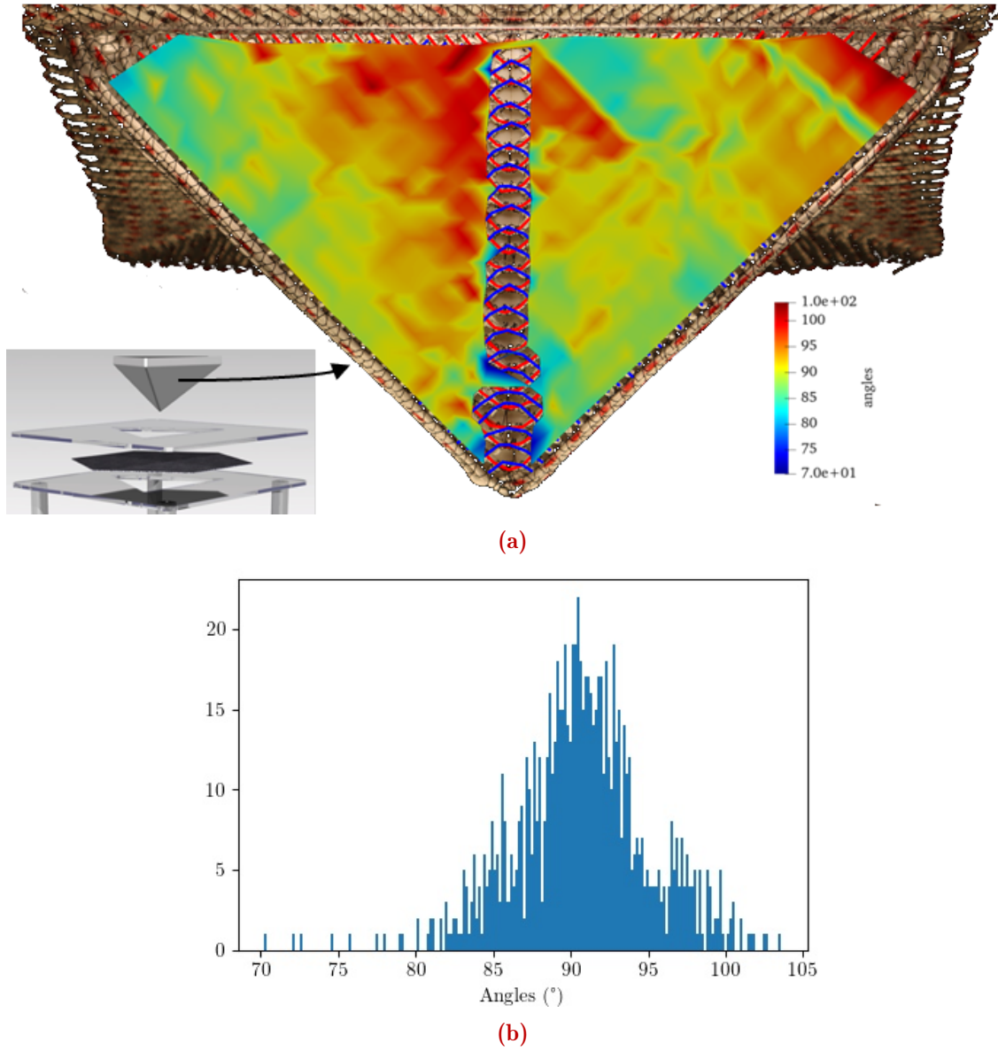
Figure 3.18: Angles between layers: (a) mesh build from triangulation of intersection points displaying the angles and (b) distribution of the angles
