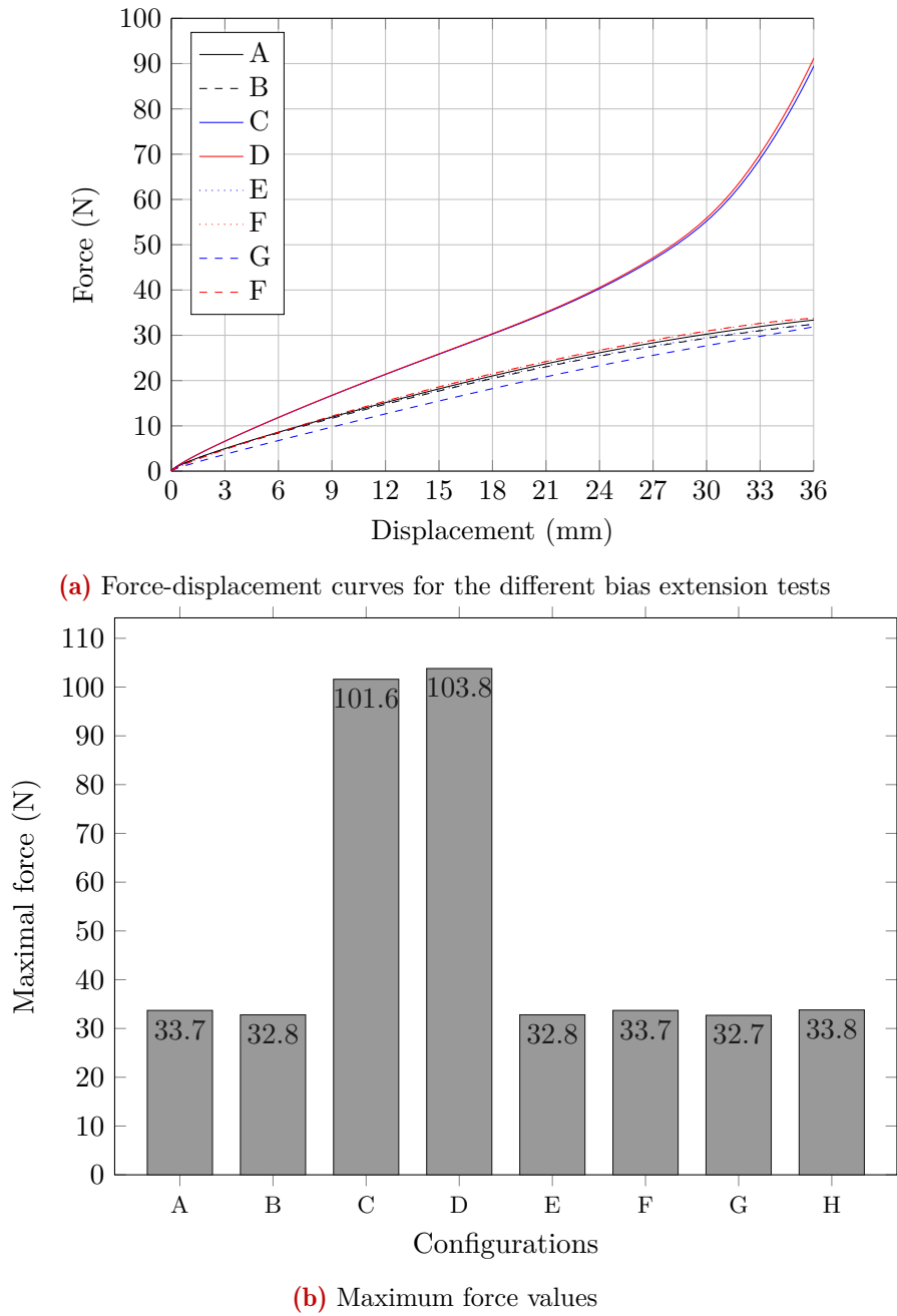
Figure 4.54: Result of the bias extension test with and without reinforcing fibre tows
