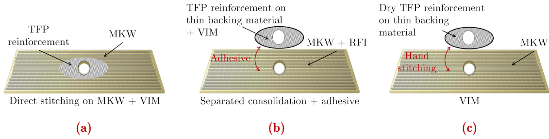
Figure 1.36: Different strategies to assemble conventional textile and TFP reinforcements (Crothers et al., 1997)
