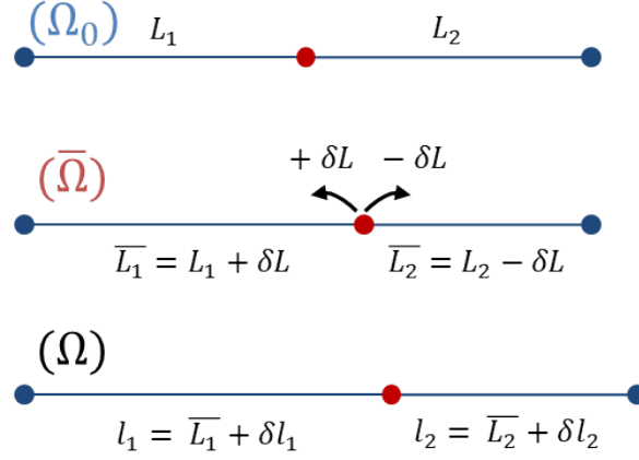
Figure 4.12: Configurations of the multi-sliding nodes model with one sliding node
