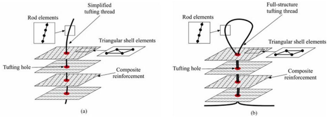
Figure 4.60: (a) Simplified model of the tufting (Model I) and (b) full-structure model of the tufting (Model II) (Huang et al., 2021)
