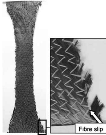
Figure 1.10: Tow slippage in bias extension test of NCF (Creech and Pickett, 2006)
