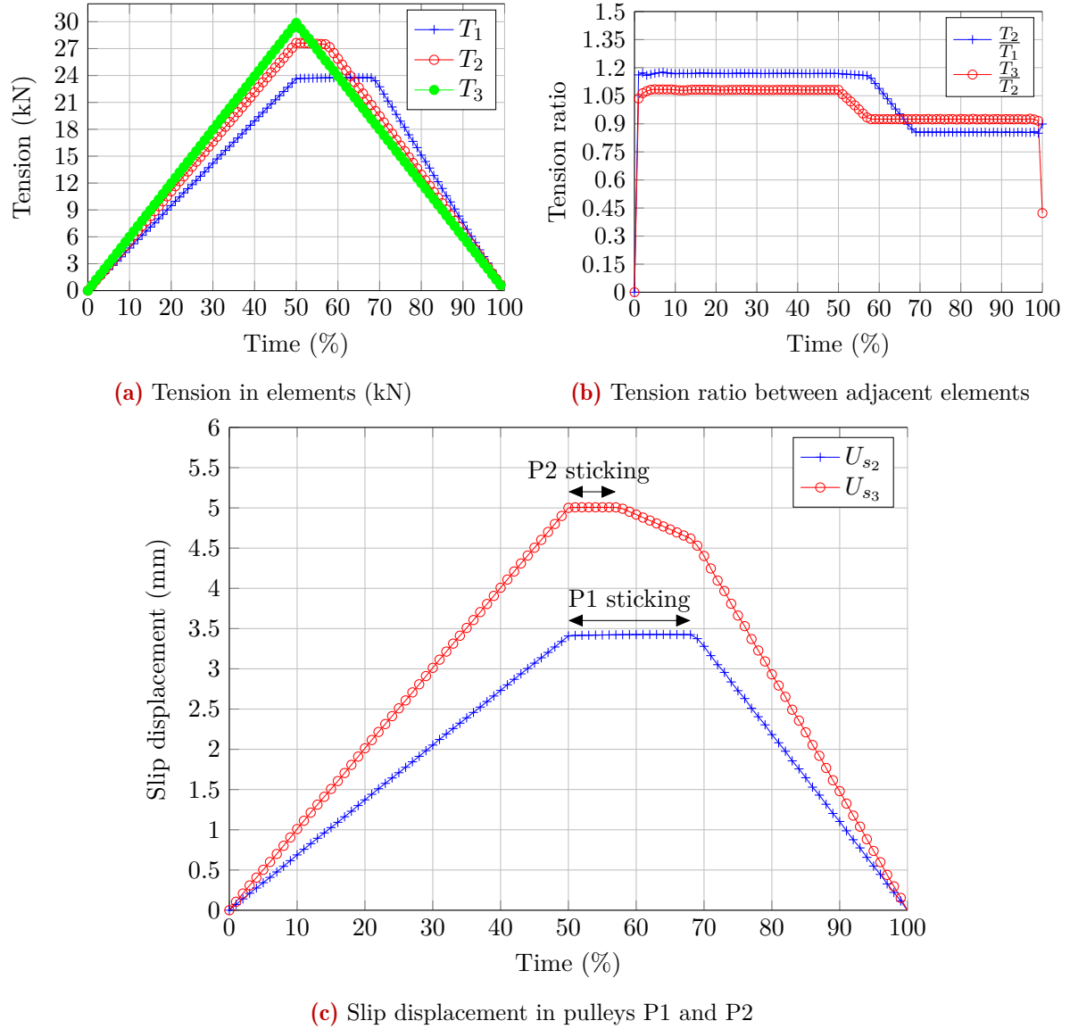
Figure 4.23: Cable with two fixed pulleys
