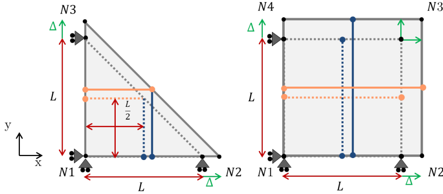
Figure 2.27: Biaxial tension of an incompressible NeoHookean membrane reinforced with 2 orthogonal beam elements (initial configuration (dotted line), final configuration (solid line))
