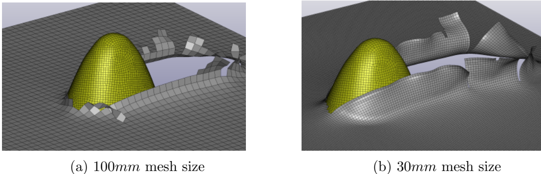
Figure 2.9: Observed deformation of bottom plating depending on mesh size
