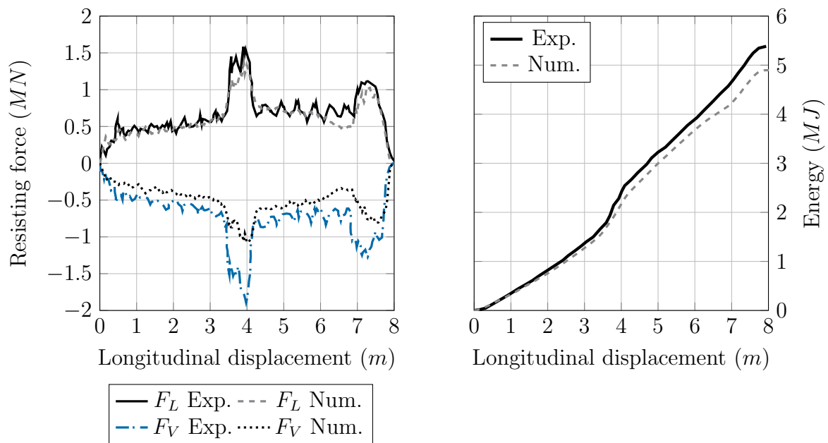
Figure 3.9: NSWC grounding test : comparison of resistant forces (left) and dissipated energy (right)
