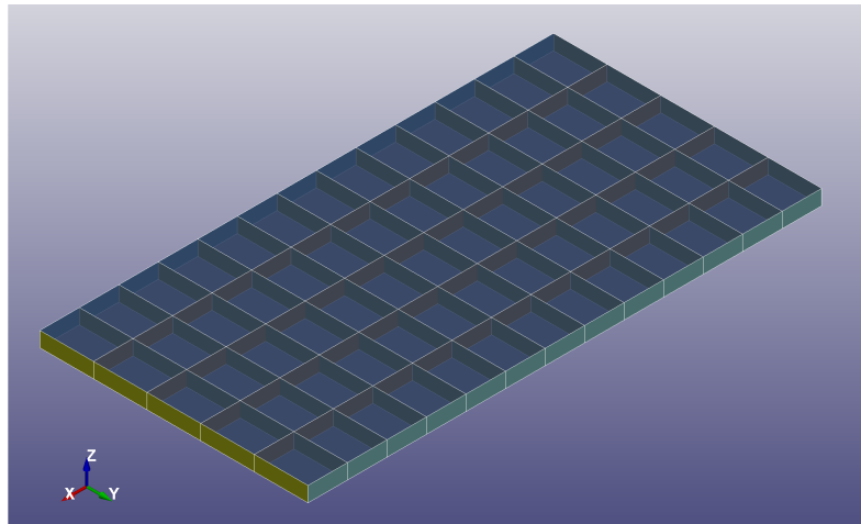
Figure 7.20: Ship bottom model - Combined grounding analysis
