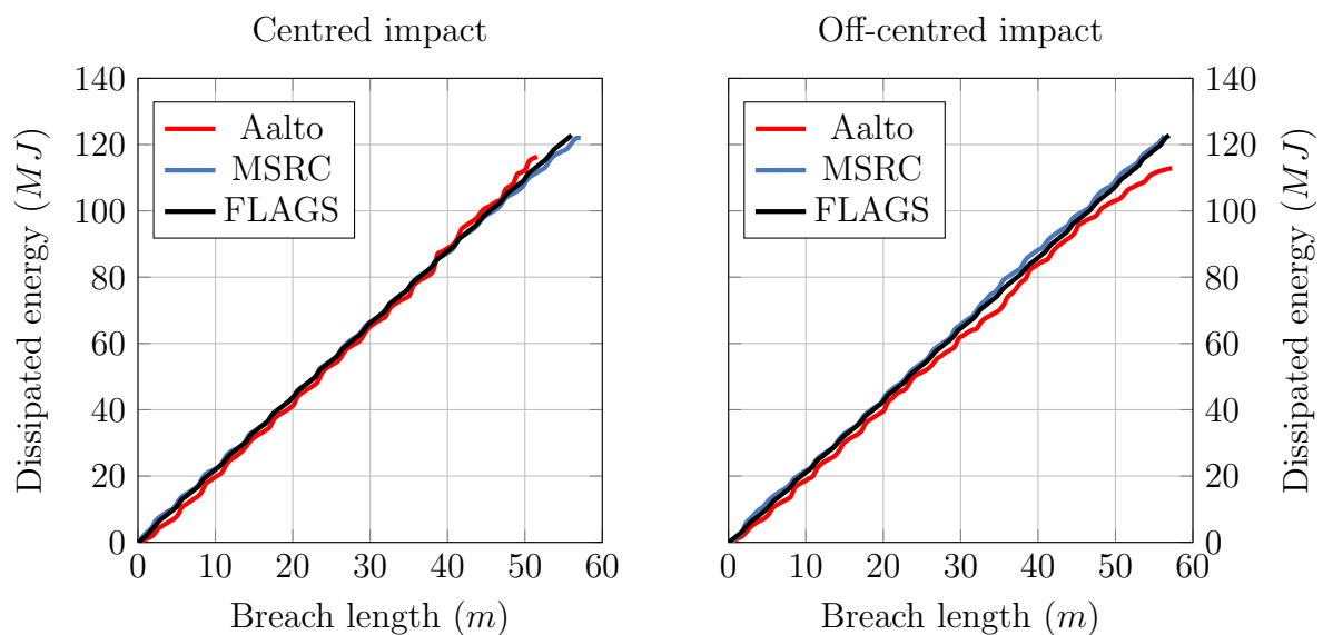
Figure 7.7: Dissipated energy versus breach length
