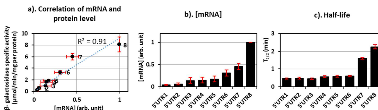
Figure 5. Concentration and stability of the lacZ mRNA of the 8 selected constructs and level of the corresponding \beta -galactosidase protein. a) Correlation of \beta -galactosidase activity and lacZ mRNA concentration. Numbers 1-8 represent the constructs with 5'UTR 1 to 8, respectively. lacZ mRNA concentration is expressed as fold change compared to the reference strain 5'UTR8. The blue dashed line represents the linear regression curve and the coefficient of determination is indicated ( R^2=0.91 ); b) lacZ mRNA concentration as fold change compared to the reference strain 5'UTR8; c) Half-life of lacZ mRNA in min for the 8 constructs. For all, error bars represent standard deviation (n= 3).
