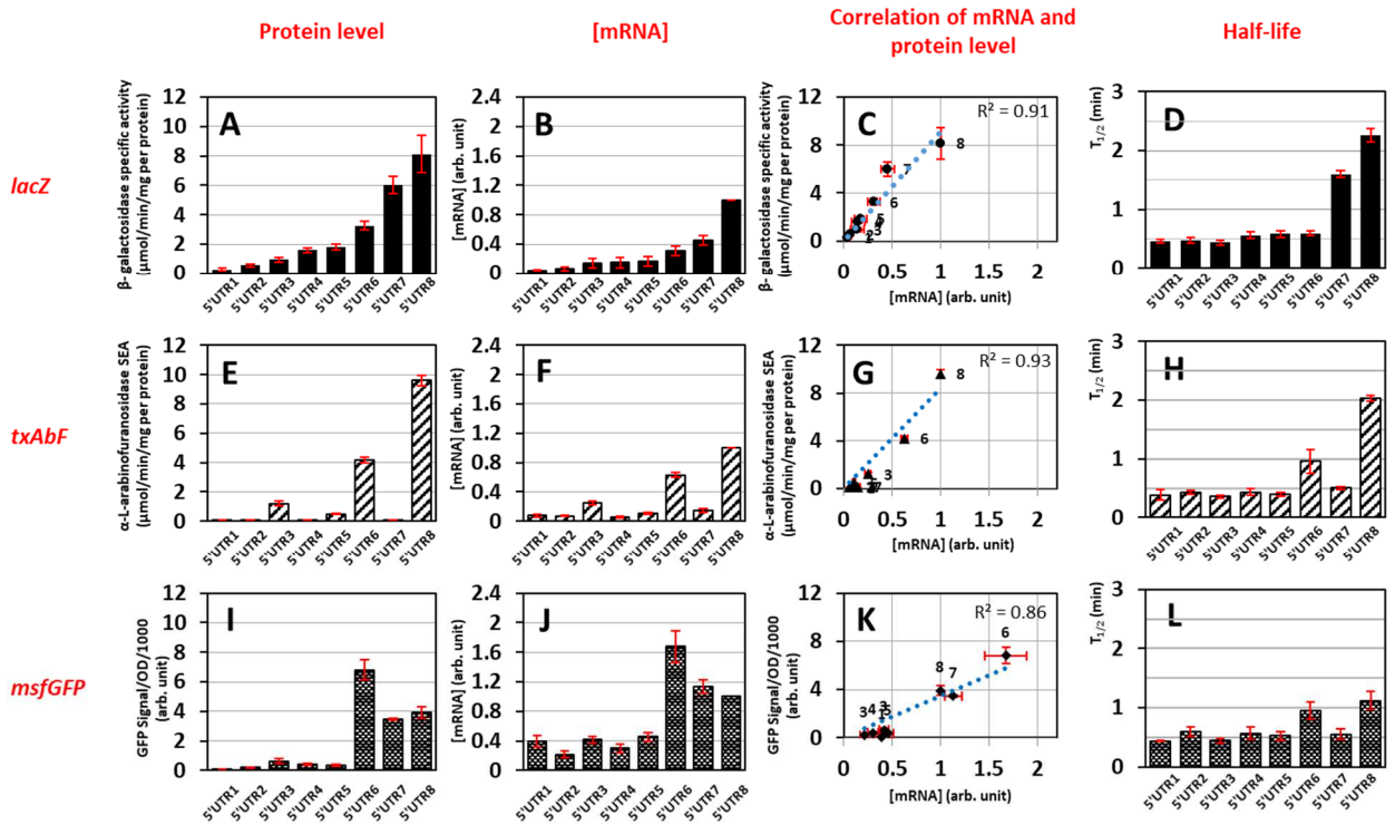
Figure 6. Protein levels and mRNA concentration of the constructs with 8 different 5'UTRs and 3 different reporters ( lacZ , txAbF and msfGFP ). For Fig 6A, B, C and D related to lacZ , the values are those shown previously in Fig 5A, B and C. A) Specific \beta -galactosidase activity. B) lacZ mRNA concentration as a fold change relative to 5'UTR8- lacZ . C) Correlation between lacZ mRNA concentration and \beta -galactosidase activity. D) lacZ mRNA half-life. E) Specific \alpha -L-arabinofuranosidase activity. F) txAbF mRNA concentration as a fold change relative to 5'UTR8- txAbF . G) Correlation between txAbF mRNA concentration and \alpha -L-arabinofuranosidase activity. H) txAbF mRNA half-life. I) msfGFP fluorescence/OD. J) msfGFP mRNA concentration as a fold change relative to 5'UTR8- msfGFP . K) Correlation between msfGFP mRNA concentration and GFP fluorescence/OD. L) msfGFP mRNA half-life. For C, G, K, the blue dashed line represents the linear regression and the coefficient of determination ( R^2 ) is indicated on the graph. For all, error bars represent standard deviation: n=3 for mRNA concentration and half-life determinations, n=9 (biological triplicates and technical triplicates) for \beta -galactosidase, TxAbF and GFP activity.
