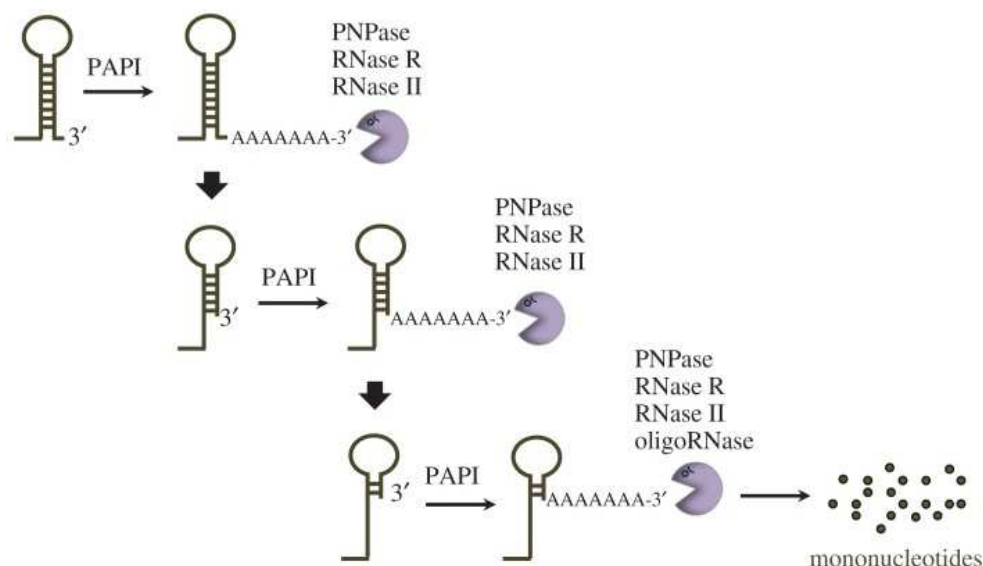
Figure 10. The PAP I-dependent degradation of structured RNAs in E. coli (Hajnsdorf & Kaberdin, 2018). Stable stem-loop structures at the 3' end of transcripts are resistant to the action of major exoribonucleases, but their degradation can be facilitated by polyadenylation. Repeated cycles of polyadenylation and subsequent 3' → 5' degradation of the polyadenylated species by exoribonucleases and the oligoribonuclease (oligoRNase) yield mononucleotides.
