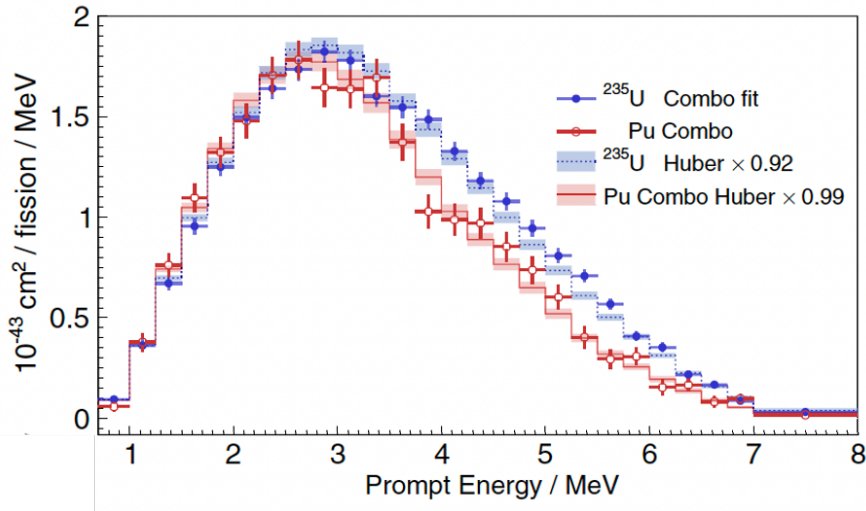
Figure 7.12: Comparison of the extracted ^{235}\text{U} and Pu combo spectra with the corresponding Huber-Mueller predicted spectra, with the normalization factors 0.92 and 0.99. One must add that the Pu combo spectrum, is normalized to the number of ^{239}\text{Pu} fissions. The event excess in the 4-6 MeV region are clearly visible for both spectra. Source [152].
