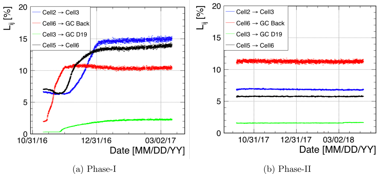
Figure 3.15: Evolution of some light leaks coefficients during Phase-I (a) and Phase-II (b) data-taking periods. Source [73].
