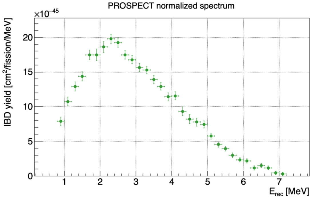
Figure 7.6: PROSPECT measured 235 U spectrum, normalized to STEREO data set.
