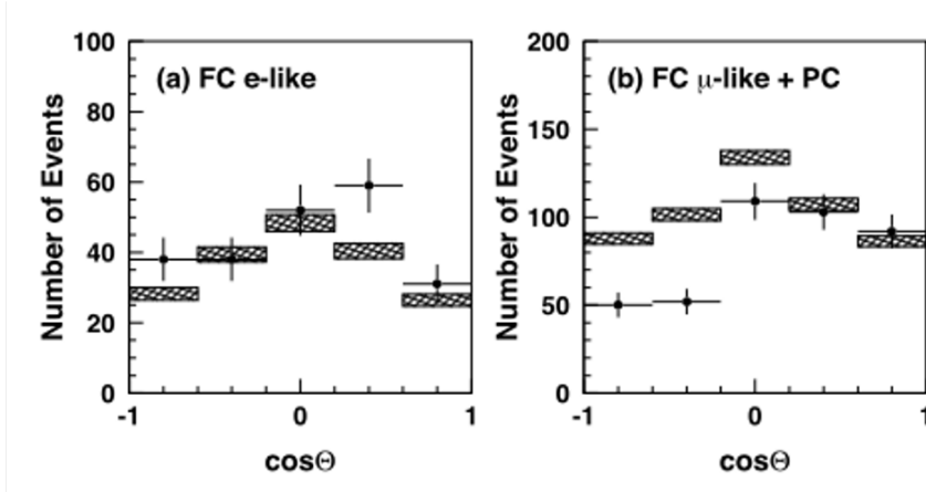
Figure 1.2: Zenith angle distribution for multi-GeV full-contained (FC) and partially-contained (PC) events , from the first 414 days of Super-Kamiokande data. Partially-contained events have a neutrino interaction in the fiducial volume with a final state particle exiting into the outer detector. The muon and electron final state particles that proceed from the CC neutrino interaction in the detector respectively refer to \nu_\mu and \nu_e events. The markers represent the events counted by Super-Kamiokande, the boxes represent the expected event counts. For upward-going neutrinos coming from the opposite side of Earth (negative values of \cos\Theta ), a deficit of \mu -events is clearly visible. Source [30].
