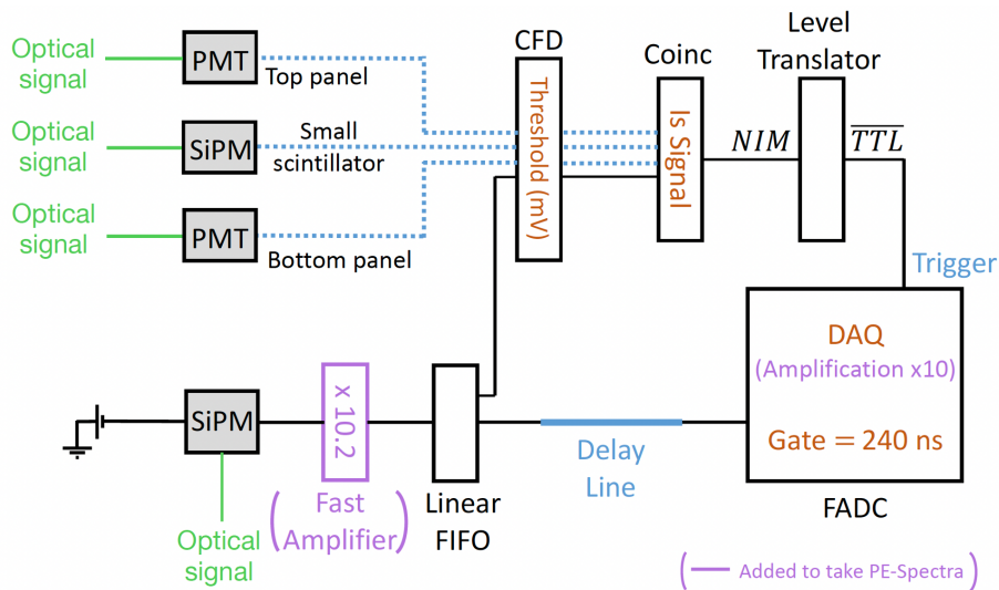
Figure 9.3: DAQ scheme. The prototype SiPM signals are processed by an FADC. The external trigger is generated by a constant fraction discriminator (CFD), a coincidence module (Coinc) and a level translator. By demanding a coincidence of the prototype SiPM signal(s) with the top and bottom PMT signals, or the SiPM signal of the small plastic scintillator, different muon samples can be selected. Optionally, for calibration measurements, the SiPM signals can be amplified by a fast amplifier and a FADC-internal amplification.
