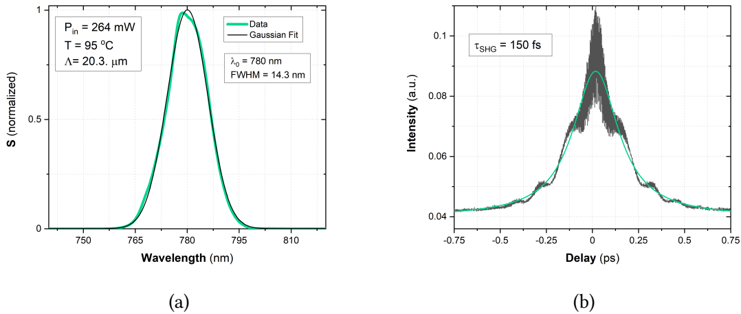
Figure 7.3: Conversion SHG Crystal. (a) Second harmonic Spectrum with a gaussian fit. (b) Autocorrelation signal of the second harmonic, giving a pulse duration of 150 fs.
