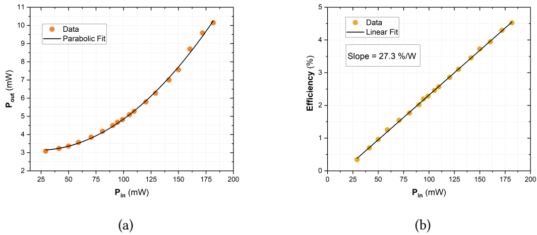
Figure 7.2: Conversion SHG Crystal. (a) Second harmonic power vs input telecom power. (b) Corresponding SHG efficiency.
