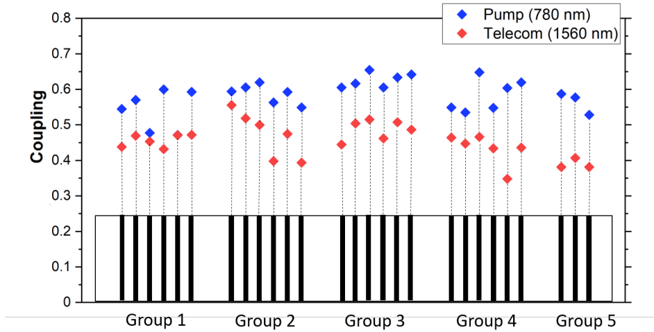
Figure 7.8: Coupling efficiency at pump and seed wavelengths for every waveguide measured along the chip. In all cases the polarization was set to vertical.
