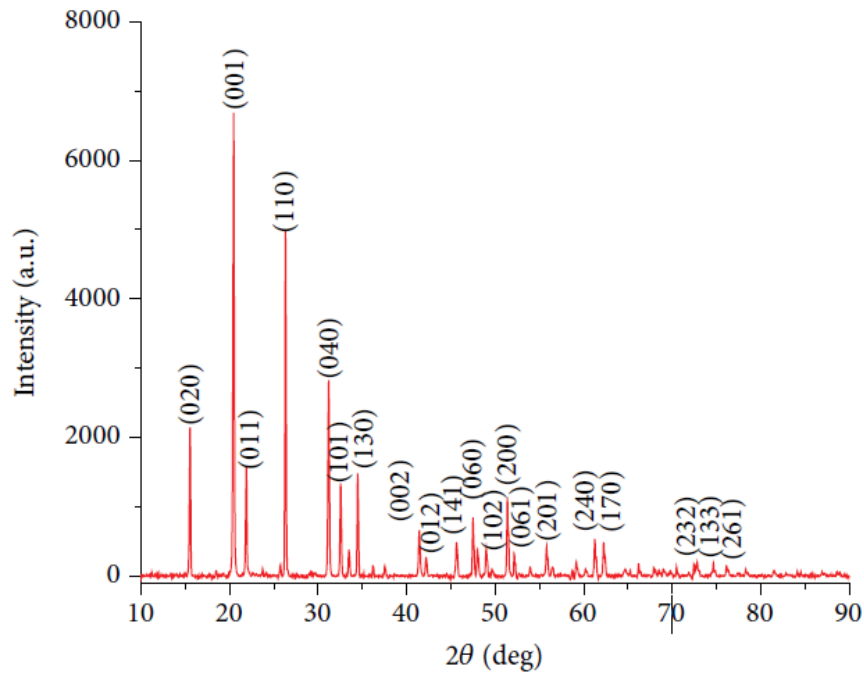
Figure 9 XRD Pattern of V_2O_5 nanoparticles.
