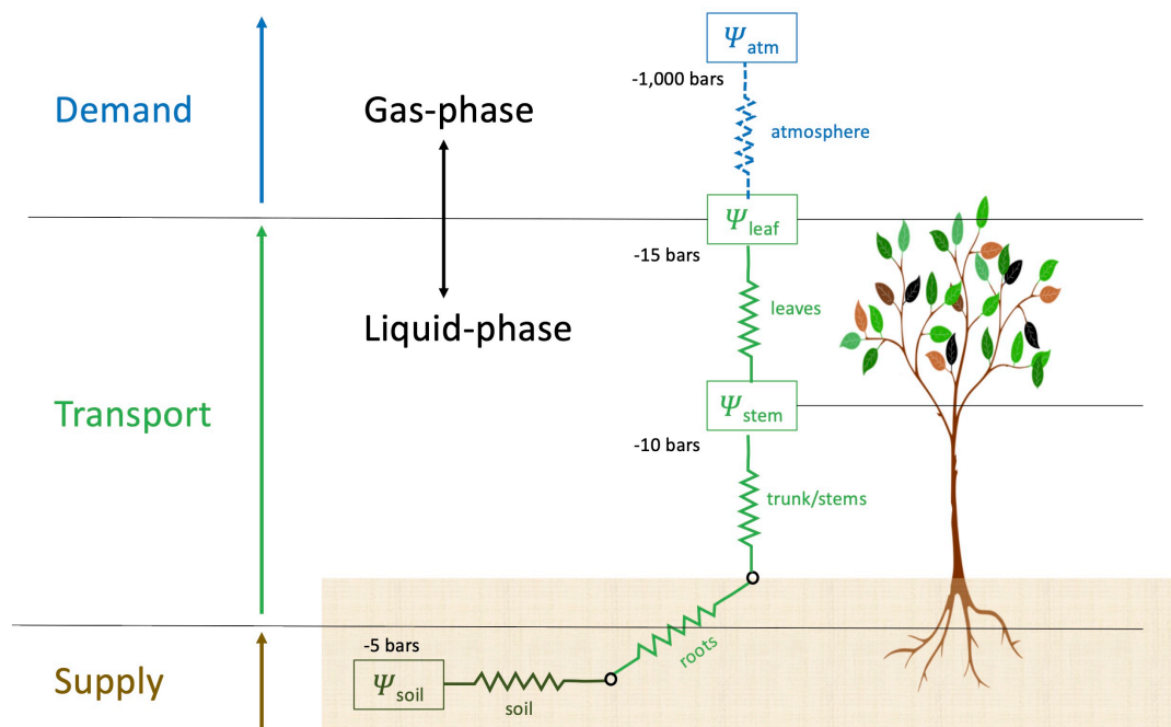
Figure 1. Schematic depiction of the soil-plant-atmosphere continuum, showing gradients of water potential across different elements of the supply, transport and atmospheric demand for water, and the boundary between gas and liquid phases.
