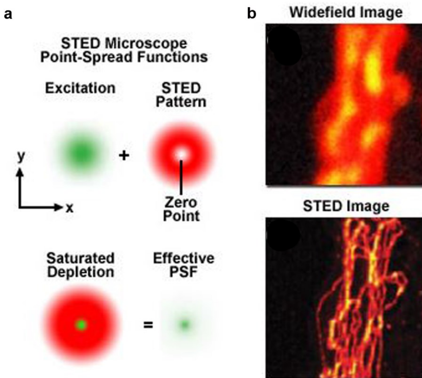
Figure 40: Principle of STED nanoscopy
