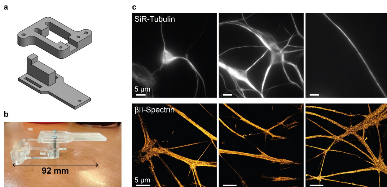
Figure 41: New PMMA-based stretching device enables long-term culture of primary hippocampal neurons until DIV 8
