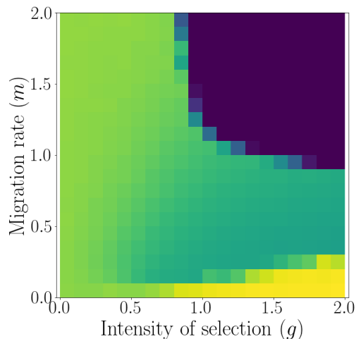
(b) IBS outcomes - 500 loci.
