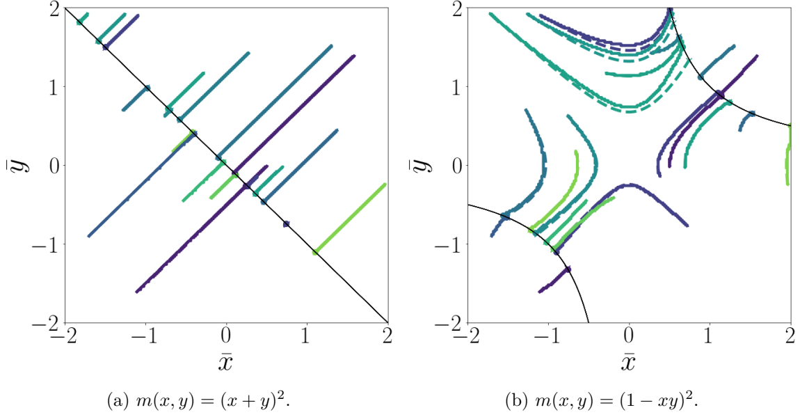
Figure 1.8: Comparison between the trajectories of the dominant alleles (\bar{x}(t), \bar{y}(t)) in a monomorphic population obtained from numerical recursions of (P(n_\epsilon)) (full lines) and the canonical equations (dashed lines), with two different selection functions. In each subfigure, each colored line corresponds to a trajectory departing from a uniformly randomly chosen monomorphic initial state (the set of initial states is the same between both figures). The black curve shows the region of steady states for each selection function: the diagonal x + y = 0 for Fig. 1.8a and the hyperbola xy = 1 for Fig. 1.8b. These two figures highlight the importance of a model and an analysis that can apply for various selection functions, as trajectories and steady states can be radically different from one particular to another.
