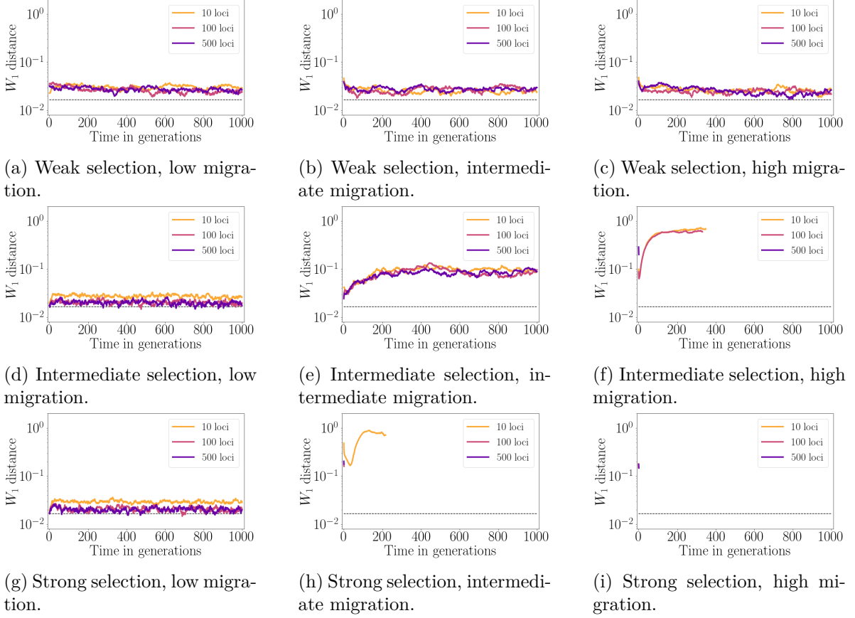
Figure 3.3: Dynamics of the W_1 distance between the distributions of the IBS replicates according to (3.8) and the solutions of the deterministic discrete-time model (3.2), for 3 increasing levels of selection (rows, top to bottom 0.1, 1, 2) and 3 increasing levels of migration (columns, left to right 0.05, 0.8, 1.4), with a large standard deviation at linkage equilibrium \sigma_{LE} = 1 (large variance case). For each figure, the three colors correspond to three different number of loci L = \{10, 100, 500\} (darker colors for larger number of alleles). The coloured lines represent the median distance across replicates (interrupted lines means that extinction occurred). The black dashed line represents the distance between two Dirac masses on consecutive points of the trait space's grid Z . Other parameter values for the deterministic models are: r = 1, \kappa = 1, \Delta t = 0.1 and those for the IBS as indicated in Section 3.3. Here, the number of loci does not influence the proximity of the deterministic model with the IBS (at least above 10 loci). The agreement between the deterministic model and the IBS is strong (coloured lines at the level of the black dashed line, which is the minimum distance between two Dirac masses on the discretization grid) when either selection is weak (top row) or migration is low (left column), and a bit worse when both selection and migration are intermediate (Fig. 3.3e). Extinction occurs in all other cases, when migration and selection are both sufficiently high (Fig. 3.3f, Fig. 3.3h, Fig. 3.3i).
