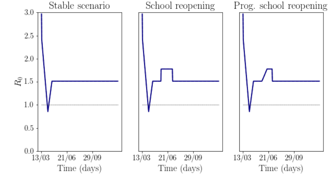
(a) Temporal dynamics of the basic reproduction number \mathcal{R}_0(t) .
