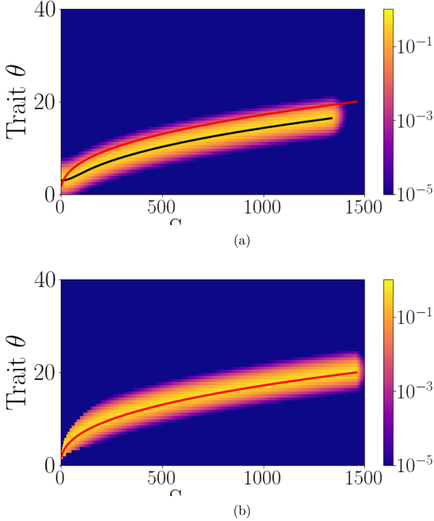
Figure 5.2: Heatmap of the trait distribution of a sexual population , associated to the Eq. (5.4) with parameters \delta t = 0.02 , \delta x = 4 , \delta \theta = 2/3 , x_{\max} = 3000 and \theta_{\max} = 201 . (a) Trait distribution given by the numerical simulations, at t = 200 . The red line represents the approximation of the mean trait behind the propagating front given by (5.7), and is common to both subfigures, while the black line is the mean trait behind the propagating front given by the simulations. (b) Trait distribution behind the propagating front given by Conjecture 1, at t = 200 .
