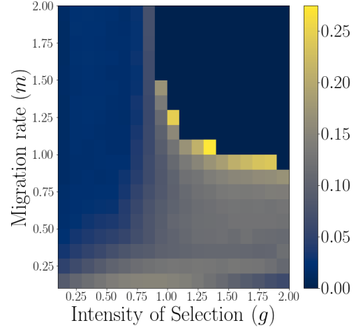
(b) Time constancy of the segregational variance throughout the IBS, for 500 loci, according to (3.11).
