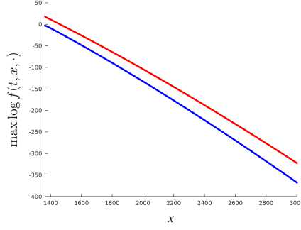
Figure 5.4: Plot of logarithm of the amplitude of the distribution ahead of the front at time t = 200 . The blue curve represents the log of the maximum of the distribution f(t, x, \cdot) of the numerical approximation given by the scheme, for different positions x located beyond the numerical value of the front position ( X^{\text{num}}(200) \approx 1400 ). The red curve represents the prefactor of the trait distribution ahead of the front given by Conjecture 1. The parameters are \delta t = 0.02 , \delta x = 4 , \delta \theta = 2/3 , x_{\text{max}} = 3000 and \theta_{\text{max}} = 201 .
