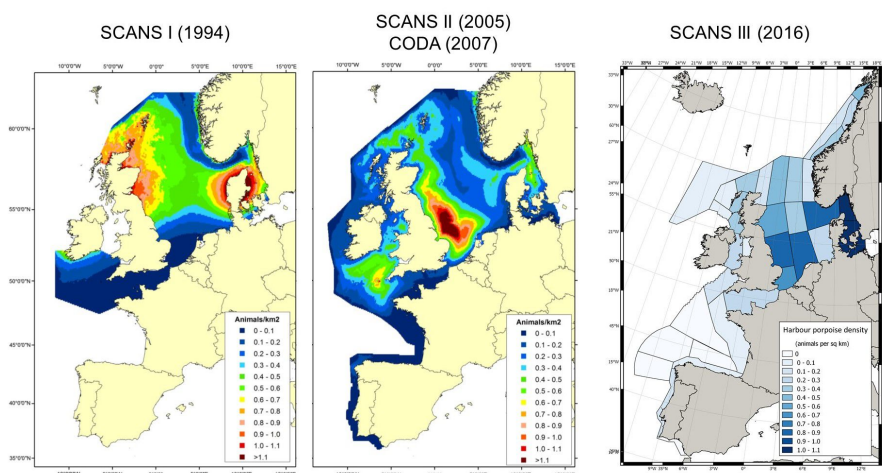
Figure 7.8: Density of Harbour porpoise estimated from the SCANS and CODA campaigns. The time period under consideration ranges from 1994 to 2016 with 3 main estimates. The density of harbour porpoises in the North-East Atlantic appears to have possibly changed over the period. The population now seems to be denser in the Western Channel, Celtic seas and Bay of Biscay than before.
