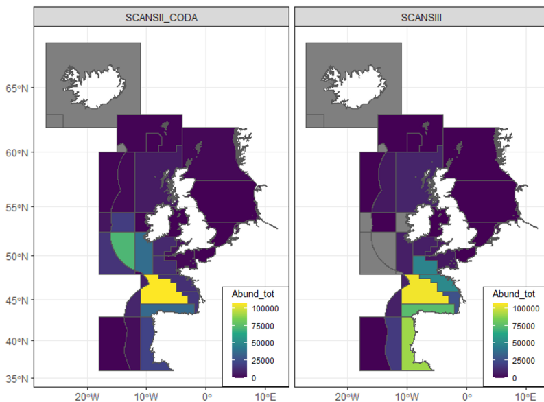
Figure 7.9: Abundance estimates of common dolphin by ICES divisions. The abundance estimates seem to be slightly higher for SCANS III than for SCANS II + CODA. Estimates from Hammond et al. (2017).
