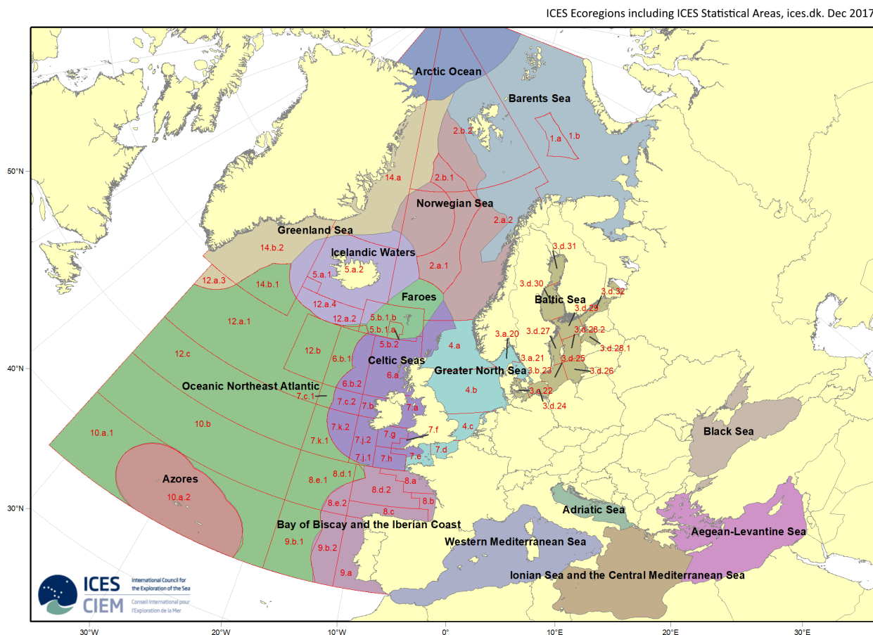
Figure 2.11: Ecoregions and statistical areas defined by ICES within the OSPAR area of the North-East Atlantic. The OSPAR area is divided by ICES into several ecoregions defined on the basis of biogeographic and oceanographic features and existing political, social, economic, and management divisions. Another division is made by taking into account statistical areas. These areas are linked to ICES fishing areas developed from historical links between an area and the collection of fisheries statistics.
