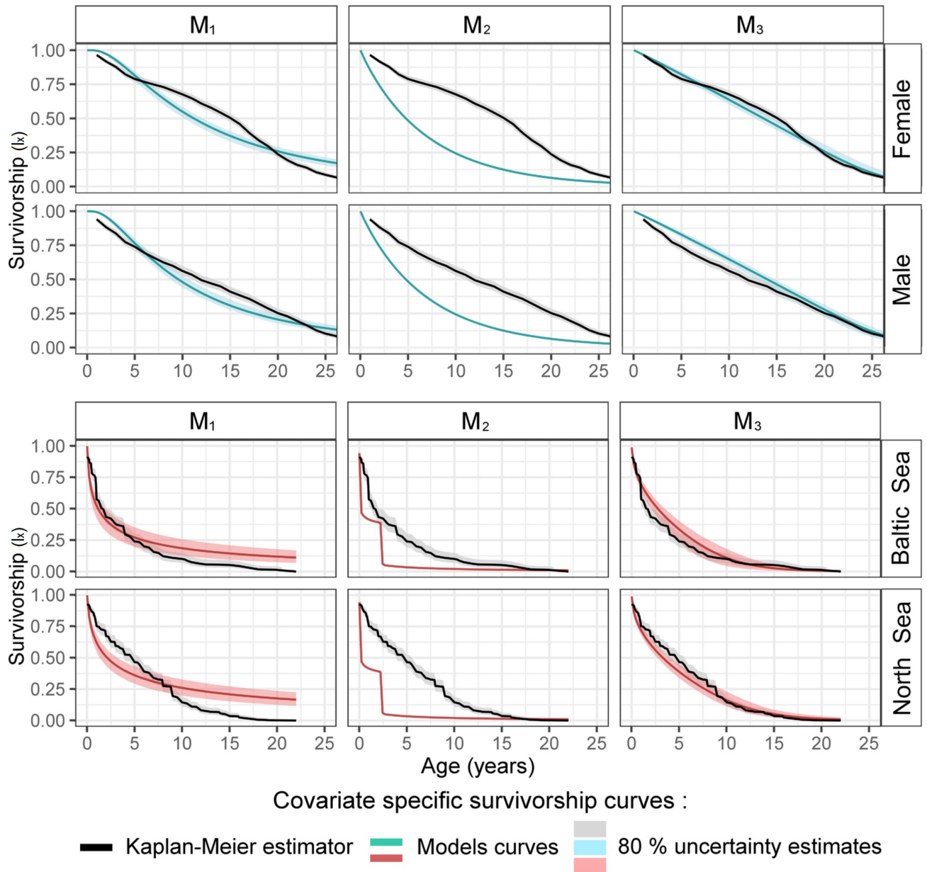
Figure 3.10: Estimated survivorship difference for both case studies.
