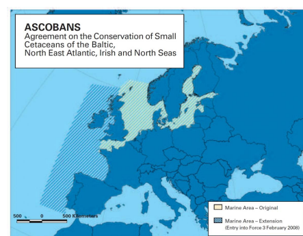
Figure 2.12: ASCOBANS Marine area. Originally, the area was restricted to English Channel, North Sea and Baltic Sea. From the 3 February of 2008, the area now takes into account Bay of Biscay, Celtic seas and offshore Portuguese waters. Figure from https://www.ascobans.org/en/legalinstrument/ascobans .
