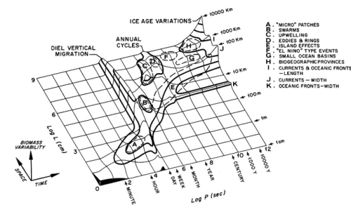
Figure 7.6: Marine biology Stommel Diagram. Emphasizes factors in marine biology, with an emphasis on biological productivity, here labeled "biomass variability". Figure from Haury, McGowan, and Wiebe (1978)
