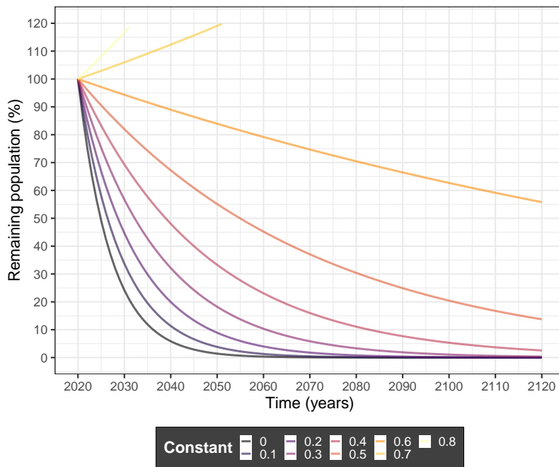
Figure 6.4: Remaining population over 100 years with constant effect on survival. The constant effect was applied to find the value for which the population remains stationary. With a survival intercept to which is added a constant effect equal to 0.65, the population remains stationary over time. This effect is then used in the estimation of the survival model to obtain the age-specific survival rates of a stationary population which will be used to inform the Pella-Tomlinson population dynamics model.
