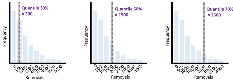
Figure 6.6: Diagram of tuning. The frequency of removals thresholds is depicted as a posterior distribution. The choice of quantile affects the definition of the management objective. Given the posterior distribution of RLA_t , a quantile value of 30% involves a tolerable bycatch threshold of 500 individuals per year. A quantile value of 70% involves a tolerable bycatch threshold of 2500 individuals per year. The choice of the quantile value therefore defines the management objective. This choice is made in order to achieve the CO.
