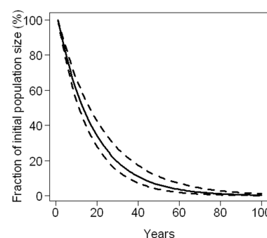
Figure 2.9: Projected population trend. From the vital rates obtained in their study, Mannocci et al. (2012) projected the evolution of the population from the growth rate estimated by Leslie's matrix model. It appears that the population will become extinct within the next 100 years. Figure from Mannocci et al. (2012).
