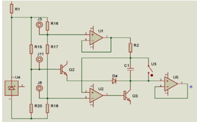
Figure 2.10: Schematic Diagram of the Voltage Ramp Generator board
