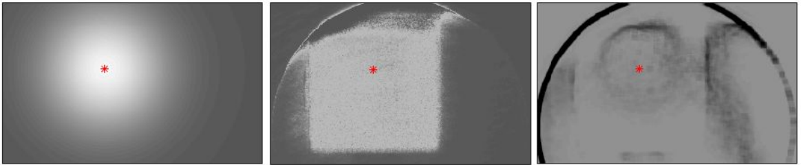
Figure 3.33: Example kernel for a pixel in the center of the flat target (red cross): (a) Euclidean distance; (b) Similarity on 2D frame; (c) local standard deviation in 3D frame
