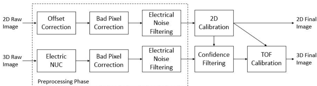
Figure 5.1: Image Processing Workflow
