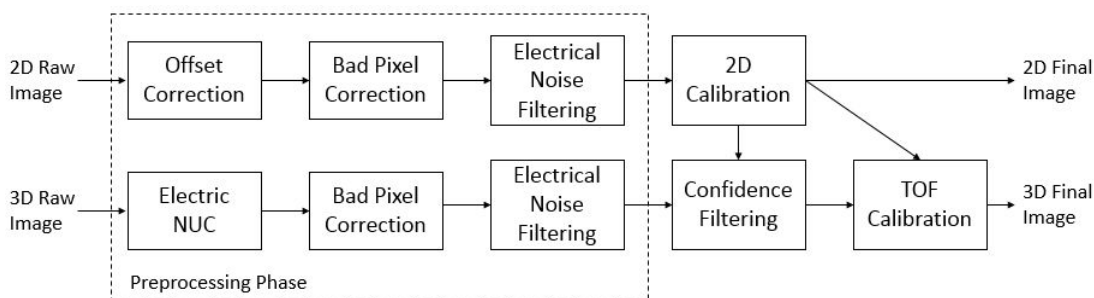
Figure 3.36: Image Processing Workflow
