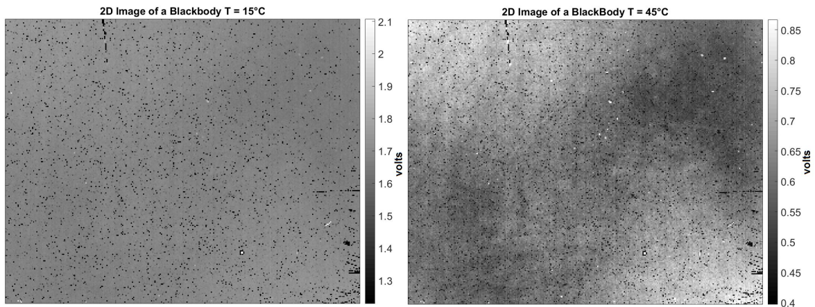
Figure 3.5: 2D images of a blackbody at 15^{\circ}C and 45^{\circ}C demonstrating an increasing nonuniformity with the incoming flux of photons
