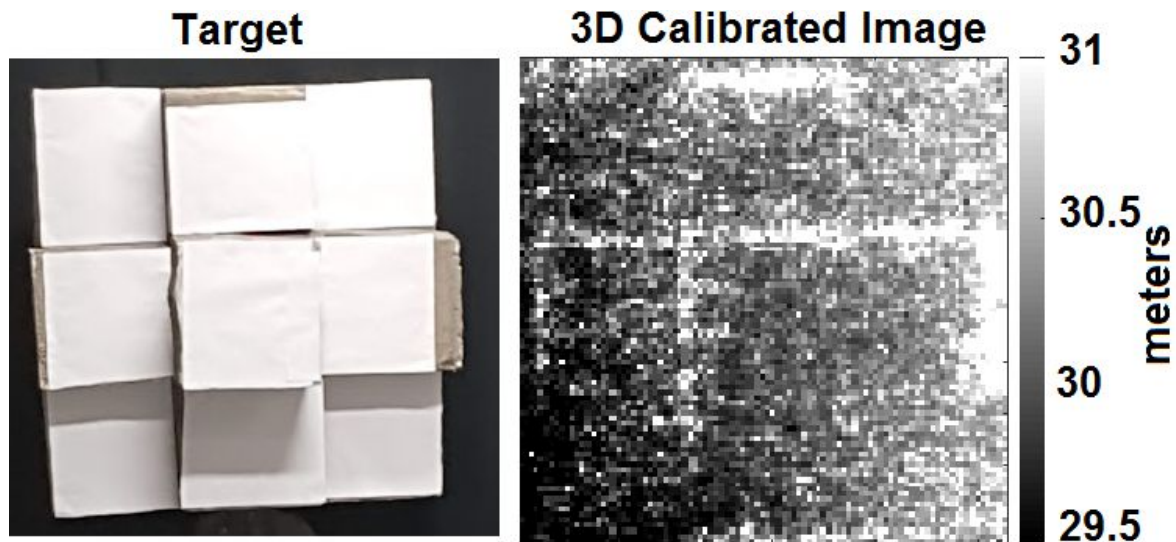
Figure 4.26: The target (left) and the final cropped 3D image after TOF Calibration
