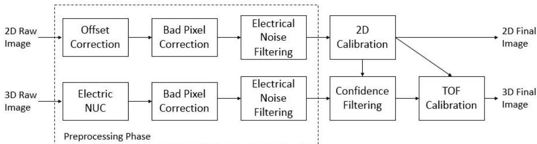
Figure 4.6: Image Processing Workflow
