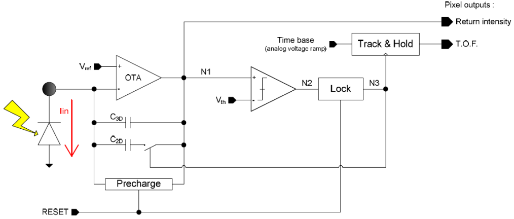
Figure 2.3: Simplified schematic of the pixel.
