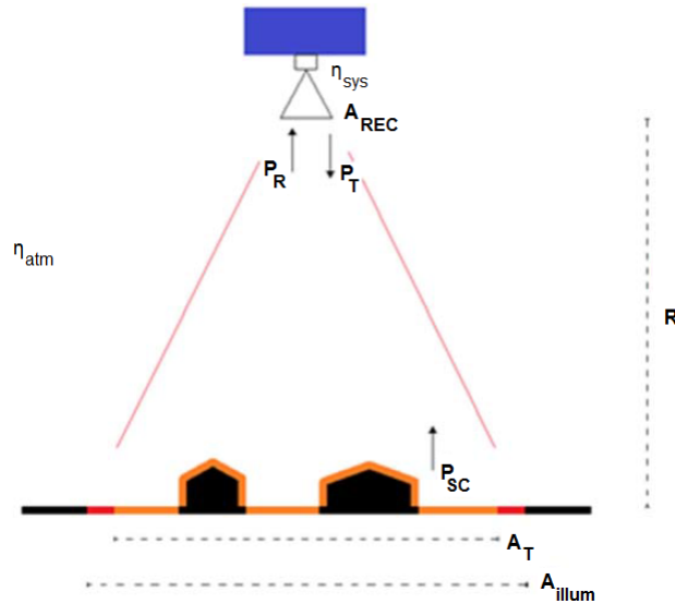
Figure 2.4: Calculating the received power: parameters.
