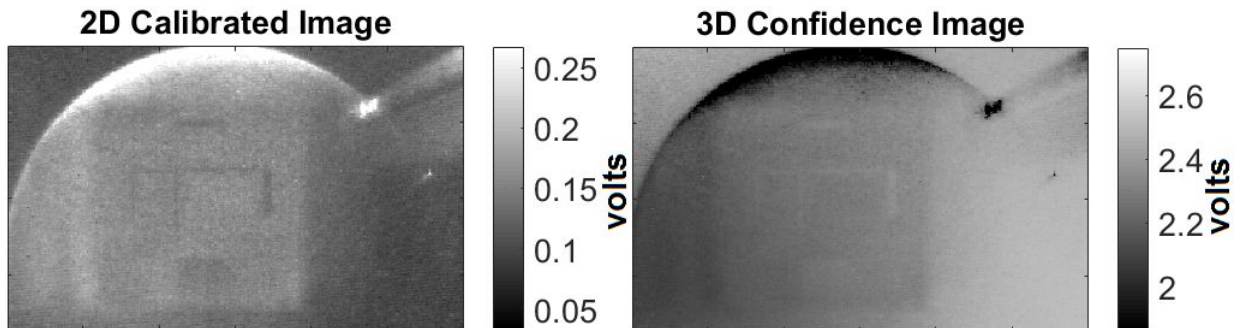
Figure 4.25: Example of 2D and 3D frames after Intensity Calibration and Confidence Filtering.
