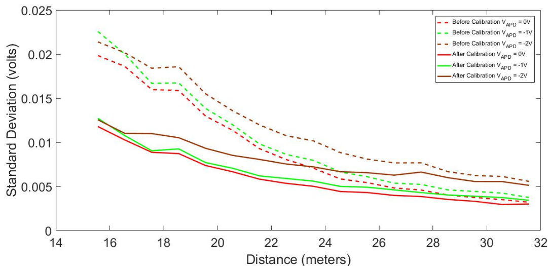
Figure 4.14: Standard deviation of the target before (dashed lines) and after 2D Calibration (full lines)
