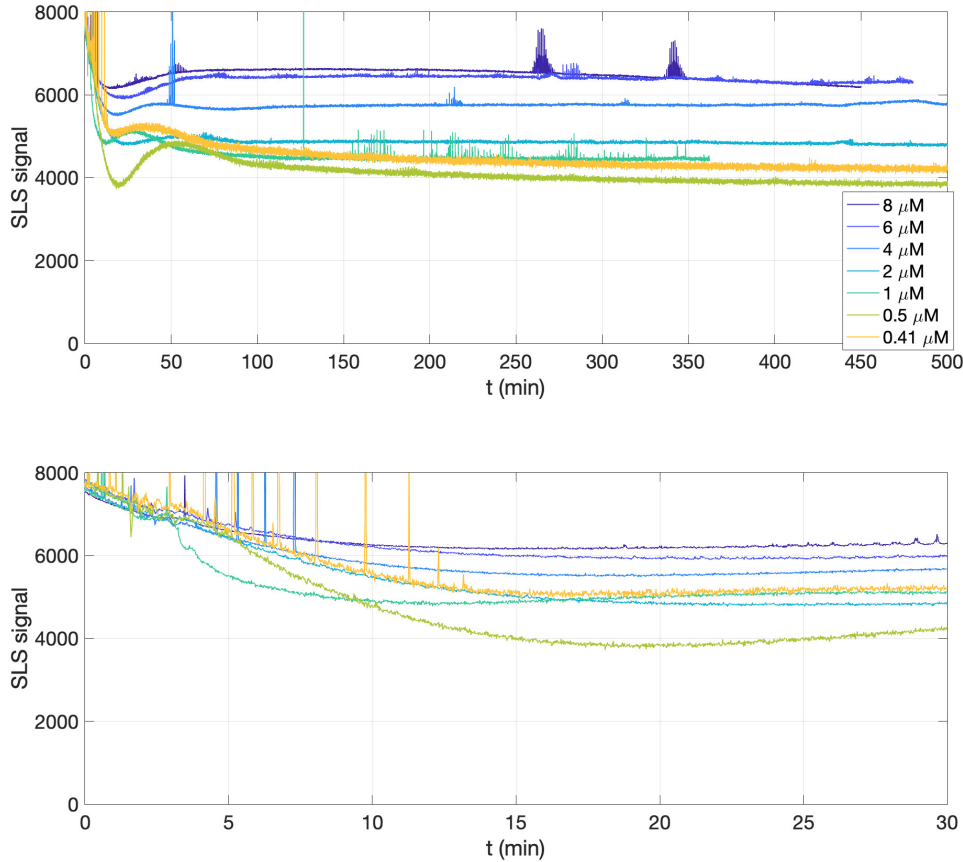
Figure 4.6 – SLS monitoring of the depolymerization of H190A P1 . The depolymerization of isolated P1 subpopulation from H190A oligomers at 70^{\circ}\text{C} was monitored by SLS, at different monomer-equivalent concentrations, in function of time. (Top) Full time range of experiment. (Bottom) First 30 minutes. (H. Rezaei, unpublished).
