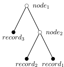
Figure 12.2: binary tree
