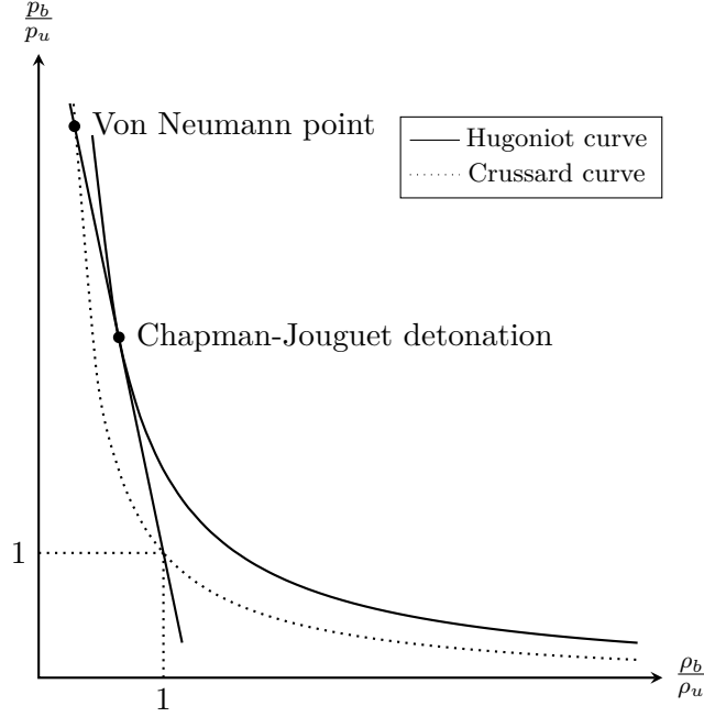
Figure 2.4: Particular point in the ZND theory
