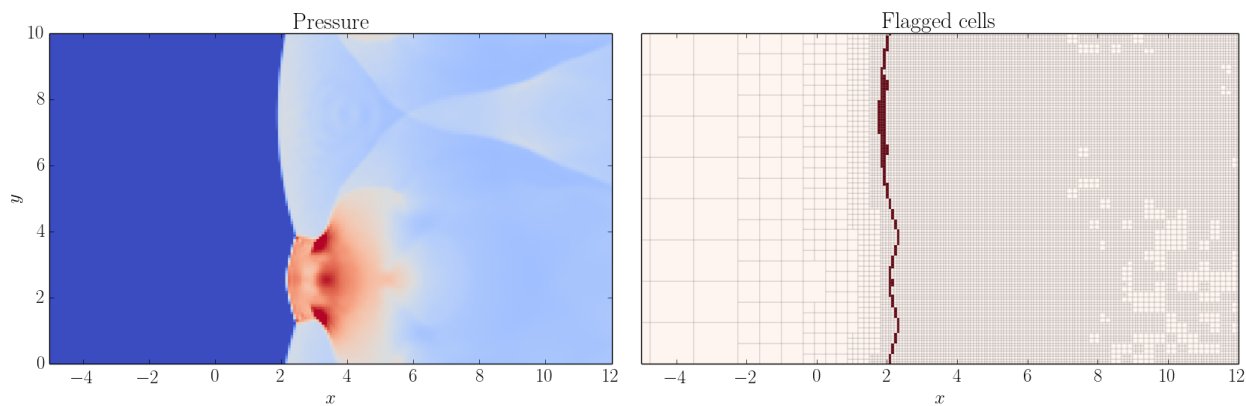
Figure 9.4: Computation of the detonation front (with OSMP7 solver and cure carbuncle method); Pressure field (left) and cells flagged by the carbuncle sensor (right).
