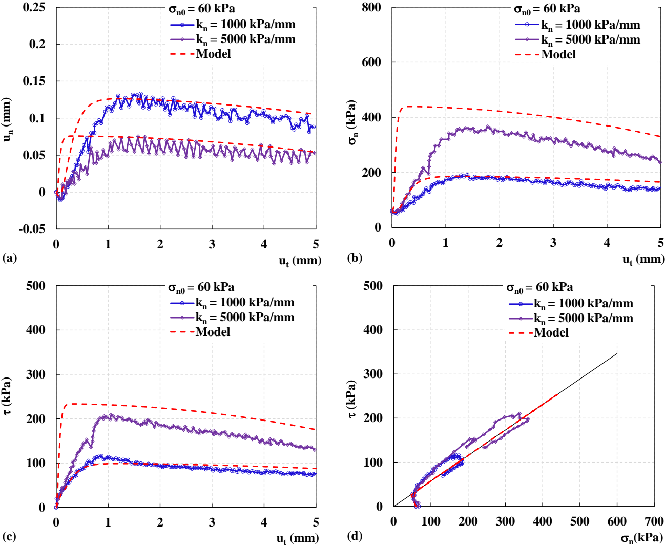
Figure A.1 : Comparison between experimental results and model predictions, \sigma_{n0}=60 \text{ kPa} , k_n=1000 and 5000 \text{ kPa/mm} with rough plate and dense sand
