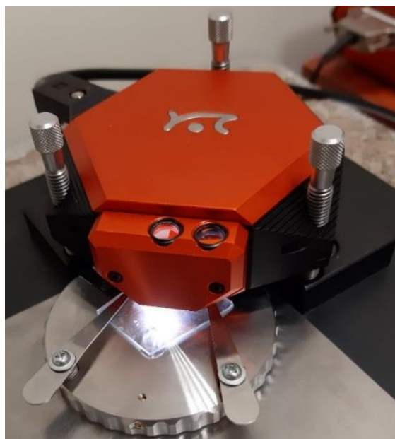
Figure 4.16: Photograph presenting Nanosurf Easyscan 2 Atomic Force Microscopy.
