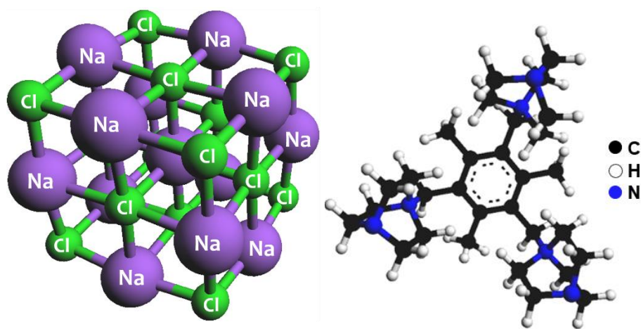
Figure 2.1: NaCl as an examples of material with ion-ion interactions (a) and chemical structure of tris(diazabicyclooctane) used as a host to build supramolecular systems (b).
