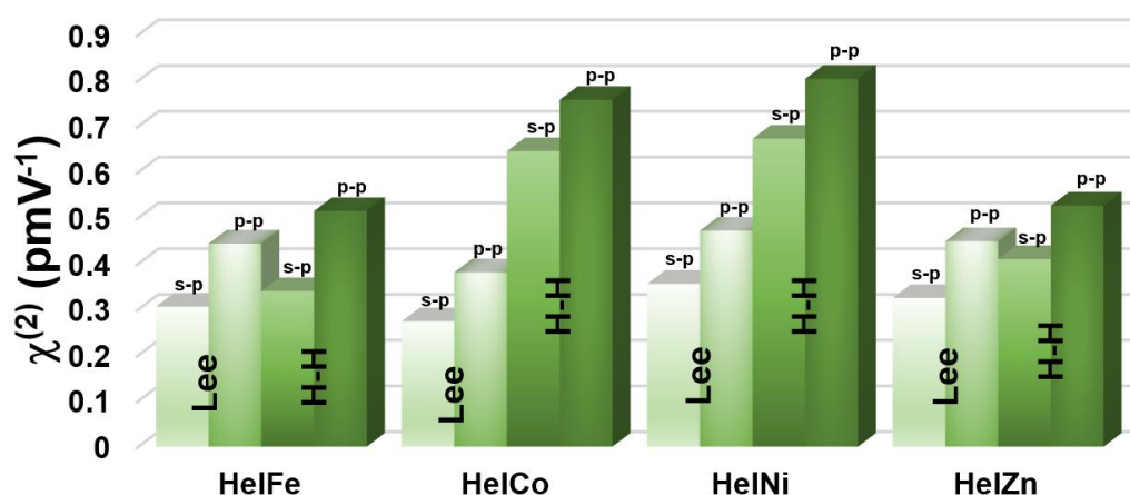
Figure 6.13: Histogram representing values of second-order nonlinear susceptibilities calculated via theoretical models.
