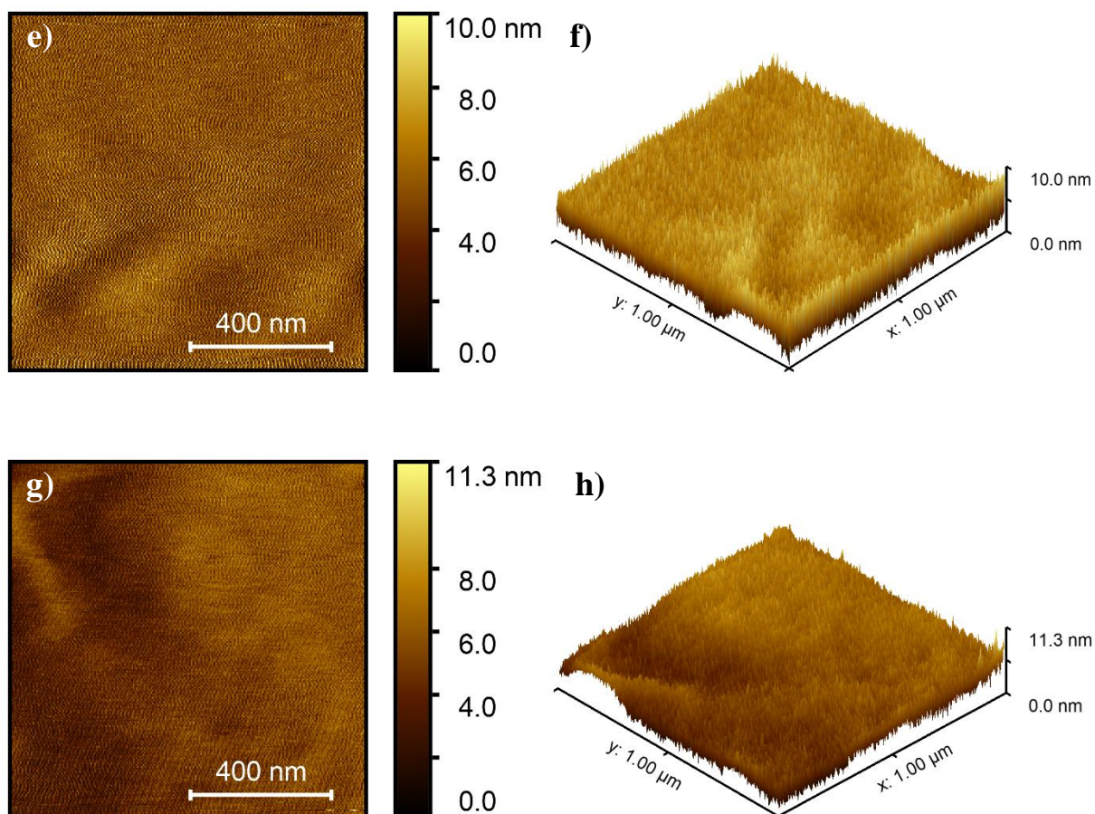
Figure 5.2: Atomic force microscopy (AFM) images of studied metalloporphyrin thin films:
