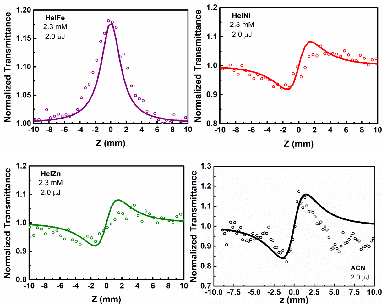
Figure 6.17: CA Z-scan and OA Z-scan characteristics of ACN and triple stranded helicate
