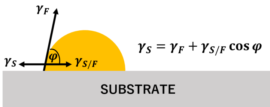
Figure 3.7: Schematic of forming island film on the substrate.
