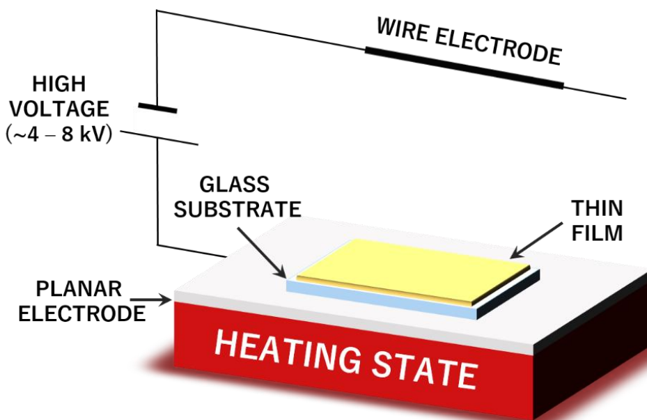
Figure 4.7: Corona Poling setup.
