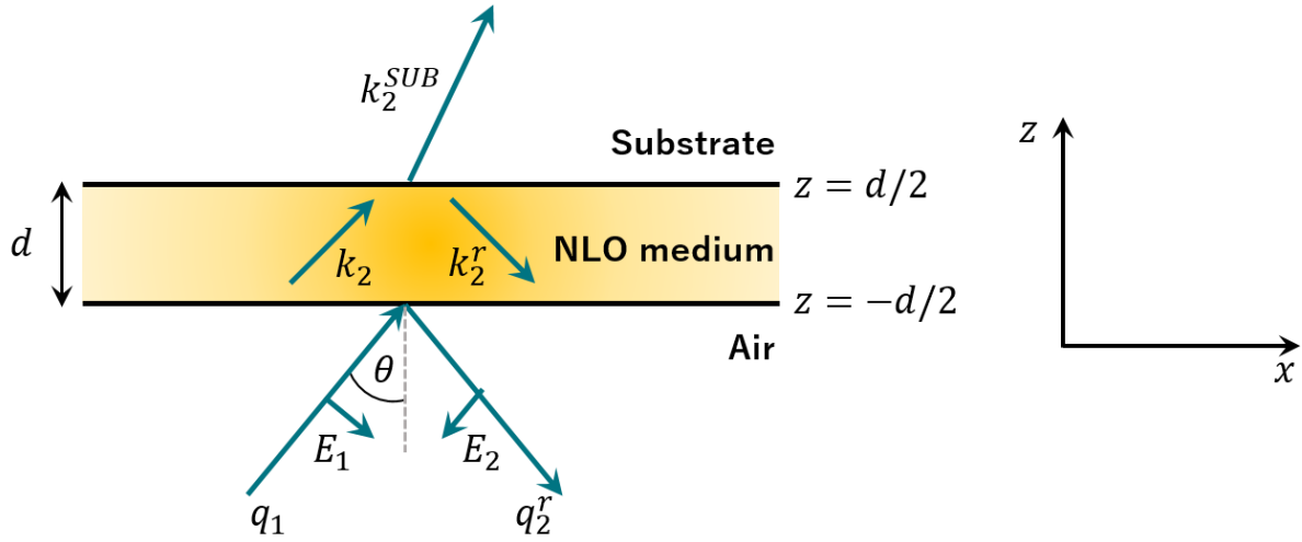
Figure 4.1: Three-layer scheme of the second harmonic generation system with a nonlinear medium.
