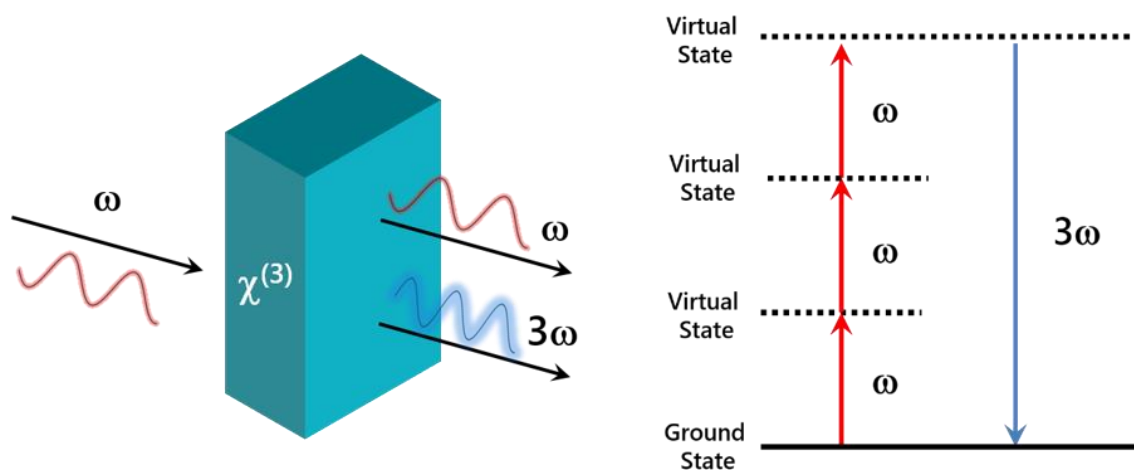
Figure 1.4: Interaction geometry during the third harmonic generation process and energy level diagram described THG process.
