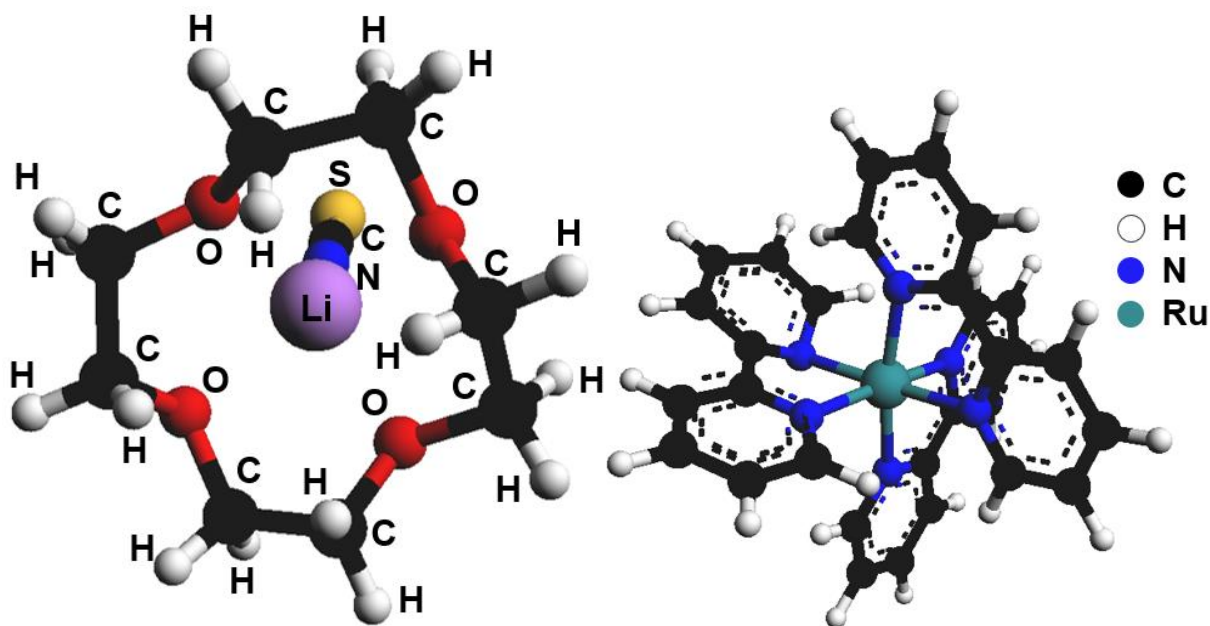
Figure 2.2: Schematic structures of 12-crown-4-Lithium complex (LiSCN) and [\text{Ru}(\text{BPy})_3]^{2+} .
