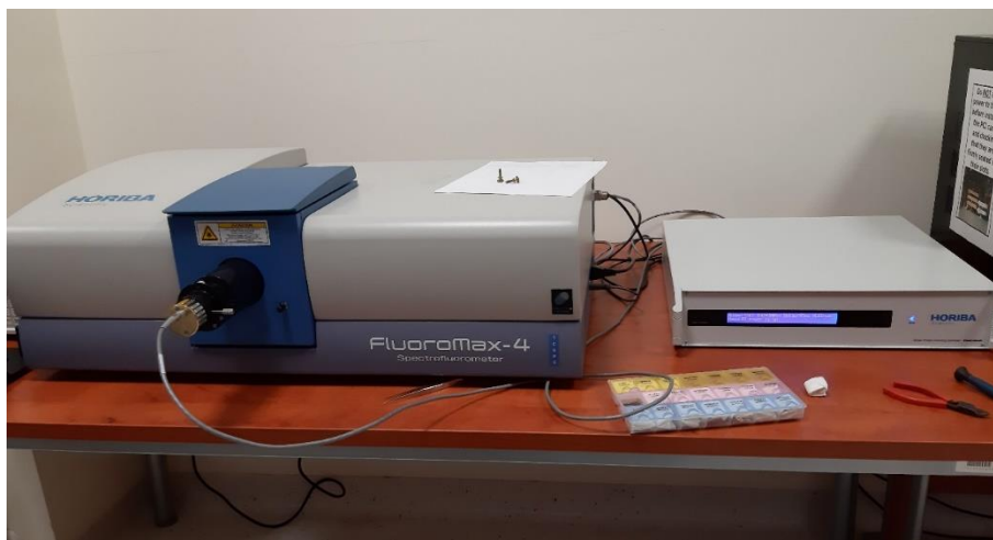
Figure 4.13: Photograph presents spectrofluorometer Horiba FluoroMax-4.
