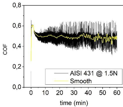
Figure 3.33 Temporal evolution of the COF for the system AISI 431 steel -Al 2 O 3 at 1.5N when in contact with the citric acid 10 -4 M solution.
