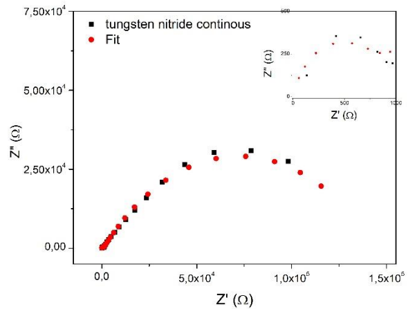
Figure 5.38 Nyquist diagram for of AISI431 steel coated with tungsten nitride in contact with the citric acid 10^{-4} M solution while in continuous sliding at 1.5 N.
