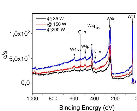
Figure 4.11 XPS survey spectrum for thin films deposited at 1 Pa of gas pressure and different plasma powers.
