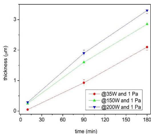
Figure 4.4 Tungsten nitride growth rate at 1 Pa of pressure and different deposition powers
