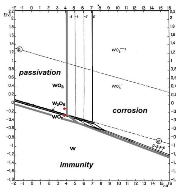
Figure 5.14 E-pH diagram for tungsten [Pourbaix 1974].
