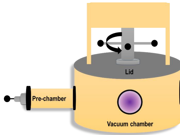
Figure 2.1 Diagram of the vacuum chamber of the Plasyss MP 300S
