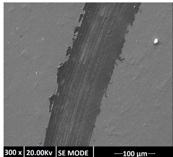
Figure 3.21 -Left- SEM micrography of the AISI 431 steel surface non exposed to wear. -Right- SEM micrography of AISI 431 steel after a pin on disc test at 1.5 N
