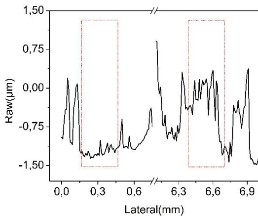
Figure 3.31 Profile of the wear track region after AISI D2 steel after a pin on disc at 0.5 N test in contact with citric acid 10^{-4} M.
