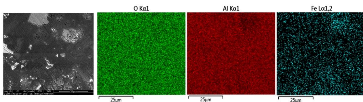
Figure 3.23 Mapping EDS images for a selected region in the counted body after a dry pin on disc test at 0.5 N
