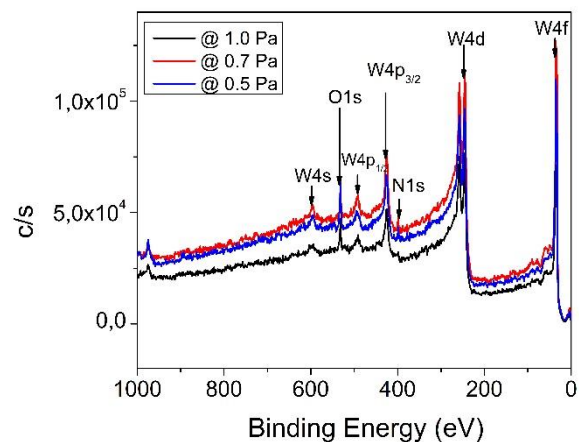
Figure 4.12 XPS survey spectrum XPS survey spectrum for thin films deposited at 150 W of plasma power and different gas pressures.
