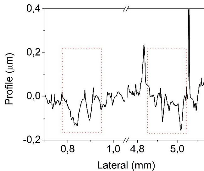
Figure 5.7 Profile of the wear track region for AISI 431 coated with tungsten nitride after a pion on disc test at 1.5 N, and room temperature and relative humidity.
