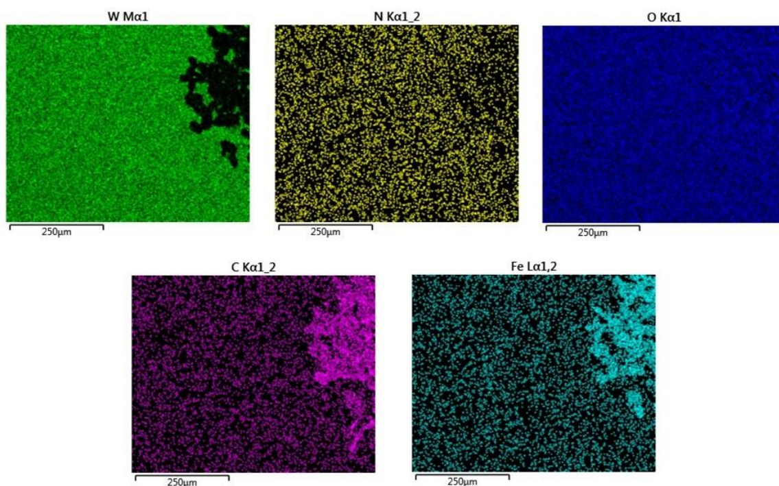
Figure 5.32 Mapping EDS for AISI D2 coated with a silicon buffer layer and tungsten nitride after contact with 10^{-4} citric acid aqueous solution.
