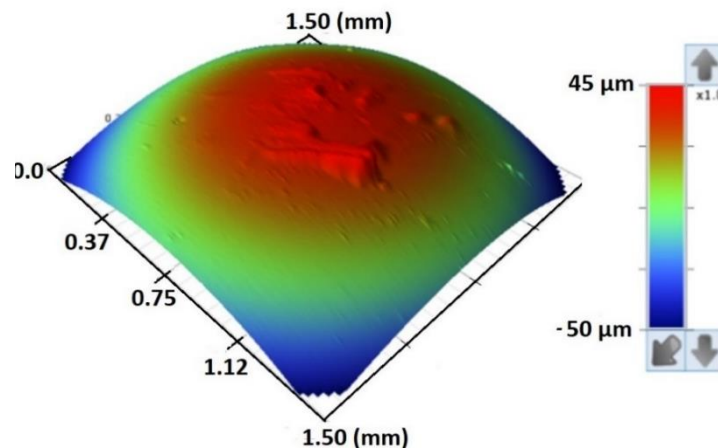
Figure 3.18 \text{Al}_2\text{O}_3 ball 3D image of profilometry after 60 min of pin on disc test at 0.5 N; in contact with AISI D2 steel.
