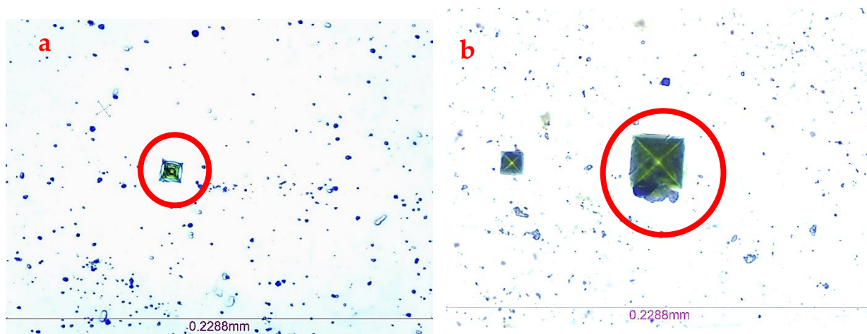
Figure 4.14 (a) Indentation trace for a 0.5 N applied load over AISI D2 coated with tungsten nitride at 200 W and 1.0 Pa. (b) Indentation trace for a 0.5 N applied load over AISI D2 coated with tungsten nitride at 200 W and 0.7 Pa.
